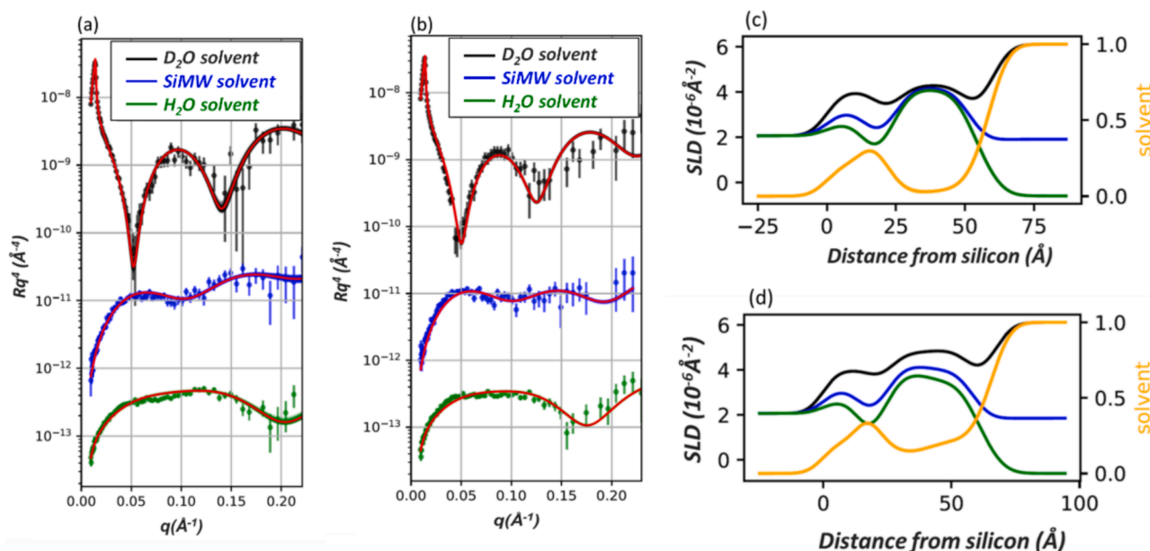
Fig. 1. Best fittings for the NR spectra of the main dRaft SLB at 37 °C and 17 °C. Best fit (lines) for the NR spectra (dots) of the dRaft SLB at 37 °C (a) and 17 °C (b) in the 3 water solvents (D 2 O in black, SiMW in blue and H 2 O in green). The H 2 O and SiMW reflectivity curves are shifted down on the vertical axis, with respect to D 2 O reflectivity, each by a factor 10 -3 , for the sake of clarity. Solvent penetration percentage is shown in yellow (right axis) together with the respective SLD profiles (left axis) at 17 °C (c) and 37 °C (d). (For interpretation of the references to color in this figure legend, the reader is referred to the web version of this article.)
