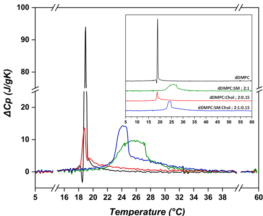
Fig. 3. DSC thermograms of lamellar systems of the dRaft model membrane and its separate components. d 54 DMPC (black), d 54 DMPC:SM; 2:1 (green), d 54 DMPC:Chol; 2:0.15 (red) and d 54 DMPC:SM:Chol; 2:1:0.15 (blue). Data were collected at a scan rate of 1 °C/3 min, in cooling mode. The insert shows the full spectra shifted on the y-axis for better visualisation. Data are reported as \Delta C_p , that is the excess C_p registered during the phase transitions, with respect to the systems' C_p before and after the phase transition. (For interpretation of the references to color in this figure legend, the reader is referred to the web version of this article.)
