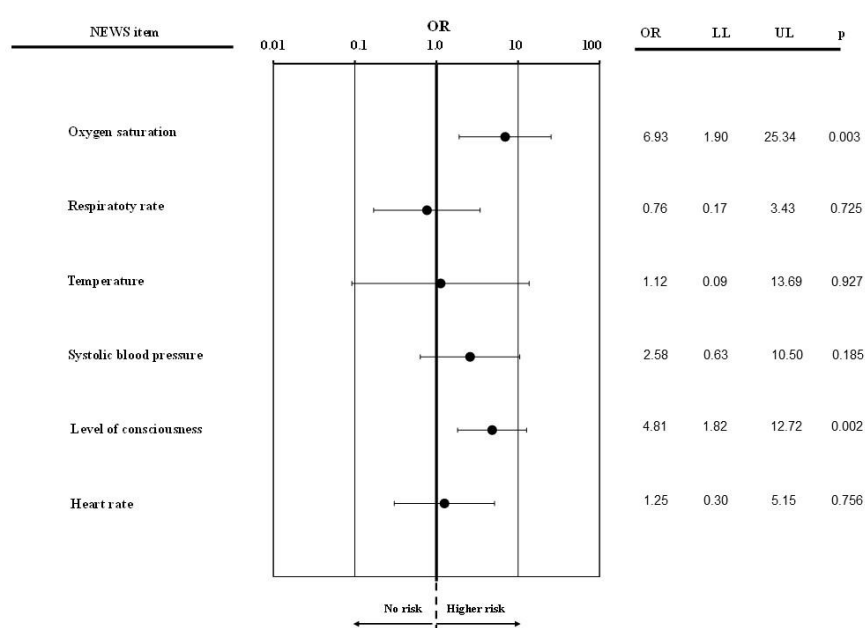
Figure 5. NEWS value with a 3-single parameter and predictors of hospitalization.
