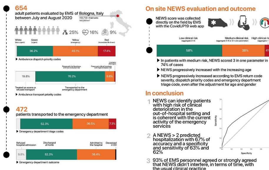
Figure 1. Infographics of the descriptive statistics.
