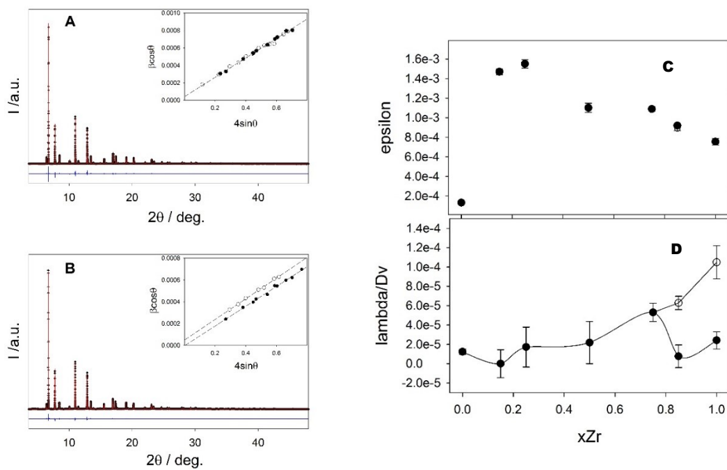
Figure SI1. HR-XRPD patterns of Gd_2(Ti_{1-x}Zr_x)_2O_7 for xZr = 0.75 (A) and 0.85 (B) with corresponding W.H. plots in the insets. The calculated strain ( \epsilon ) values and \lambda/D_v values are shown in panels (C) and (D), respectively. Full and empty circles are the refined values for the fluorite and pyrochlore peaks, respectively.
