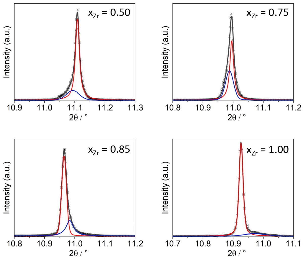
Figure SI2. Close-up view of (440) p reflection in selected HR-XRPD patterns of Gd 2 (Ti 1-x Zr x ) 2 O 7 solid solution. Cross symbols represent the observed pattern; the dark grey solid line is the total calculated profile by Rietveld refinement, while solid red and blue lines are the calculated profile for Phase 1 and Phase 2 respectively.
