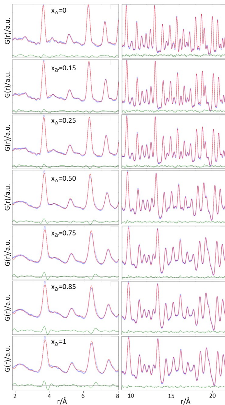
Figure SI5. Experimental G(r) functions in the 1.8-8 Å (left side) and 9-22 Å (right side) intervals are displayed as light blue circles. Labels in the panels refer to the sample composition according to Gd_2(Ti_{1-x}Zr_x)_2O_7 formula. The fits using the pyrochlore model are reported as red curves. The green curves represent the differences between experimental data and the model-
