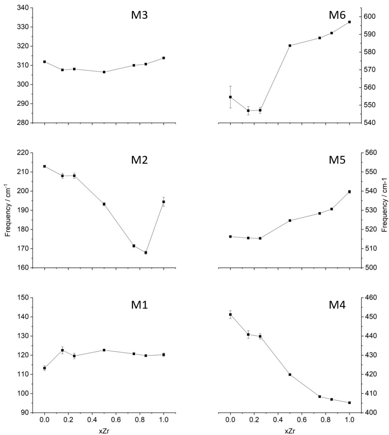
Figure SI4 Frequency shift of Raman modes in Gd_2(Ti_{1-x}Zr_x)_2O_7 as obtained by fitting the spectra with Gaussian functions.
