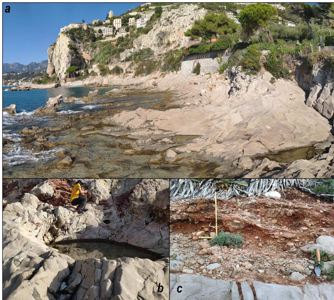
Figure 4. General view of the main coastal features in the study area (a), dominated by the ramp (a). Major rockpool of the pothole type (b), and relic spot of raised marine deposit, and (c) in the area of Punta Garavano.
