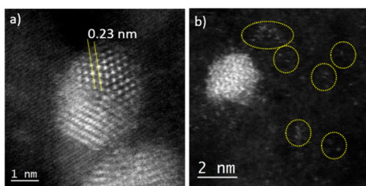
Figure 2. High-resolution STEM-HAADF images of 1 wt % Pd/NiO catalyst showing a crystalline particle (a) and sub-nanometer species of Pd distributed across the support (b).
