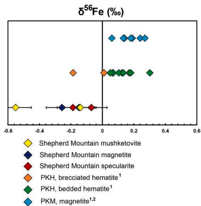
Fig. 7. The stable Fe isotope compositions of mushketovite, magnetite, and specularite from the Shepherd Mountain deposit. The \delta^{56}\text{Fe} values of magnetite and hematite from the PKM and PKH deposits, respectively, are included for comparison. The reported values are an average of two measurements. Error bars indicate the conservative errors of the variations of the standard. Data source: 1 = Tunnell et al. (2021), 2 = Childress et al. (2016).
