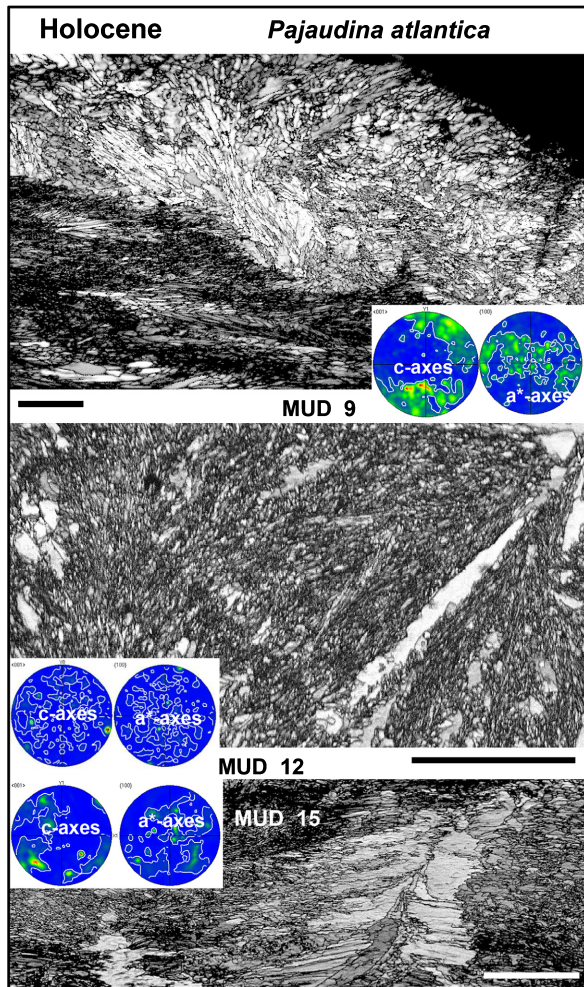
Fig. 10. EBSD band contrast image and associated pole figure depicting the microstructure and texture of the Recent thecideide brachiopod Pajaudina atlantica (LMU-PA008, LMU-PA0010 and LMU-PA09 from top to bottom, respectively) The shell of this brachiopod species includes all types of biocrystals: nanogranules, granules, acicles, small polygonal crystals and large polygonal crystals. The degree of calcite co-orientation is low. Scale bars represent 20 \mu\text{m} for A and 50 \mu\text{m} for B and C. [Colour figure can be viewed at wileyonlinelibrary.com ]
