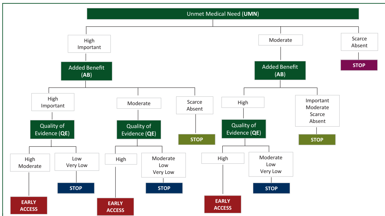
Figure 1. General scheme of the skip pattern approach. Colored cells indicates the priority status and the exclusion level according to the general scheme of the skip pattern approach.
