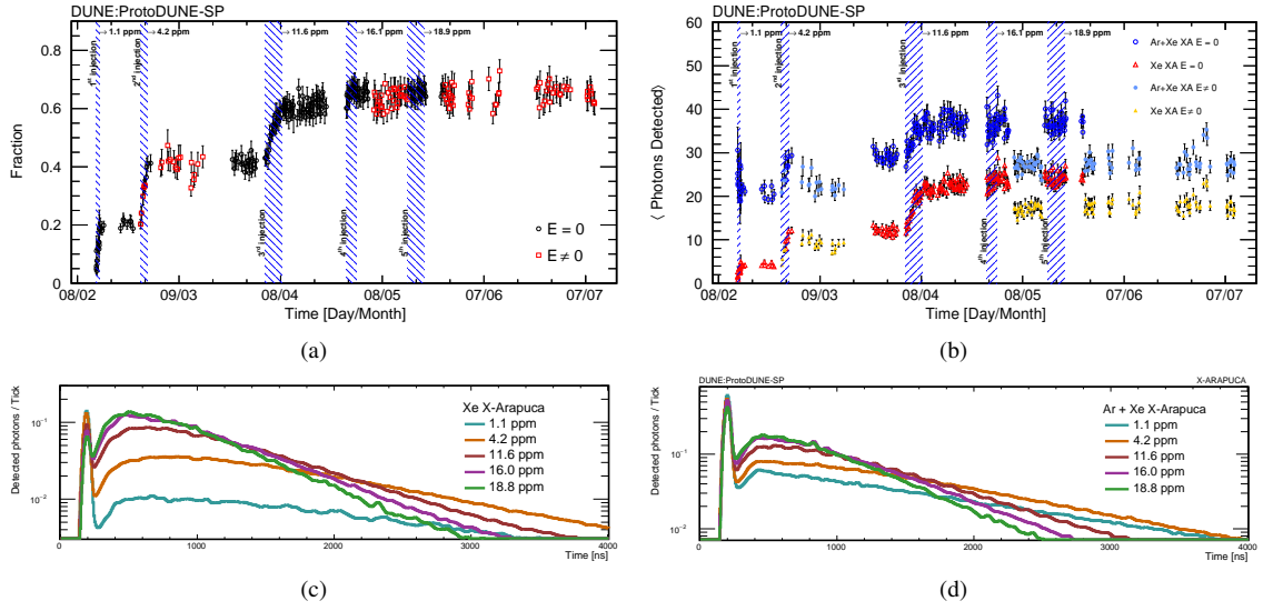
Figure 4: (a): Fraction of wavelength-shifted light ( 128 \text{ nm} \rightarrow 178 \text{ nm} ). (b) Average light detected by the dedicated X-ARAPUCA modules. Shaded areas show xenon injection periods. (c)(d) Average waveforms as a function of the xenon concentration for the “Xe XA” and the “Ar+Xe XA” respectively.
