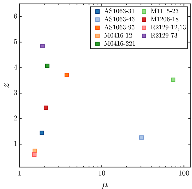
Fig. 5. Redshift and magnification of the sources in Table 3 identified by visual inspection after removing the two sources marked with the asterisk. The 1\sigma error on magnification is about 10% up to \mu = 10 , and it can reach a factor of 2 or higher for \mu > 20 .
