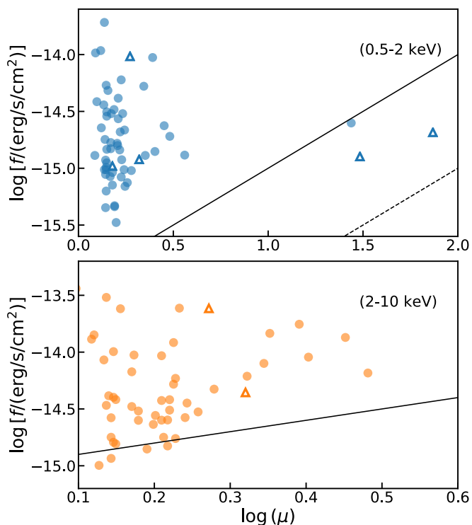
Fig. 10. Scatter plot of the soft (top panel) and hard (bottom panel) observed flux vs. the weighted magnification. In the top panel the region below the solid and dashed black lines corresponds to lensed fluxes below 10^{-16} and 10^{-17} erg/s/cm 2 , respectively. In the bottom panel, the region below the black line corresponds to lensed fluxes below 10^{-15} erg/s/cm 2 . Sources marked with circles are X-ray selected, and triangles correspond to sources identified as X-ray counterparts of optically lensed sources (listed in Table 3). Only sources with S/N \geq 2 in each band are shown.
