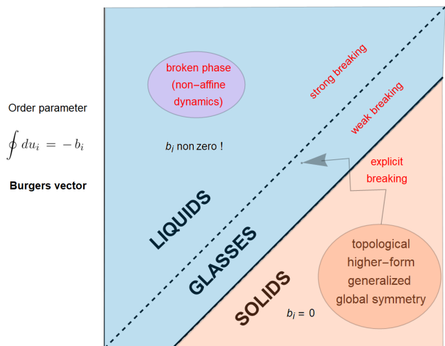
Figure 13. The phase diagram in terms of the topological higher-form generalized global symmetry, which corresponds to the conservation of the two-form \partial_\mu J_I^{\mu\nu} = 0 , and of the topological order parameter – the Burgers vector b_i . The filled line indicates the explicit breaking of such a symmetry due to the appearance of non-affine displacements. It also distinguishes the phases with zero Burgers vector b_i = 0 (solids) from the ones (glasses, fluids) with a finite value for this topological order parameter. The dashed line between liquids and glasses cannot be defined by any fundamental symmetry, but only by the strength of the symmetry breaking, weak for glasses (corresponding to a very long relaxation time) and strong for liquids. In this view, the difference between solids and amorphous systems (liquids and glasses) is purely topological and not linked to any spacetime symmetry.
