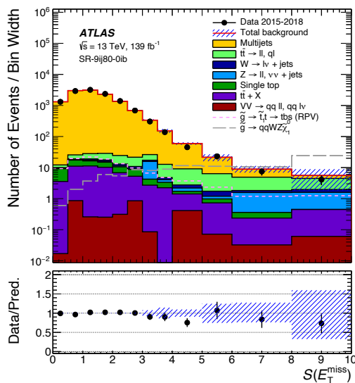
(c) SR-9ij80
