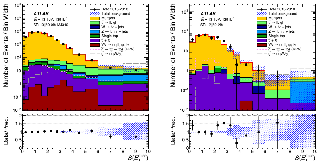
(a) SR-10ij50-0ib-MJ340
