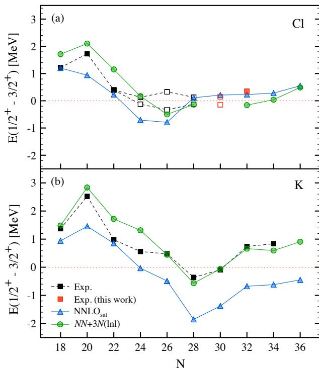
FIG. 9. Variation of the energy difference between the first 1/2^+ and 3/2^+ states for Cl and K isotopes with the neutron number N . GGF calculations were performed with NNLO sat and NN+3N(\text{lnl}) interactions. Full squares are experimental values. When only the absolute value of the energy difference \Delta has been established, empty squares are added following a 1/2_1^+ or 3/2_1^+ hypothesis for the ground state. No value is given for the calculation of ^{47}\text{Cl} with the NN+3N(\text{lnl}) interaction, as explained in text. Experimental values for ^{41,43,45}\text{Cl} are taken from [3, 19–24]; experimental values for K isotopes are taken from [13–15].
