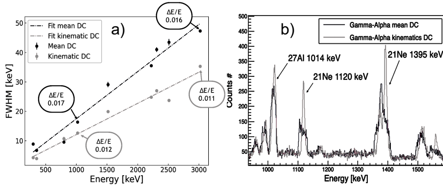
Fig. 2. – a) Energy resolution (FWHM) plotted against the energy in a range between 0 and 3 MeV of the \gamma peaks after Doppler correction with \beta -factor calculated from the \gamma event or with the information from GALTRACE. b) Two \gamma spectra obtained with the aforementioned methods.
