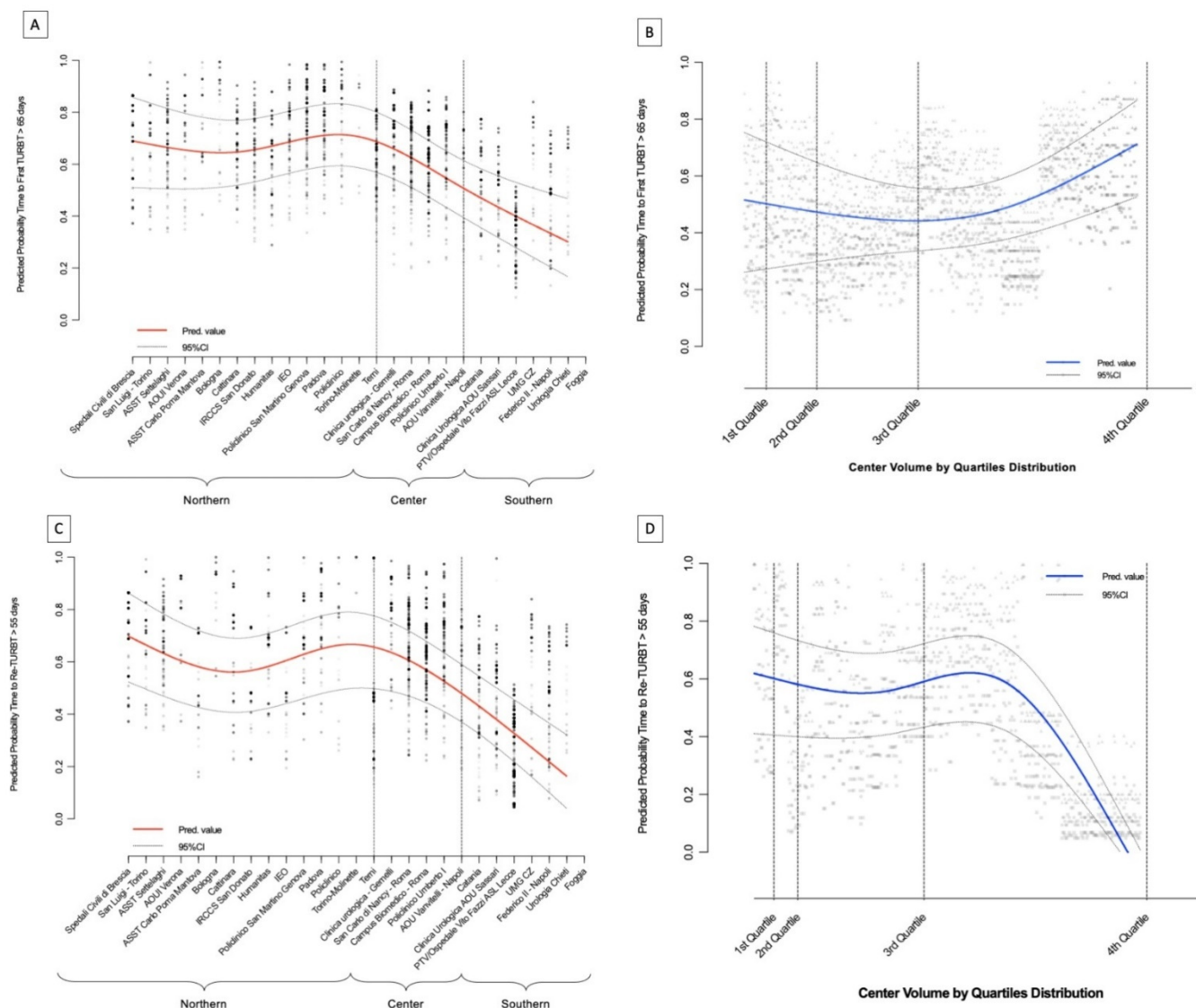
Figure 2. LOWES functions. (A) Predicted probability time to first TURBT > 65 days among institutions; (B) Predicted probability time to first TURBT > 65 days among center volume percentiles; (C) Predicted probability time to Re-TURBT > 55 days among institutions; (D) Predicted probability time to Re-TURBT > 55 days among center volume percentiles.
