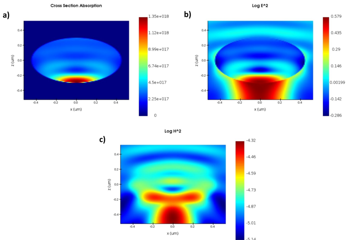
Fig. 3 Cross sections at 658 nm (wavelength) in xz -plane through the middle of the pigment particle with a long axis radius of 450 nm for a optical absorption, b integrated electric field ( E^2 ), and c integrated magnetic field ( H^2 ). The high inten-
