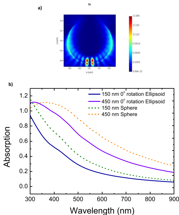
Fig. 5 a Cross section at 300 nm (wavelength) in xz -plane through the middle of the spherical pigment particle with radius of 450 nm of the z -component of integrated the electric field. The constructive interference patterns are clearly visible and are indicative for light circulation within the particle. b Optical absorption spectra of ellipsoidal and spherical pigment particles. Although the optical absorption of the spherical particles appears larger than that of the ellipsoid particles, the total volume ratio between the spherical and ellipsoidal particles is 2.25, resulting in less light absorption per pigment molecule than in the spherical particle
