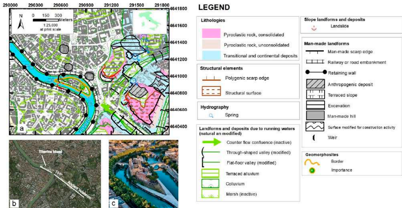
Figure 14. (a) Geomorphological map of the Tiberina Island geosite. It is evidenced on the urban geomorphological map of Rome as it represents an urban geomorphosite of high cultural value inserted in a wider territory rich of geomorphological and cultural features. (b) Scheme showing the ancient confluence between Velabrum Maius and Tevere River. (c) Tiberina Island iconic image.
