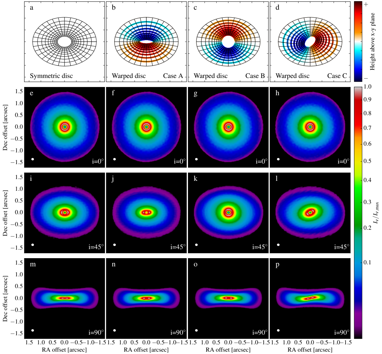
Figure 6. Same as Figure 5, but the colorscale images show synthetic ALMA observations at 340 GHz. The synthesised beam is shown in white in the bottom left corner of each panel. No obvious azimuthal asymmetry is visible in the sub-millimetre continuum images of warped discs. The isophotes of an inclined disc are concentric ellipses, whose position angle and aspect ratio may change as a function of radius. The strength of this effect increases with increasing inclination angle.
