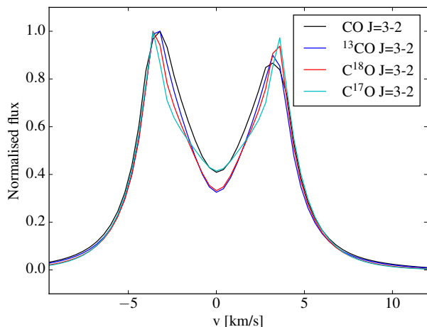
Figure 8. Variation of the line profile as a function of optical depth in our fiducial model as seen in the J=3-2 transition of various CO isotopologues. A linear continuum has been subtracted from the spectral lines, which were then normalised to their peak value. The inclination of the outer disc is i = 45^\circ and the disc is bending perpendicular to the line of sight (Case C). The CO line shows a clear asymmetry in the strength of the Keplerian peaks but the amount of asymmetry in the line profile decreases from CO, through ^{13}\text{CO} and \text{C}^{18}\text{O} to \text{C}^{17}\text{O} . This behaviour is caused by the increasing azimuthal temperature variation in the disc with increasing height above the midplane. The higher the optical depth in the lines, thus the higher they originate above the midplane, the higher the asymmetry of the Keplerian peaks will be.
