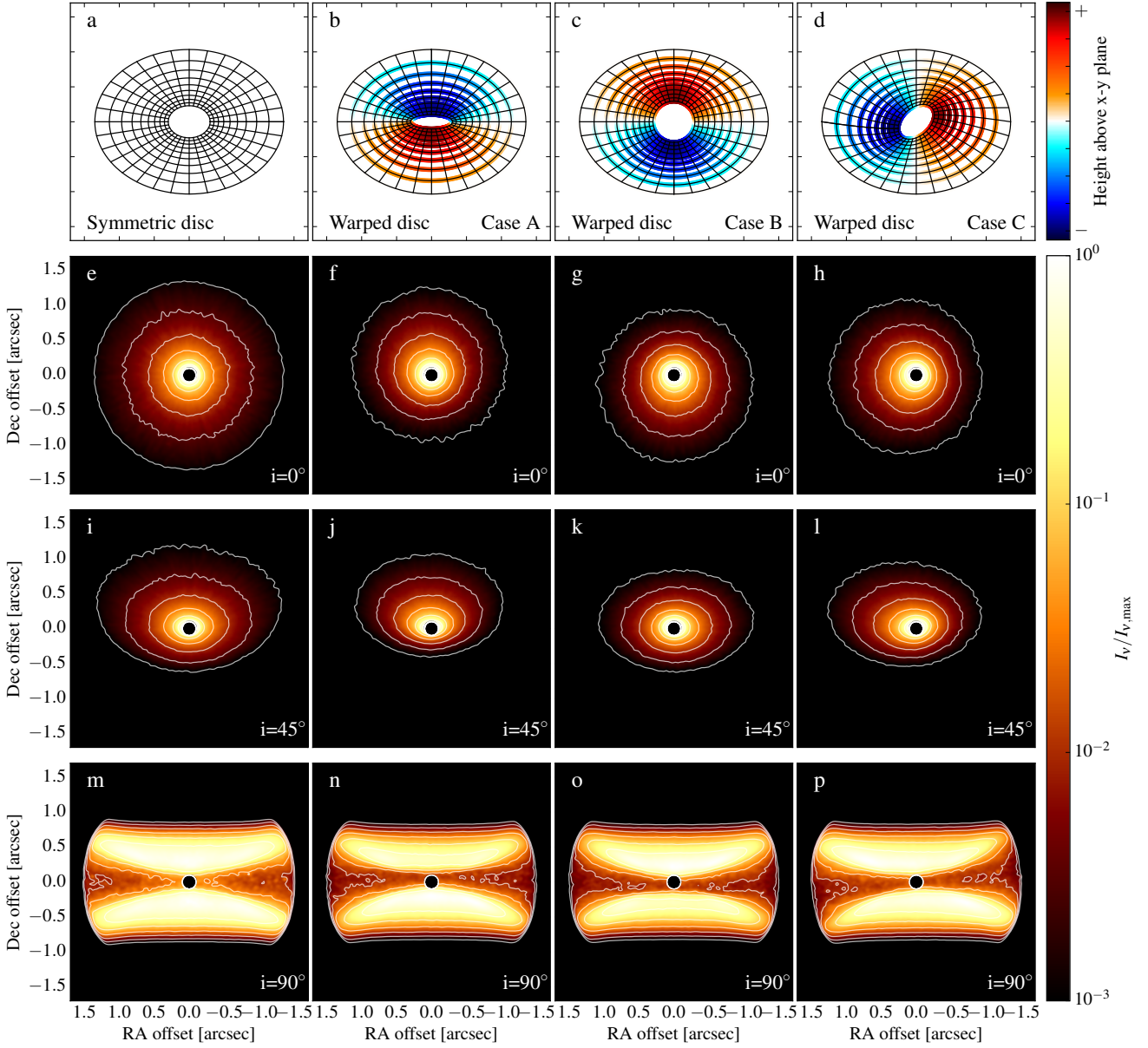
Figure A1. Same as Figure 5, but for the weakest warp in our simulations with \alpha = 0.02 and \beta_0 = 15^\circ . The deviation of the surface brightness distribution of such weakly warped disc from that of that of an unperturbed, symmetric disc is significantly weaker than in our fiducial model at all inclination angles. The presence of a warp might be inferred from the shift of the stellar position from the centre of the disc as seen in scattered light. However, this effect can also be caused by anisotropic scattering if the grains are comparable or larger than the wavelength of observations. Note that the smaller outer radius of the warped discs compared to the unperturbed model, whose surface density is based on our fiducial model (with \alpha = 0.2 and \beta_0 = 30^\circ ) is due to the faster spreading of the disc in the hydrodynamic simulations in the fiducial model.
