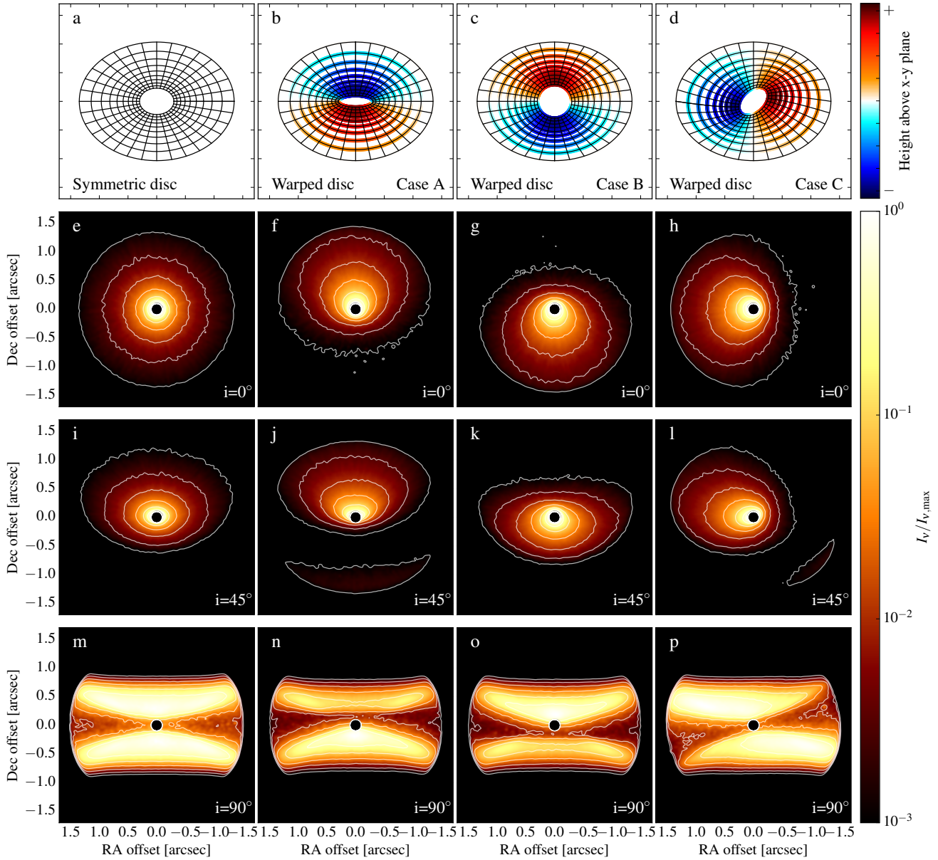
Figure 5. Morphology of warped discs in near-infrared scattered light observations. Panel a shows a cartoon of a symmetric disc while Panel b–d shows a cartoon depicting the structure and orientation of the warp shown in the synthetic images in each column. The colourscale shows the height above the mid-plane of the disc with blue showing structures below the mid-plane while red shows regions above the mid-plane. The second, third and fourth row from the top show the scattered light images at i = 0^\circ , i = 45^\circ and i = 90^\circ inclination angles, respectively. The second, third and fourth column from the left shows the synthetic H-band scattered light images of our fiducial warped disc model, while the leftmost column shows the images predicted images of an unperturbed, symmetric disc. Warped discs show an azimuthally asymmetric surface brightness distribution at all inclination angles, even if seen perfectly face on. The surface brightness asymmetry is due to the shadowing of the outer disc by the inner regions. The position angle of the asymmetry is set by the orientation/position angle of the warp.
