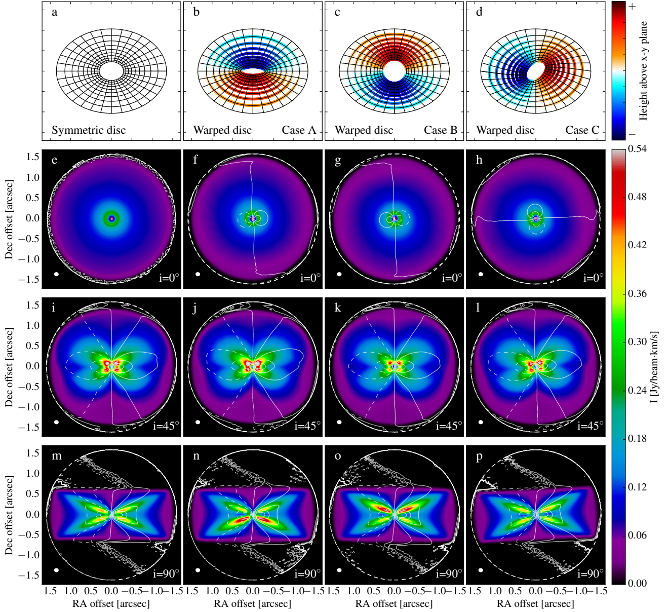
Figure A4. Same as Figure 9, but for the weakest warp in our simulations with \alpha = 0.02 and \beta_0 = 15^\circ . Both the kinematic signatures and the surface brightness asymmetry are significantly weaker than in the fiducial model with \alpha = 0.2 and \beta_0 = 30^\circ . The surface brightness asymmetry is only visible clearly when the disc is seen at a very high inclination angle and the disc is bending along the line of sight (Panel n , o ). The strength of the kinematic signatures decreases with increasing inclination angle.
