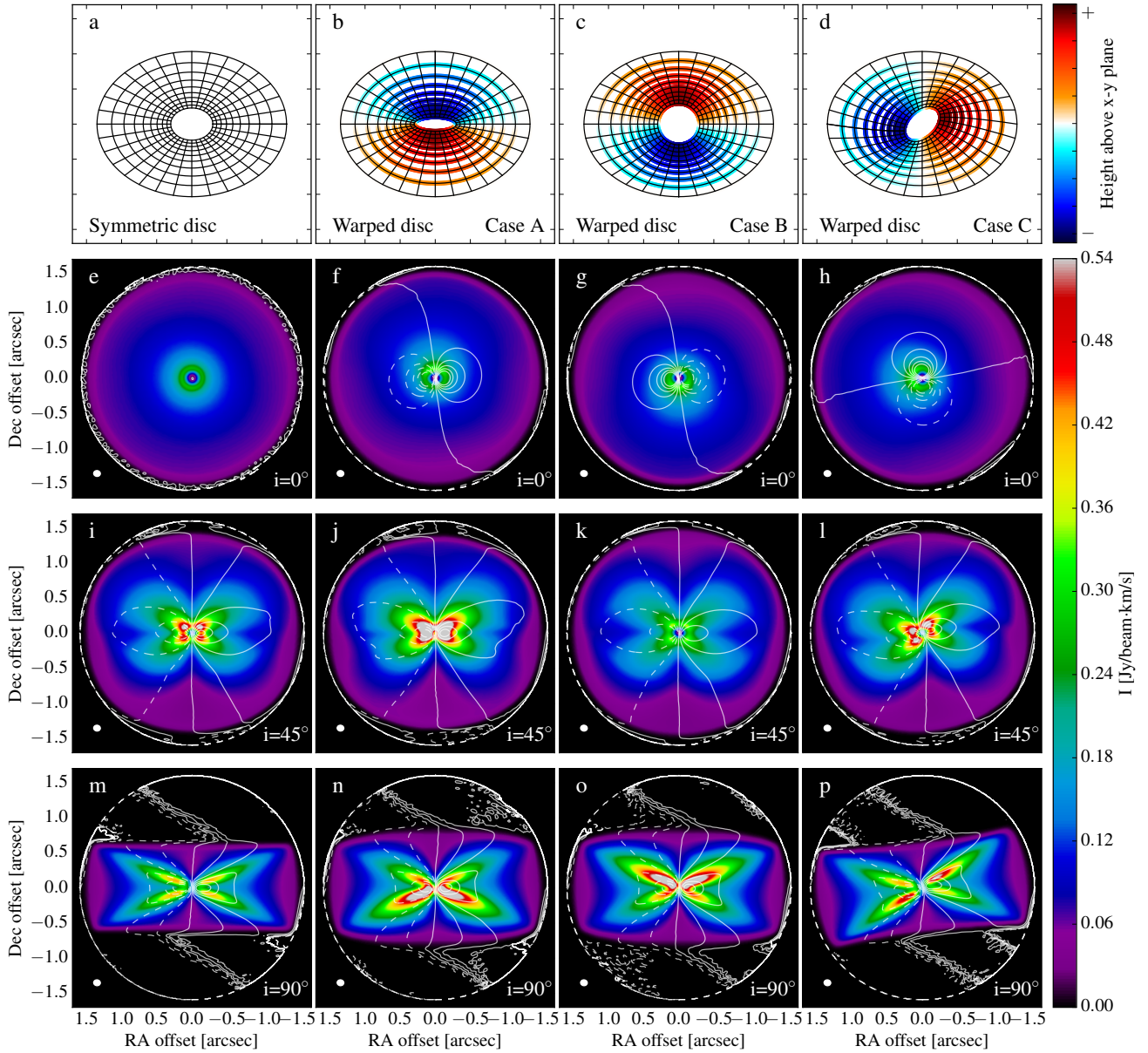
Figure 9. Predicted ALMA observations in the CO J=3-2 line. The colourscale images show the integrated intensity (0th moment map) while the contour lines show the intensity weighted velocity (1st moment) map. Dashed contours denote negative velocity. Panel a–d show the orientation of the warp in the disc in each column. The synthesised beam is shown in white in the bottom left corner of each panel. The surface brightness distribution of warped discs shows asymmetries at all inclination angles. For face-on discs (Panel f–h ) the projected velocity increases towards the inner edge of the disc independently of the orientation of the warp. At intermediate inclinations (Panel j–l ) the projected velocity of a warped disc increases or decreases inwards depending on the orientation of the warp. In case the disc does not bend along the line of sight the velocity field shows a characteristic twist around the centre of the disc (see Panel l ). The strength of the kinematical signatures of warp decreases with increasing inclination angle. For edge-on discs the velocity field is practically indistinguishable from that of an unperturbed disc (Panel n–p ).
