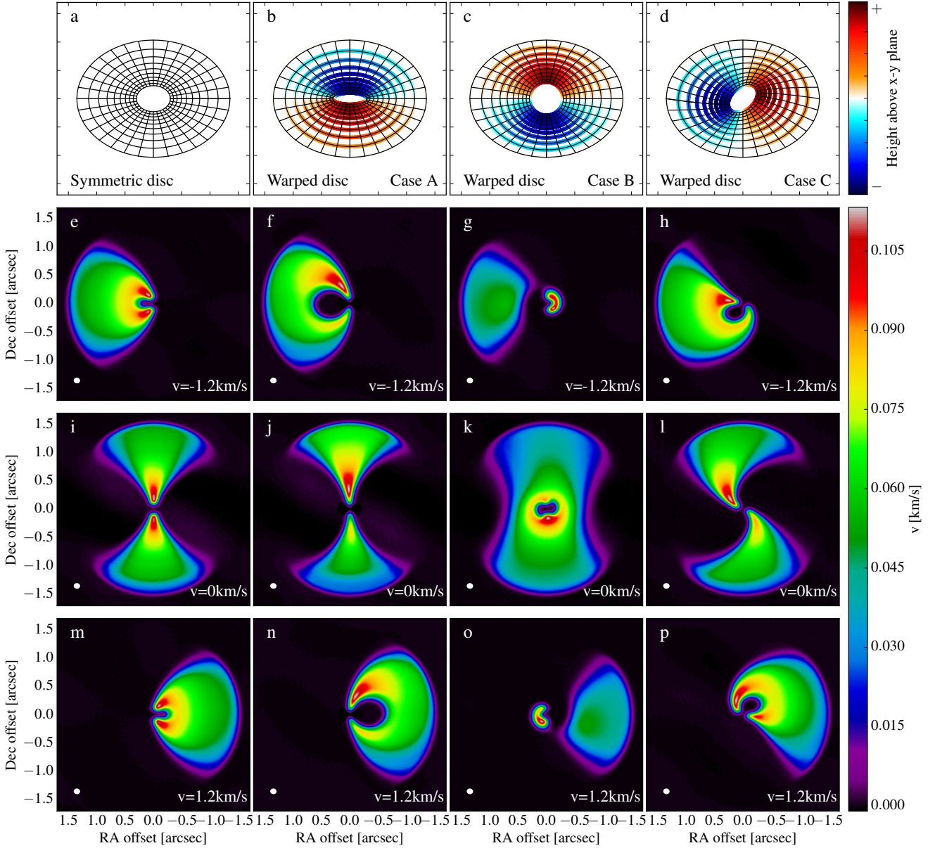
Figure 10. Predicted channel maps of warped disc in the CO J=3-2 line in ALMA observations. Panels a–d shows a cartoon depicting the structure and orientation of the warp. The left column shows the channel maps of an unperturbed disc for reference. The channel maps are shown at v = -1.2 km/s (Panel e–h ), v = 0 km/s (Panel i–l ), v = +1.2 km/s (Panel m–p ), respectively. The inclination of the outer disc is i = 10^\circ .
