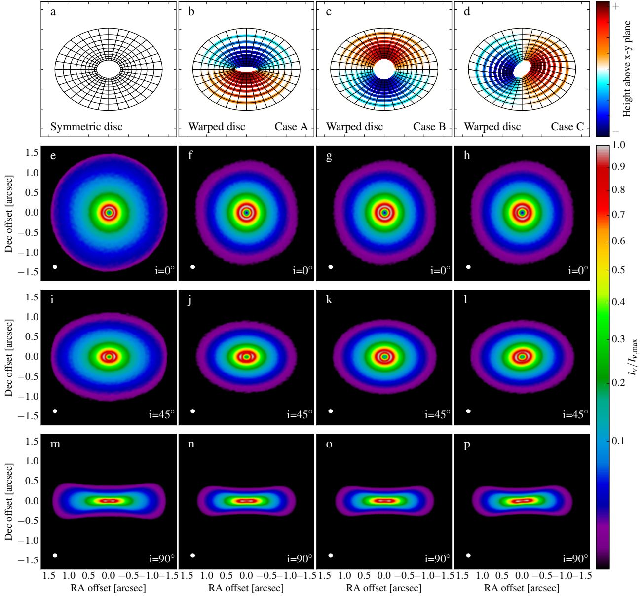
Figure A2. Same as Figure 6, but for the weakest warp in our simulations with \alpha = 0.02 and \beta_0 = 15^\circ . In most cases such weak warping does not cause any observable deviation in the surface brightness distribution from that of an unperturbed disc. The warping is only visible in panels l and p , i.e. if the disc is bending perpendicular to the line of sight. In this case the warping of the disc causes the position angle of the isophotes to change with radius.
