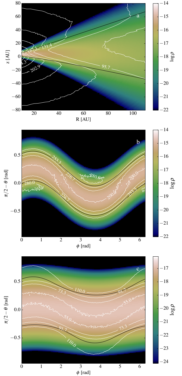
Figure 4. Density and temperature structure of a warped circumbinary disc in a vertical slice in the rz -plane at \phi = 0^\circ (a) and in the \phi - \theta surface at r = 12 au (b) and at r = 100 au (c). The colour-scale image shows the logarithm of the dust density in the disc while the white contours show the dust temperature. The black contour shows the location of the radial optical depth of unity at 0.5 \mu\text{m} .
