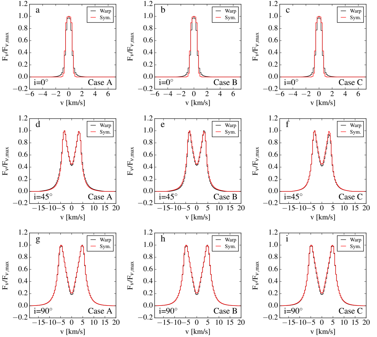
Figure A3. Same as Figure 7, but for the weakest warp in our simulations with \alpha = 0.02 and \beta_0 = 15^\circ . The warping of the disc in this model is so low that the deviation of the line-profile from that of an unperturbed disc is only visible if the outer disc is seen face-on. At moderate to high inclination angles the line profile of such weakly warped disc and that of an unperturbed symmetric disc is indistinguishable from each other. In real observations with realistic noise levels the detection of a warp can be challenging even at very low inclination angles.
