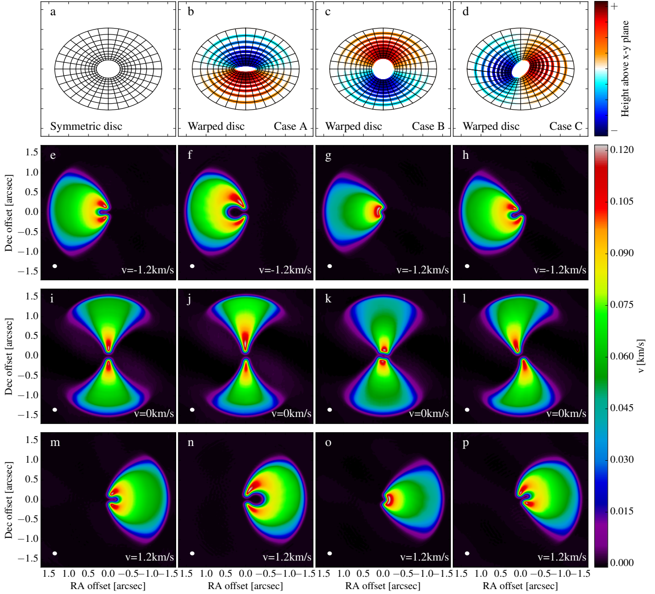
Figure A5. Same as Figure 10, but for the weakest warp in our simulations with \alpha = 0.02 and \beta_0 = 15^\circ . In this case \beta'(r_{\text{in}}) = 5.9^\circ . Since the assumed inclination angle is larger ( i = 10^\circ ) no apparent counter rotation occurs. However, the warping of the disc is visible if the disc bends perpendicular to the line of sight (Case C) as the emission at the zero velocity channel becomes twisted. If the disc bends along the line of sight (Case A/B), warping of the disc becomes difficult to recognise, especially in Case A.
