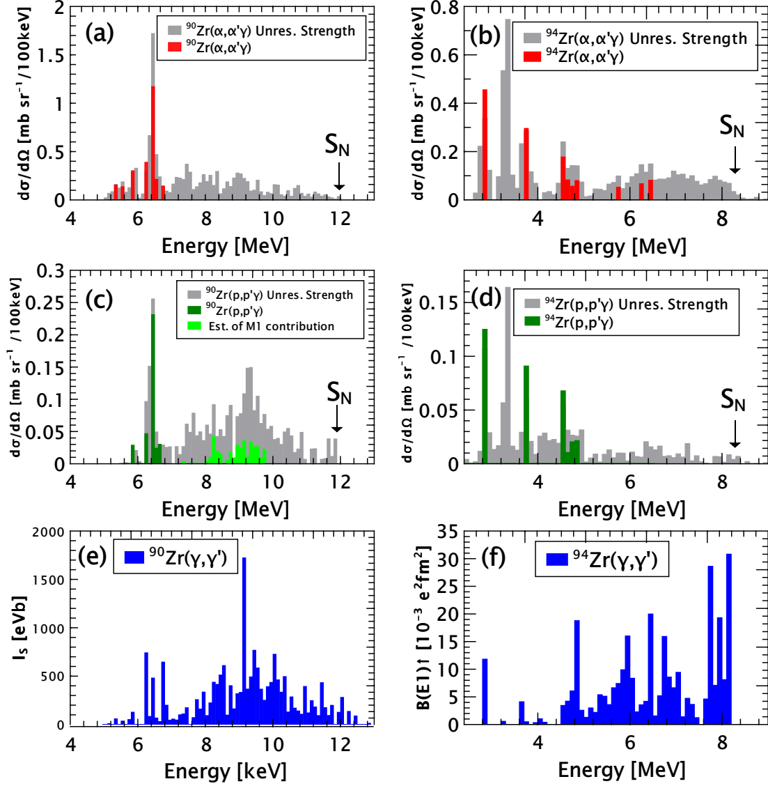
Figure 2: Cross section for the excitation of dipole states from different reaction types for the nuclei ^{90}\text{Zr} and ^{94}\text{Zr} . Panels (a) and (b) are for the (\alpha, \alpha') \gamma reaction at 130 MeV, panels (c) and (d) are for the (p, p') \gamma reaction at 80 MeV, while panels (e) and (f) show (\gamma, \gamma') measurements from references [15] and [16]. The coloured bars correspond to discrete transitions while the grey bars correspond to the continuum regions in the present measurements. In panel (c) the estimated contribution from 1^+ states obtained using the measured M1 strength from [17] is shown in the grey area with light green bars.
