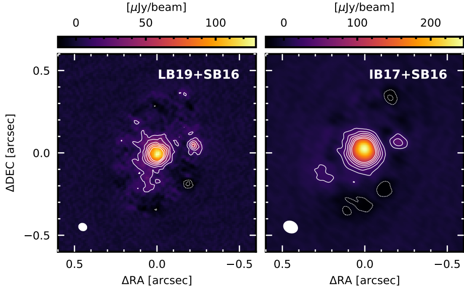
Figure 2. Residual images obtained after subtracting the Fourier transform of the CLEAN model for the outer ring (referred to as ‘cavity images’), obtained with the new data (LB19+SB16; left) and the data published in Isella et al. (2019) (IB17+SB16; right) considering a Briggs robust parameter of 1. Contours are 3 to 18 times the rms noise level ( 4.7 and 6 \mu\text{Jy beam}^{-1} , respectively), spaced in steps of 3\sigma . Dashed contours correspond to -3\sigma . A gallery of cavity images is given in Appendix A.2 .
