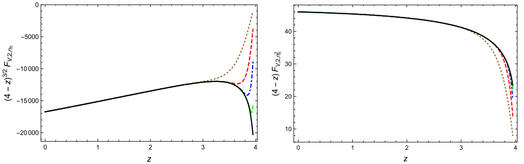
Fig. 9. The vector form factor F_{V,2} in the threshold region as a function of z : left \varepsilon^0 n_h^1 , right \varepsilon^0 n_h^2 , the approximation with 20, 50, 100, 200, 500 terms is shown in brown, red, blue, green and black, respectively.
