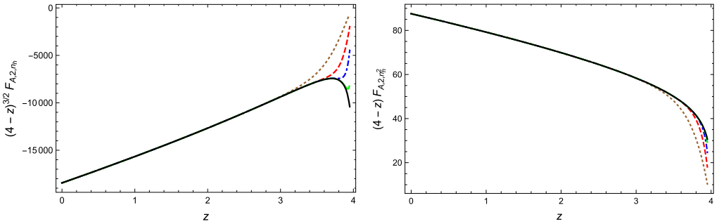
Fig. 11. The axialvector form factor F_{A,2} in the threshold region as a function of z : left \varepsilon^0 n_h^1 , right \varepsilon^0 n_h^2 , the approximation with 20, 50, 100, 200, 500 terms is shown in brown, red, blue, green and black, respectively.
