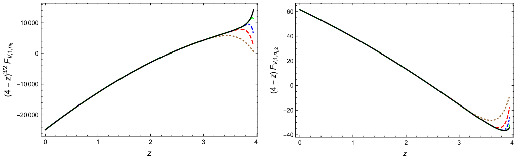
Fig. 8. The vector form factor F_{V,1} in the threshold region as a function of z : left \varepsilon^0 n_h^1 , right \varepsilon^0 n_h^2 , the approximation with 20, 50, 100, 200, 500 terms is shown in brown, red, blue, green and black, respectively.
