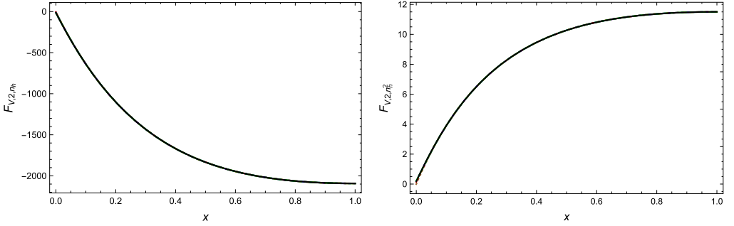
Fig. 2. Vector form factor F_{V,2} : left \varepsilon^0 n_h^1 , right \varepsilon^0 n_h^2 , the approximation with 20, 50, 100, 200, 500 terms is shown in brown, red, blue, green and black, respectively.
