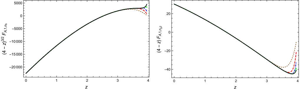
Fig. 10. The axialvector form factor F_{A,1} in the threshold region as a function of z : left \varepsilon^0 n_h^1 , right \varepsilon^0 n_h^2 , the approximation with 20, 50, 100, 200, 500 terms is shown in brown, red, blue, green and black, respectively.
