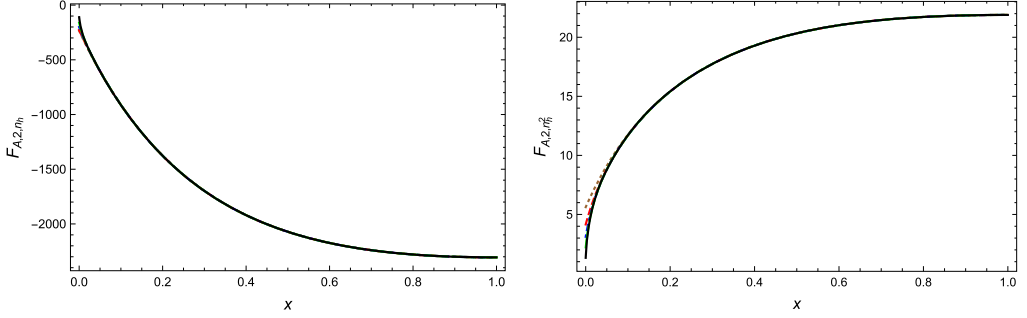
Fig. 4. Axial vector form factor F_{A,2} : left \varepsilon^0 n_h^1 , right \varepsilon^0 n_h^2 , the approximation with 20, 50, 100, 200, 500 terms is shown in brown, red, blue, green and black, respectively.
