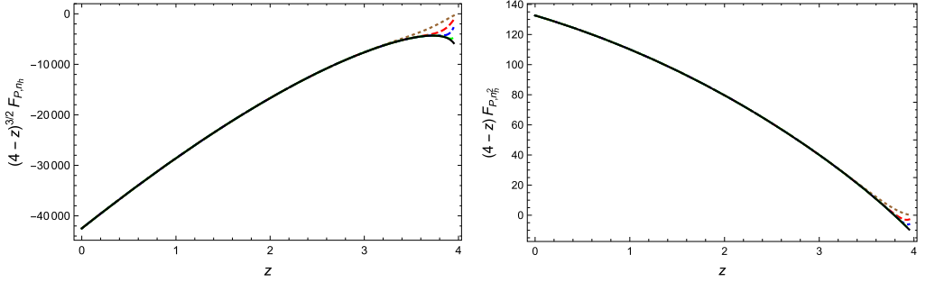
Fig. 13. The pseudoscalar form factor F_P in the threshold region as a function of z : left \varepsilon^0 n_h^1 , right \varepsilon^0 n_h^2 , the approximation with 20, 50, 100, 200, 500 terms is shown in brown, red, blue, green and black, respectively.
