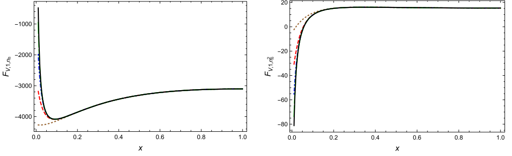
Fig. 1. Vector form factor F_{V,1} : left \varepsilon^0 n_h^1 , right \varepsilon^0 n_h^2 , the approximation with 20, 50, 100, 200, 500 terms is shown in brown, red, blue, green and black, respectively. (For interpretation of the colors in the figure(s), the reader is referred to the web version of this article.)
