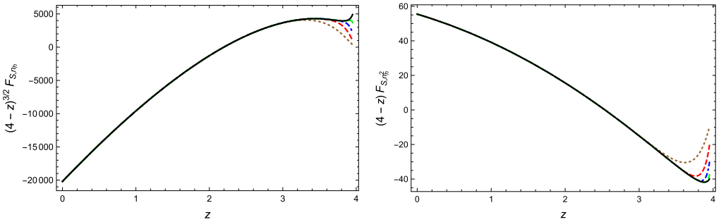
Fig. 12. The scalar form factor F_S in the threshold region as a function of z : left \varepsilon^0 n_h^1 , right \varepsilon^0 n_h^2 , the approximation with 20, 50, 100, 200, 500 terms is shown in brown, red, blue, green and black, respectively.
