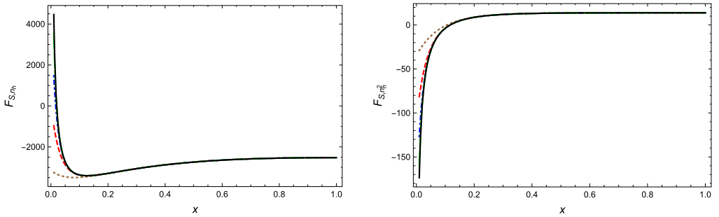
Fig. 6. Scalar form factor F_S : left \varepsilon^0 n_h^1 , right \varepsilon^0 n_h^2 , the approximation with 20, 50, 100, 200, 500 terms is shown in brown, red, blue, green and black, respectively.
