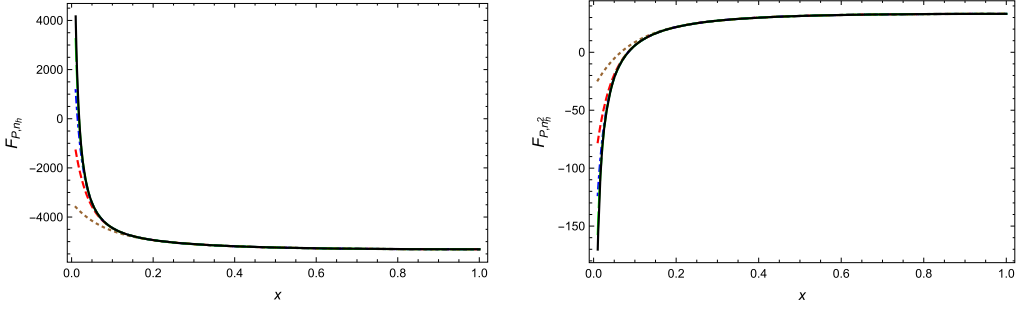
Fig. 7. The pseudoscalar form factor F_P : left \varepsilon^0 n_h^1 , right \varepsilon^0 n_h^2 , the approximation with 20, 50, 100, 200, 500 terms is shown in brown, red, blue, green and black, respectively.
