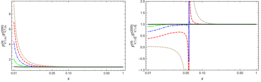
Fig. 5. Ratios of the approximations with 20, 50, 100, 200, 500 terms and our best approximation using 2000 terms for the vector form factor F_{V,1} . Left \varepsilon^0 n_h^1 , right \varepsilon^0 n_h^2 . The ratio using 20, 50, 100, 200, 500 terms is shown in brown, red, blue, green and black, respectively.
