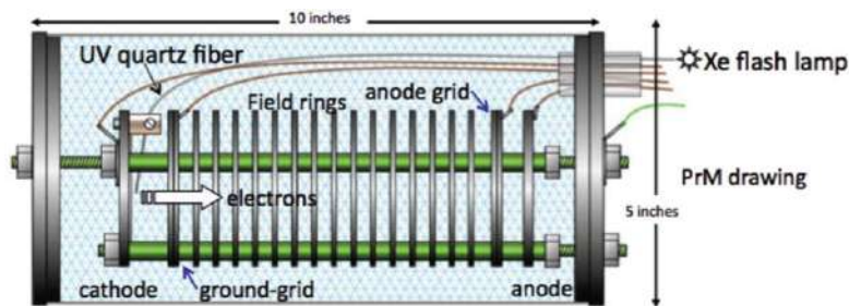
Figure 55: Schematic diagram of the purity monitor design [16].
