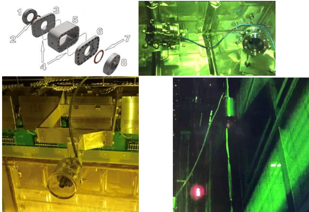
Figure 65: Top left: a CAD exploded view of a vacuum-tight camera enclosure suitable for cryogenic applications [35]. Its numbered features are (1) quartz window, (2 and 7) copper gasket, (3 and 6) flanges, (4) indium wires, (5) body piece, (8) signal feedthrough. Top right: two of the ProtoDUNE-SP cameras in stainless steel enclosures similar to the CAD design on the top left. Bottom left: one of the cameras in an acrylic enclosure. Bottom right: a portion of an image taken with camera 105 showing a purity monitor mounted outside the APA on the beam-left side. This photo was taken with ProtoDUNE-SP completely filled.
