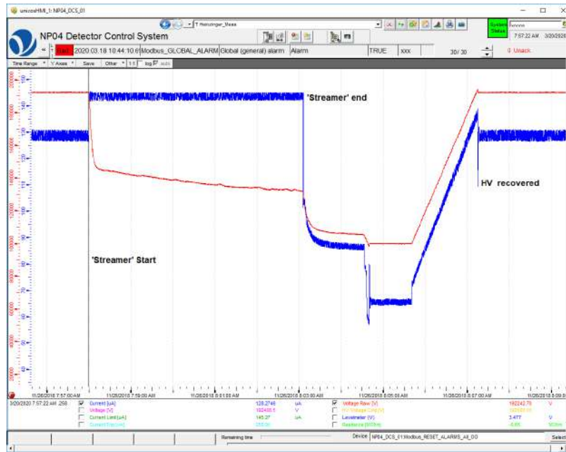
Figure 26: Automatic Recovery of a ‘streamer’ event recorded on 26/11/2018 by DCS. The HV current (in blue) is limited at 142 \mu\text{A} ; the voltage (in red) decreases until the discharge is finished, returning to the nominal voltage after a predefined time.
