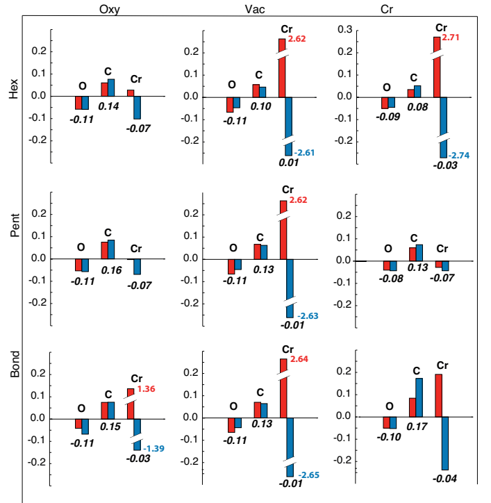
Fig. 2 Spin resolved (red, majority; blue, minority) charge transfer averaged over the O and Cr atoms at and around the adsorption site (see the text for details) together with the average value on the C atoms facing to the surface. The total charge transfer (spin up + spin down) averaged over the same atoms is reported in bold below the block histograms. For the systems that display AFM patterns (except Bond/Cr ) the spin dependent charge transfer of Cr is out of scale (see the text) and the actual value is reported in red and blue for spin up and spin down, respectively.
