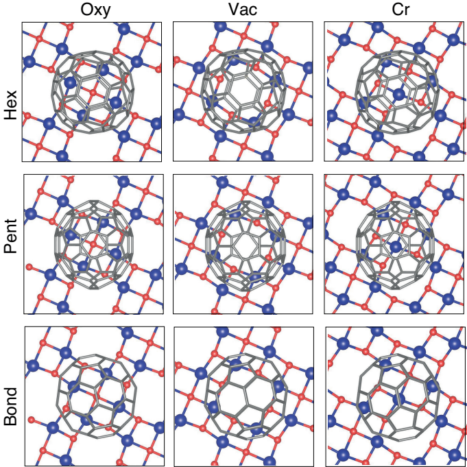
Fig. 1 Top view of the explored configurations, depending on adsorption site and relative orientation between C_{60} and Cr_4O_5 . The color code is as follows: Cr - blue, O - red and C - grey. The Fe substrate layers are not shown.
