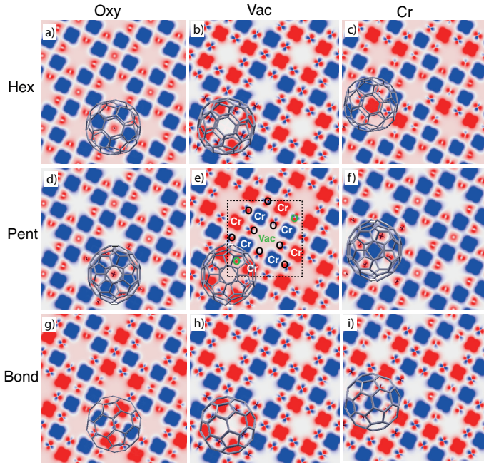
Fig. 3 Spin polarization \rho_{up} - \rho_{down} for each pattern (top view). A cut on the surface plane passing through the Cr atoms is reported with an isosurface value of 0.02 \text{ \AA}^{-3} . Red and blue areas correspond to positive and negative values of spin polarization, respectively.
