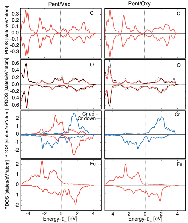
Fig. 4 PDOS on Fe and Cr ( d component), O and C atoms facing to the surface ( p -component) for the Pent/Vac (left) and Pent/Oxy (right) configurations. Two representative Cr atoms with opposite polarization are reported for the AFM configuration. For O we report as a red line the PDOS averaged over the cell, and as a black dashed line that averaged on the four nearest neighbours to C_{60} in the Pent/Vac configuration, and that of the O below C_{60} for the Pent/Oxy case.
