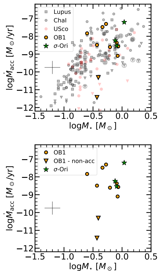
Fig. 15. Relation between the mass accretion rates and stellar mass obtained from the X-Shooter for the PENELLOPE targets in the Orion region. The top panel shows the comparison with data obtained with the same technique in the literature, while the bottom panel highlights solely the new results from this work.
