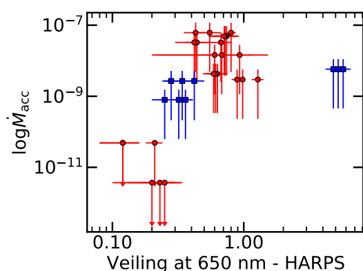
Fig. 10. Veiling measured on the UVES (red) and ESPRESSO (blue) spectra using the HARPS template versus the M_{\text{acc}} measured for each target from the X-Shooter spectra. Each target was observed three times with UVES or ESPRESSO, and only once with X-Shooter.
