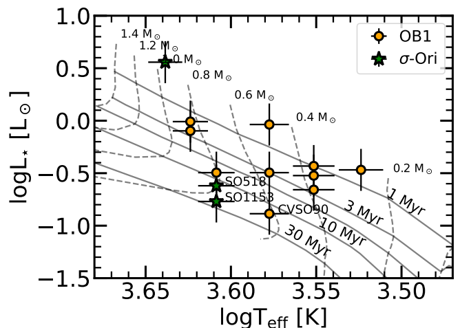
Fig. 5. Hertzsprung-Russel diagram (HRD) of the Orion targets, with evolutionary tracks from Baraffe et al. (2015). The isochrones shown here are for ages of 1, 3, 5, 10, and 30 Myr.
