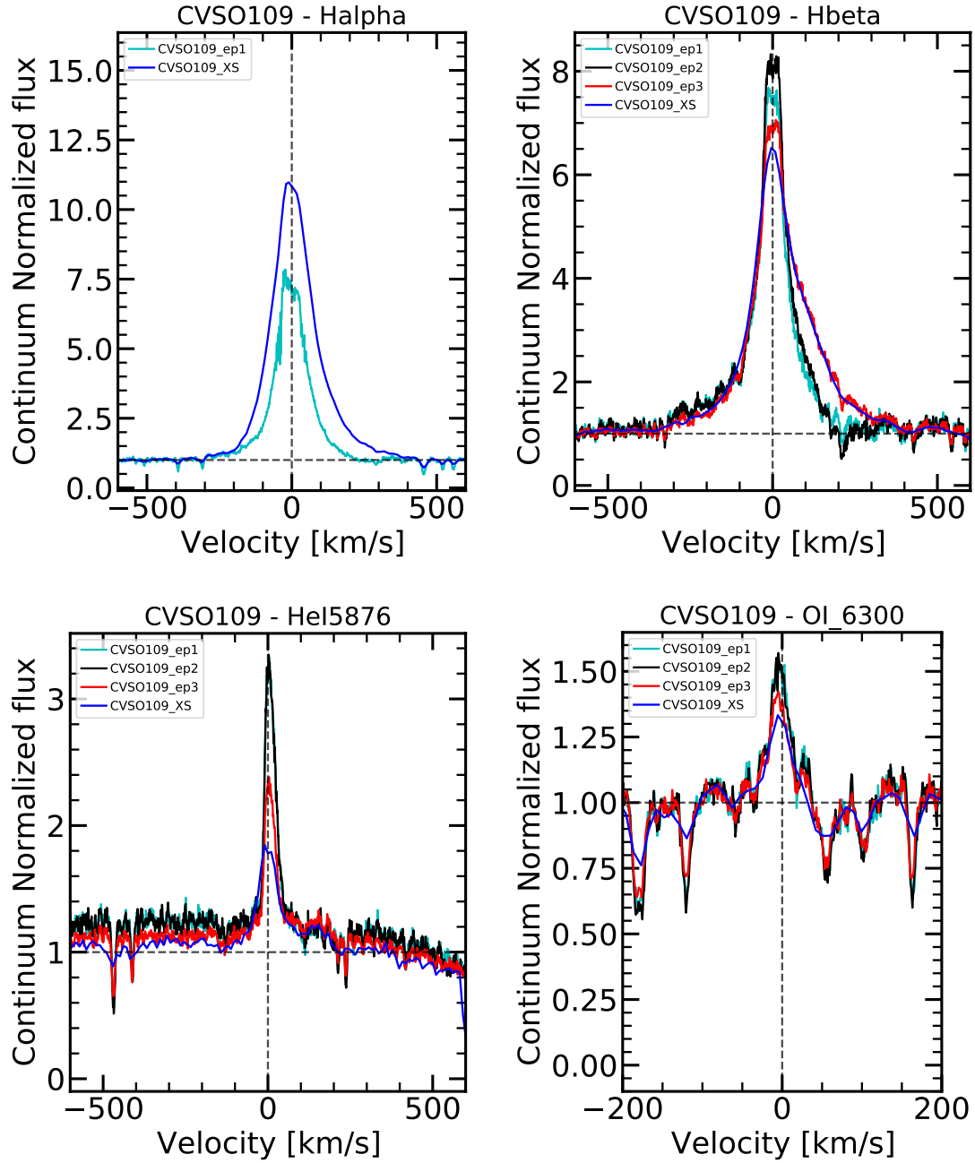
Fig. G.7. Emission lines of the target CVSO109 observed with UVES and X-Shooter. In the second and third epoch of UVES observations of CVSO109 the H \alpha line is saturated, and this is therefore not shown here.
