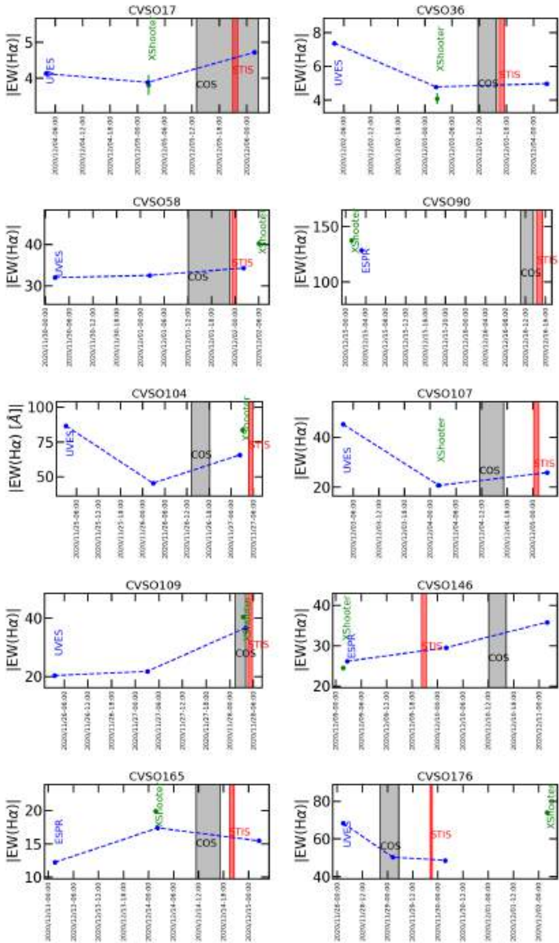
Fig. B.1. Variability of the H \alpha equivalent width for the Orion OB1 targets as measured by EPRESSO or UVES (blue) and X-Shooter (green), Article number, page 22 of 46 Article number, page 22 of 46 Article number, page 22 of 46
