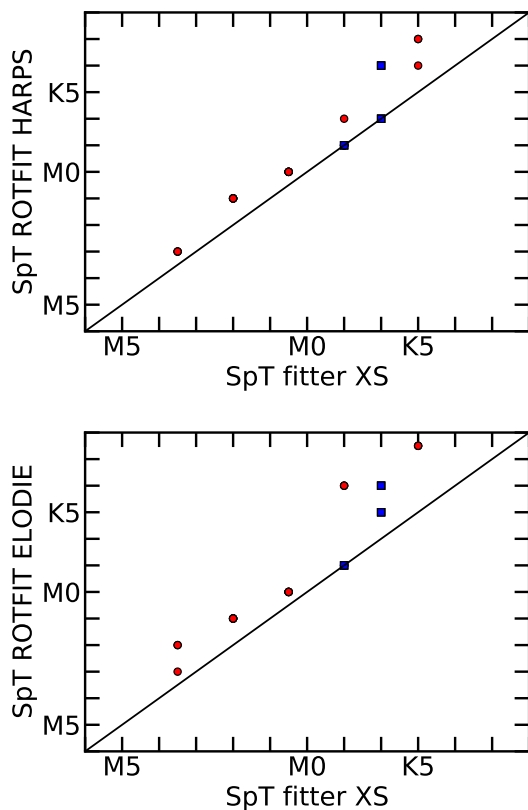
Fig. 7. Spectral type (SpT) derived with ROTFIT on the UVES (red) and ESPRESSO (blue) spectra vs SpT from the fit of the X-Shooter spectra. Top: ROTFIT results using the HARPS templates, bottom: ROTFIT results using the ELODIE templates.
