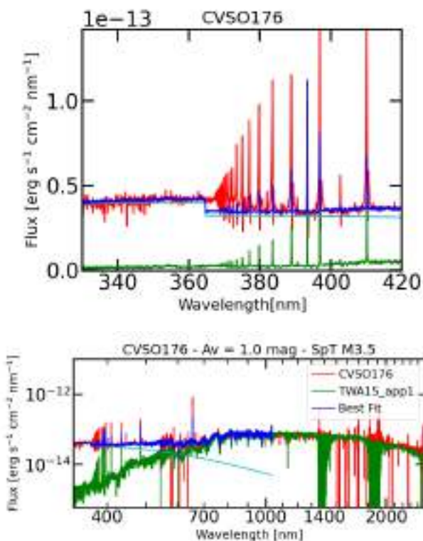
Fig. 4. Example of a best fit for the X-Shooter spectrum of CVSO176 obtained with the fitter described in Sect. 2.5.1. The spectrum of the target is shown with a red line, the best fit photospheric template with a green line, the slab model with a cyan line, and the best-fit sum of the template and slab model with a blue line. The best fit is only shown up to 1000 nm, since the contribution from the disk emission can be significant at longer wavelengths.
