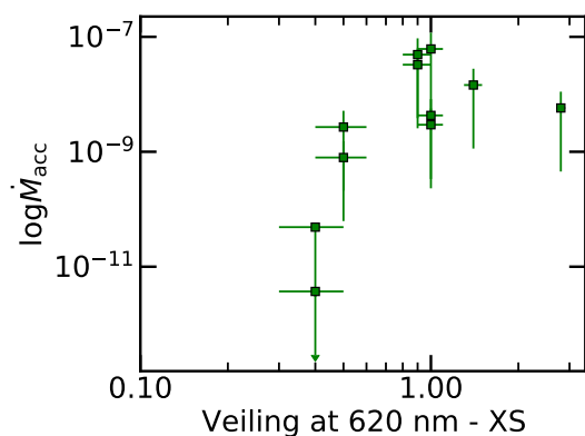
Fig. 11. Veiling measured on the X-Shooter spectra vs the M_{\text{acc}} measured for each target from the same spectra.
