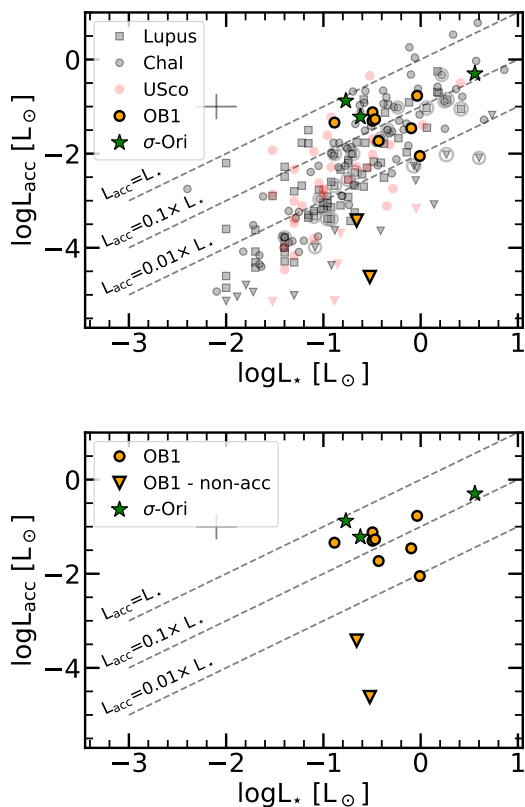
Fig. 14. Relation between the accretion luminosity and stellar luminosity obtained from the X-Shooter for the PENELLOPE targets in the Orion region. The top panel shows the comparison with data obtained with the same technique in the literature, while the bottom panel highlights solely the new results from this work.
