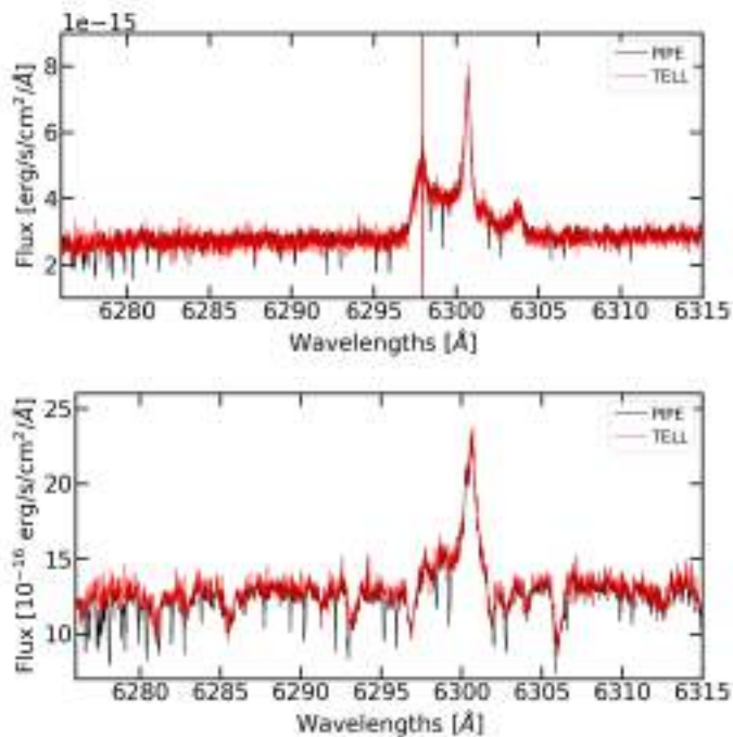
Fig. 3. Example of telluric correction in the region of the [OI]6300Å line for the ESPRESSO spectrum of CVSO 90 performed with molecfit (top) and for the UVES spectrum of CVSO 58 carried out with a standard telluric (bottom). The black spectrum is obtained from the pipeline reduction, and the red one shows the telluric corrected spectrum.
