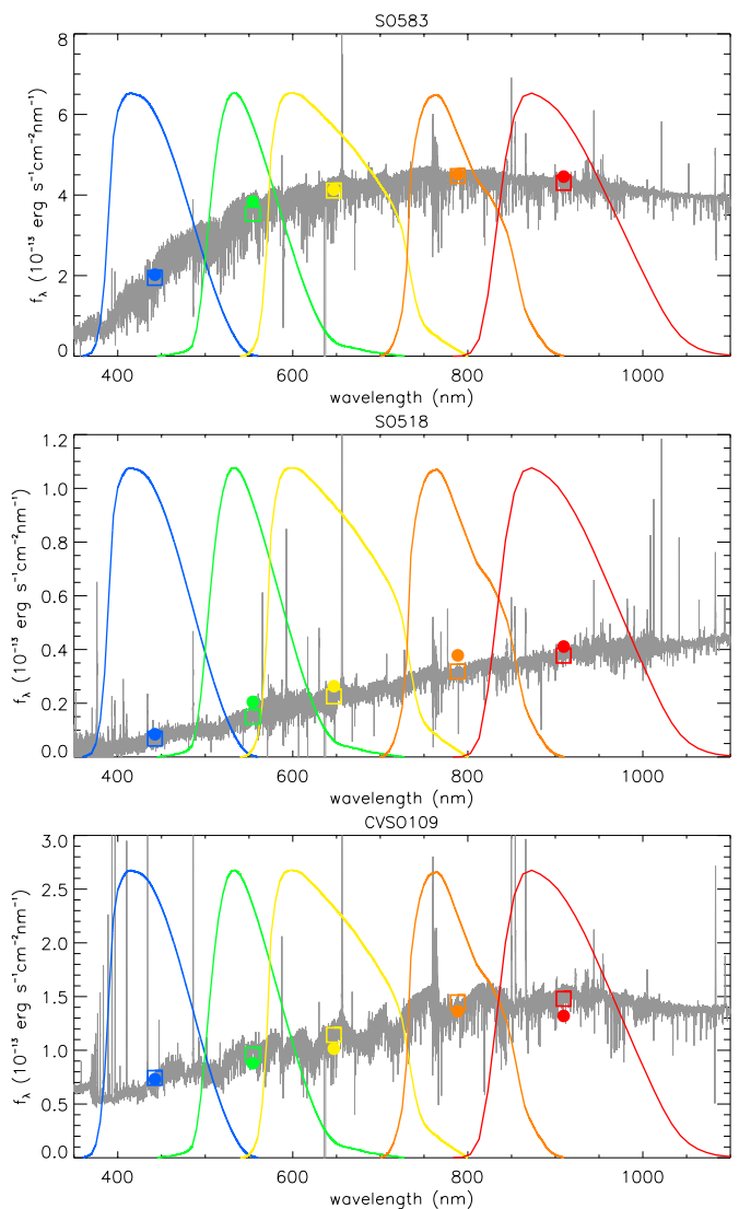
Fig. 2. X-Shooter flux-calibrated spectrum of three of our targets (grey), as labelled, with quasi-simultaneous photometry for the same target obtained from OACT in the BVRcIcz' bands (dots). The filter bandpasses and the synthetic photometry (open squares) obtained integrating the spectrum over these bandpasses are overlaid.
