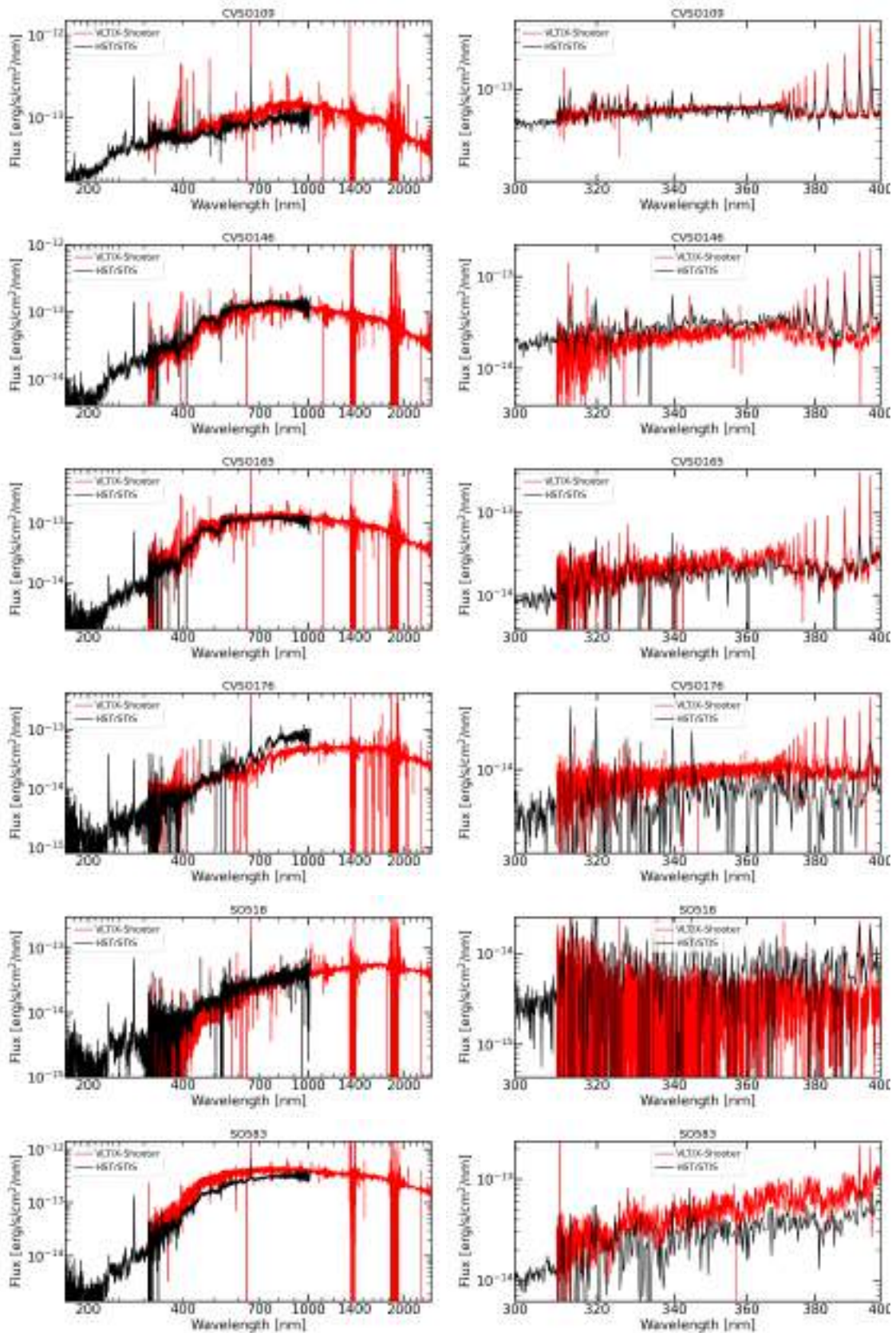
Fig. F.2. Comparison between the observed VLT/X-Shooter (red) and HST/STIS (black) spectra.
