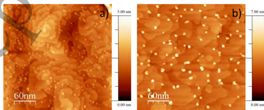
Figure 3. STM topography images of FeSe thin films grown at 420^\circ\text{C} and the substrate-to-target distance of about 5 cm (a) and 10 cm (b), respectively.
