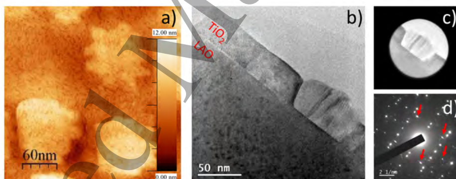
Figure 7. (a) STM topography images of a \text{TiO}_2 thin film grown at substrate-to-target distance of about 5 cm; (b) cross-sectional HRTEM of the same films in the proximity of the flower-shaped structure; (c-d) SAED of a flower-shaped domain (red arrows correspond to diffraction spots associated to the rutile phase).
