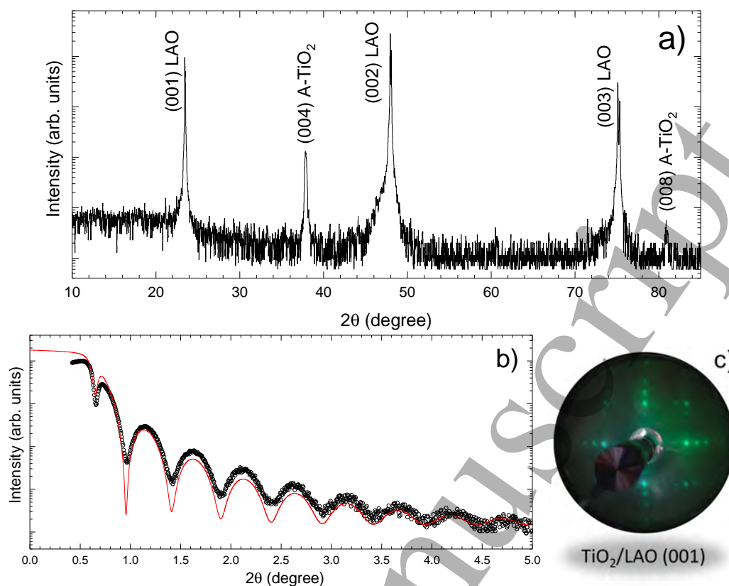
Figure 6. (a) symmetrical \theta - 2\theta and (b) low-angle x-ray reflectivity scans of an anatase \text{TiO}_2 film grown on \text{LaAlO}_3 (001) substrate (simulation of low-angle x-ray reflectivity is also reported as red solid line); (c) typical LEED pattern of \text{TiO}_2 showing the (4 \times 1)-(1 \times 4) surface reconstruction.
