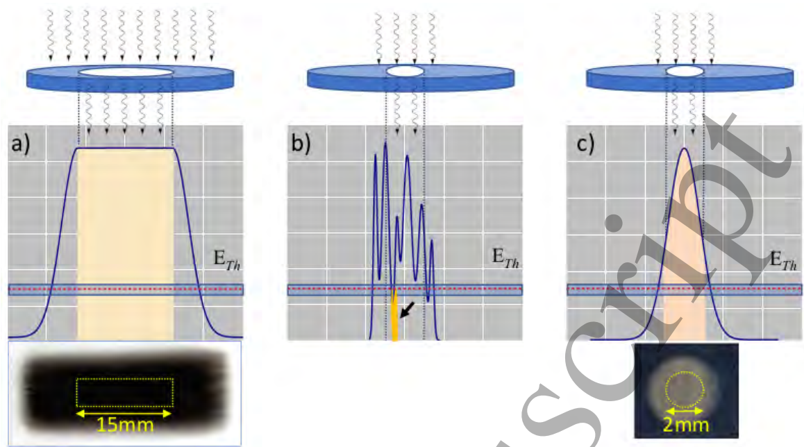
Figure 1. Typical energy profile of a KrF excimer (a), an early-stage (b) and a new-generation state-of-the-art (c) Nd:YAG lasers, respectively; for all of the laser spot, the effect of using a shadow-mask (blue) to tentatively improve the uniformity of the energy profile is shown; threshold energy E_{Th} (red dotted line) is also reported; in particular, in the case of the inhomogeneous laser beam (b), sub-threshold region (yellow) is enlightened by a black arrow. Energy profiles obtained by thermal paper at the output of the laser window are also reported for a KrF (a) and a state-of-the-art Nd:YAG (c) lasers, respectively.
