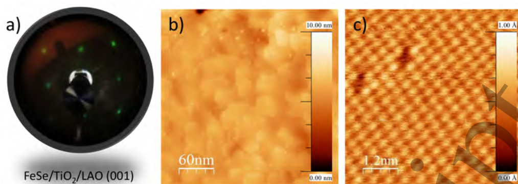
Figure 11. (a) LEED pattern showing the FeSe 1x1 surface reconstruction and STM topography image (b) of a FeSe/TiO 2 bilayer grown on LAO substrate. (c) atomically resolved STM topography of the same FeSe/TiO 2 bilayer.
