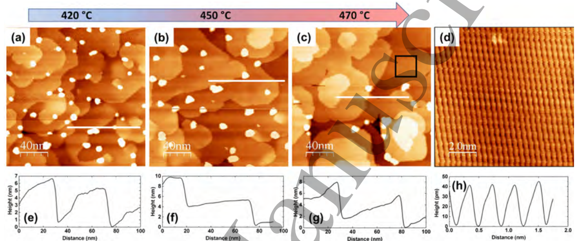
Figure 4. STM topography images of FeSe thin films grown at substrate-to-target distance of 10 cm and at different temperatures (namely 420° (a), 450° (b) and 470° (c), respectively, in the scan area of 200 \times 200 \text{ nm}^2 . The atomic resolution of the zoomed area marked as the black box in (c) in the scan area of 12 \times 12 \text{ nm}^2 . The corresponding line-profiles of all the samples are shown in e-h graphs.
