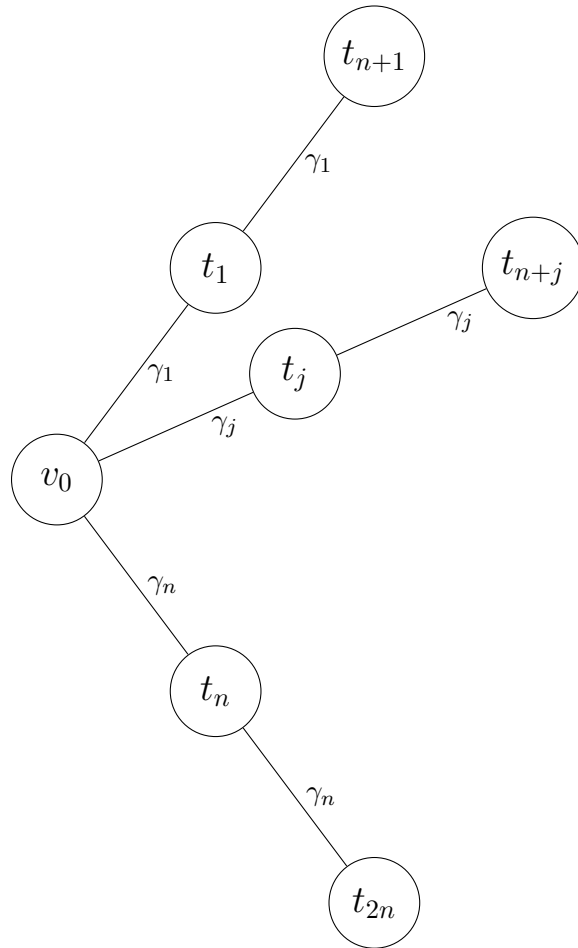
Figure 6: Special 2-level star graph.
