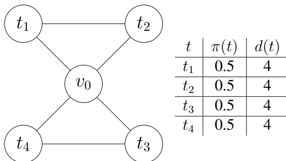
Figure 1: Example of patrolling setting.
