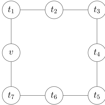
Figure 5: Cycle graph.
