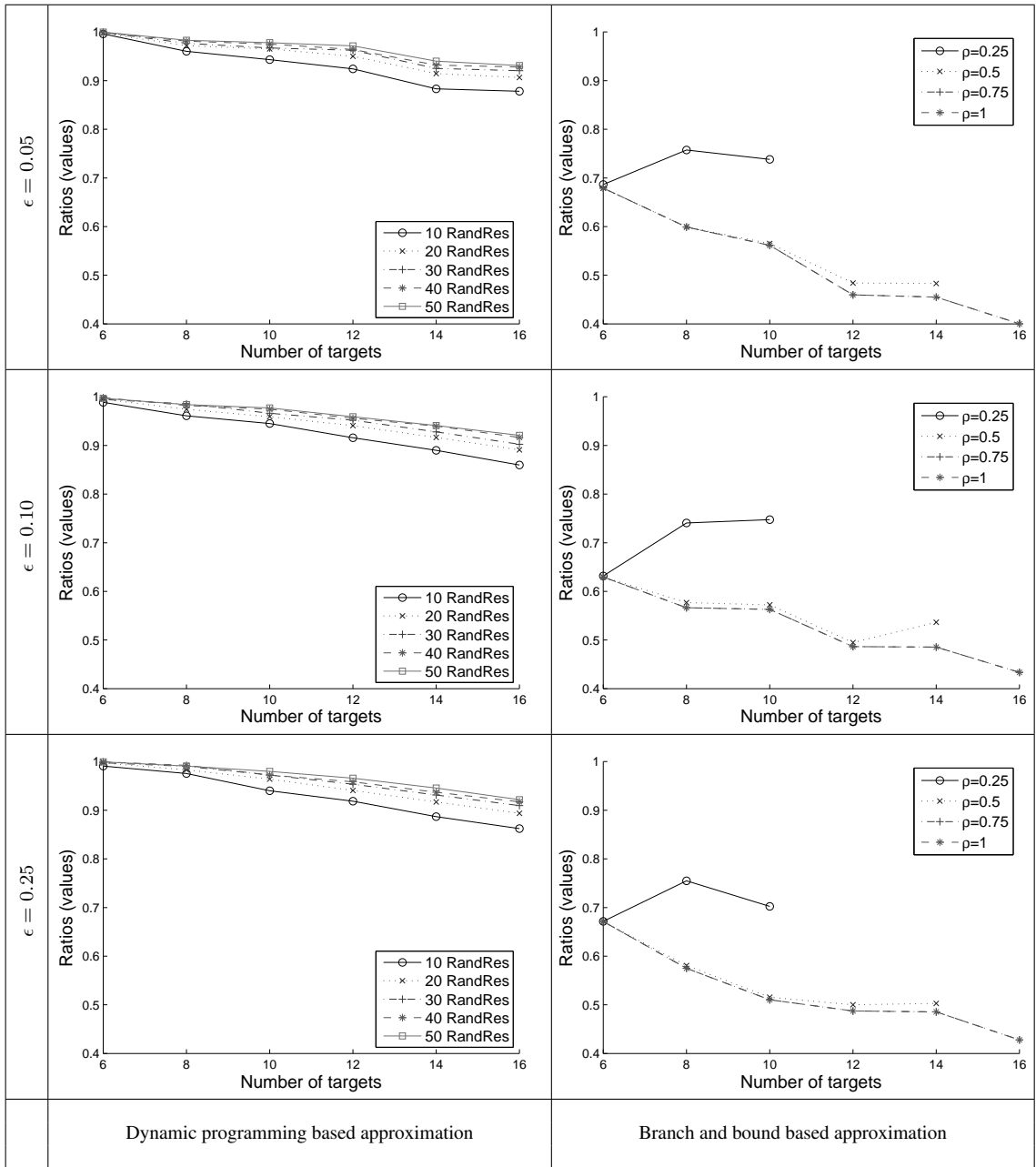
Figure 13: Approximation ratios as |T| varies.
