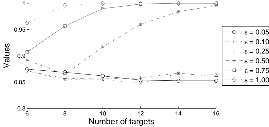
Figure 12: Optimal game values as |T| and \epsilon vary.
