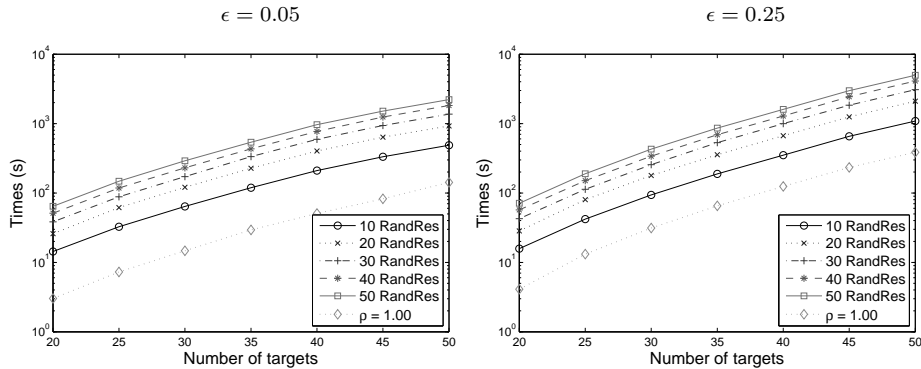
Figure 16: Time ratios as |T| varies.
