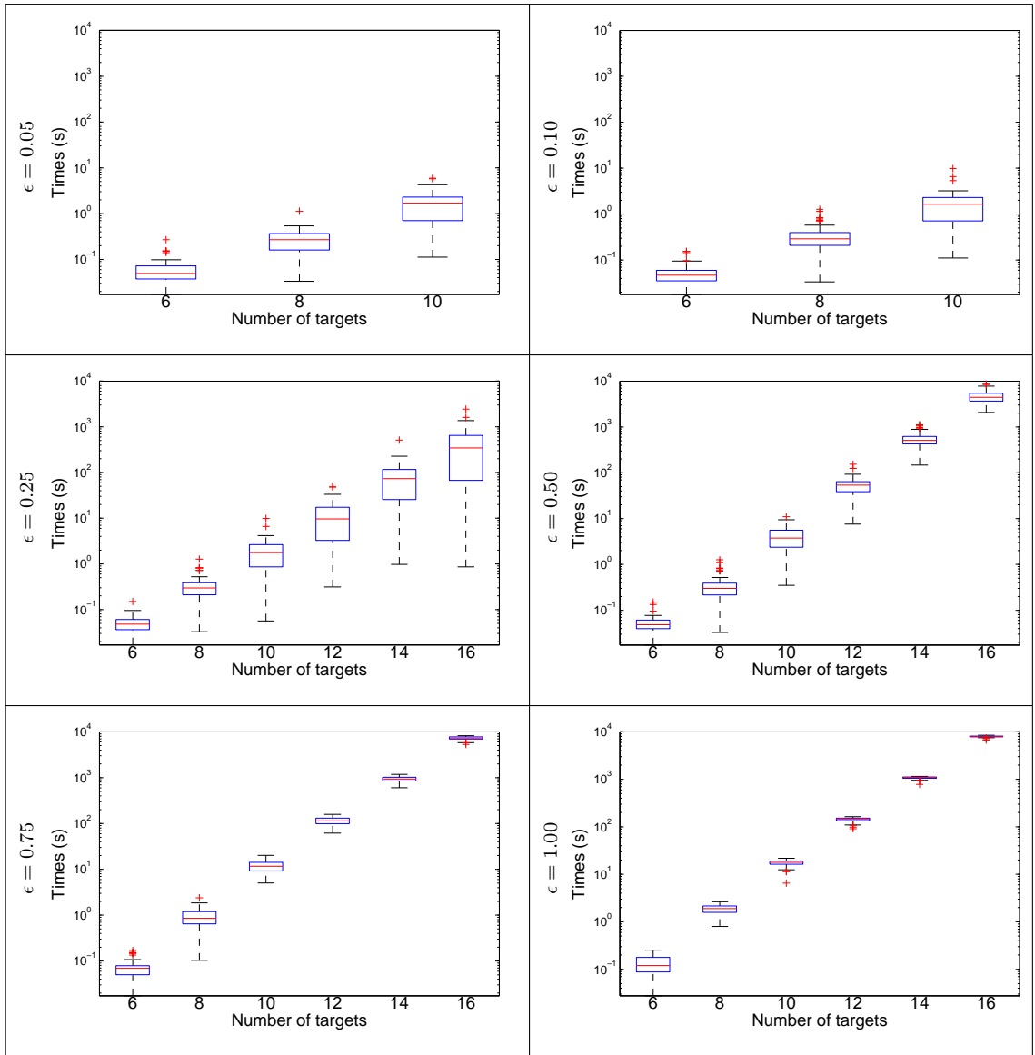
Figure B.21: Boxplots of compute times required by our exact dynamic programming algorithm.
