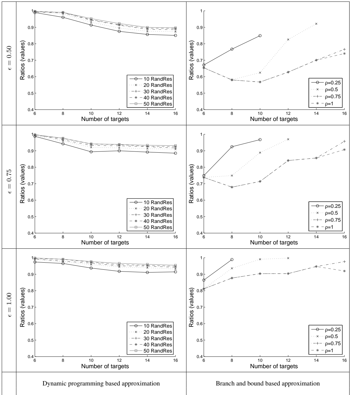
Figure 14: Approximation ratios as |T| varies.
