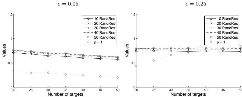
Figure 15: Game values as |T| varies.
