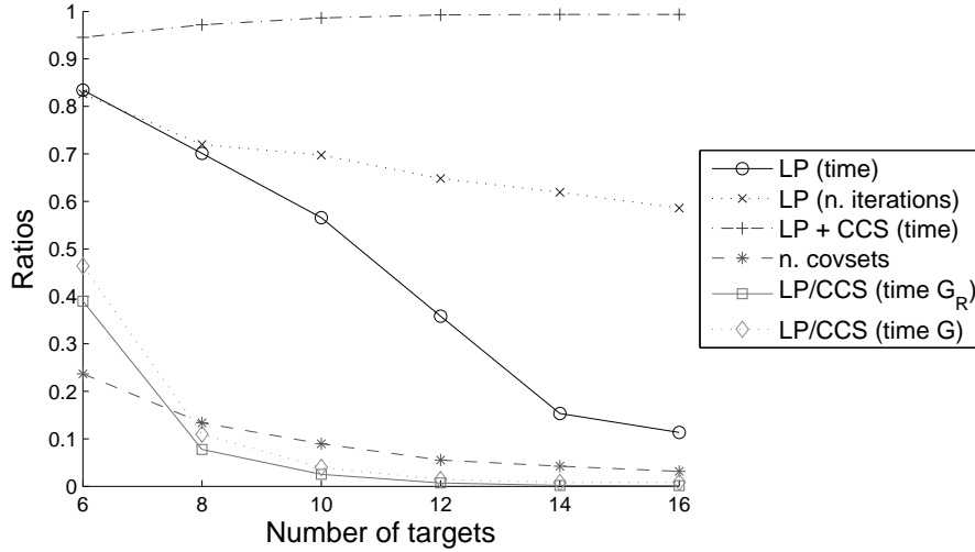
Figure 11: Ratios evaluating dominances with \epsilon = 0.25 as |T| varies.
