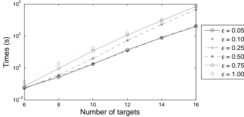
Figure 10: Compute times in seconds of our exact dynamic programming algorithm (Algorithm 1), with the annotation of dominated (proper) covering sets and the generation of the routes, as |T| and \epsilon vary.
