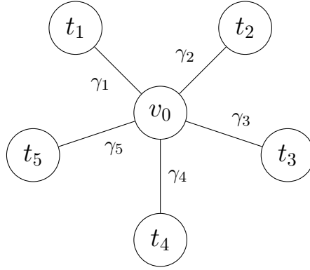
Figure 7: Star graph.
