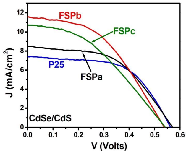
Figure 8. Current-voltage curves obtained with a quantum dot sensitized solar cell carrying various CdSe/CdS/TiO 2 /FTO photoanodes and a Cu 2 S/brass counter electrode. The polysulfide electrolyte contained 1.0 M Na 2 S + 1.0 M S.
