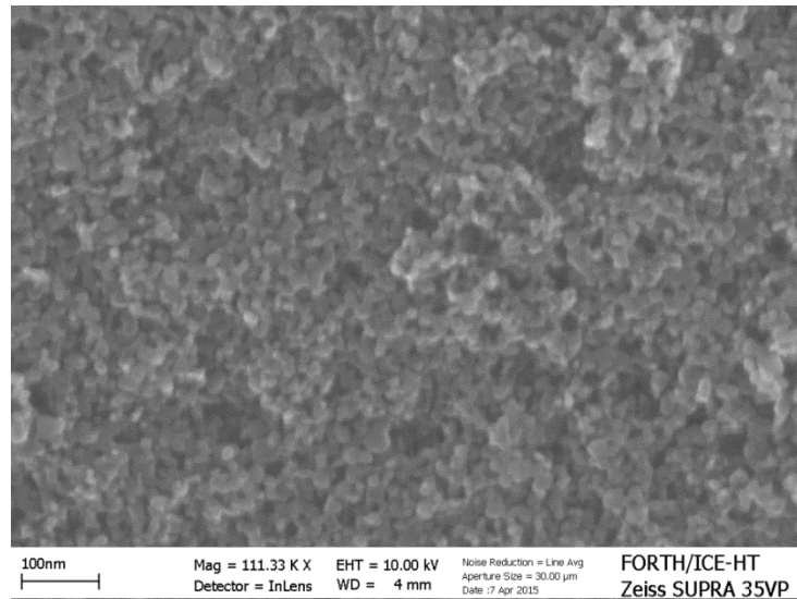
Figure 2. FESEM image of a film made by depositing a paste of FSPb powder followed by calcination. The scale bar is 100 nm, the particle sizes range between 7 and 15 nm.
