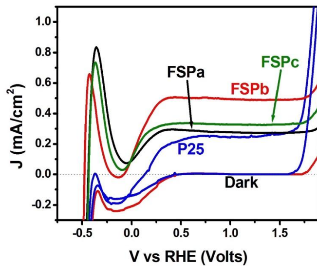
Figure 4. Current-Voltage curves obtained with a photoelectrochemical cell comprising a photoanode made of various titania films. The two dark curves at the bottom correspond to P25 and FSPb. The electrolyte contained only 0.5 M NaOH.
