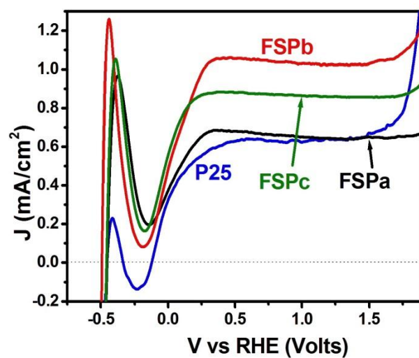
Figure 5. Current-voltage curves obtained with a photoelectrochemical cell comprising a photoanode made of various titania films. The electrolyte solution contained 0.5 M NaOH + 5 % v/v ethanol.
