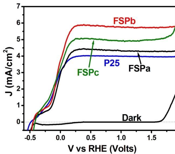
Figure 6. Current-voltage curves obtained with a photoelectrochemical cell comprising various CdS/TiO 2 /FTO photoanodes. The electrolyte contained 0.5 M NaOH + 5 % v/v ethanol.
