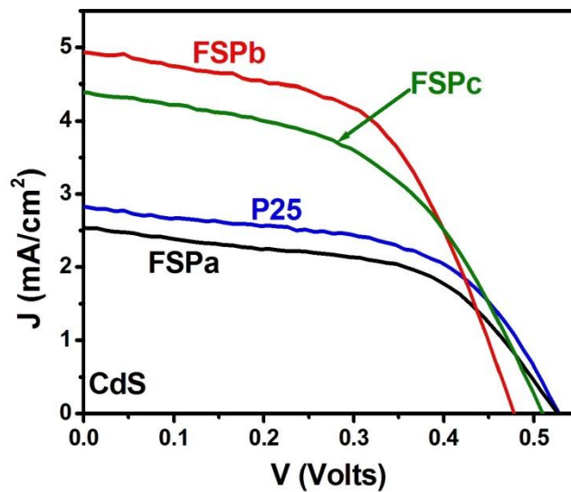
Figure 7. Current-voltage curves obtained with a quantum dot sensitized solar cell with various CdS/TiO 2 /FTO photoanodes and a Cu 2 S/brass counter electrode. The polysulfide electrolyte contained 1.0 M Na 2 S + 1.0 M S.
