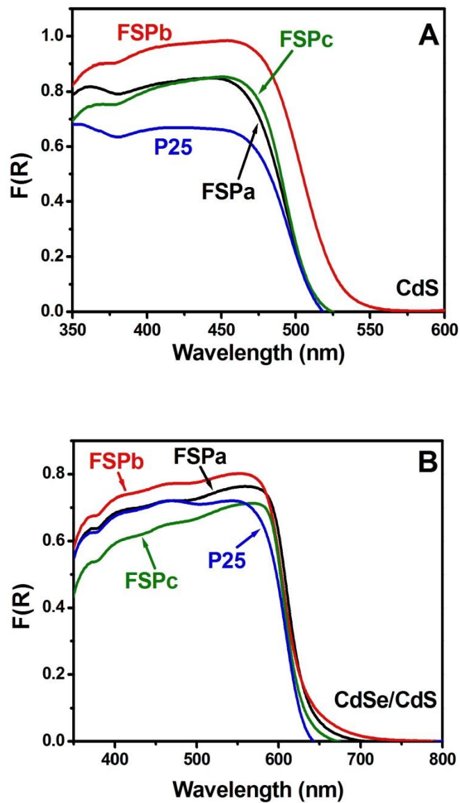
Figure 3. Diffuse reflection spectra of (A) CdS/TiO 2 /FTO and (B) CdSe/CdS/TiO 2 /FTO photoanodes made with the various titania powders. The amount of titania was ca. 3 mg cm -2 in each film.
