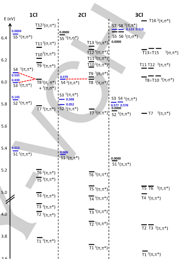
Figure 10. Scheme of singlet and triplet electronic levels with oscillator strengths (only for singlet states, in blue) and character for 1CI (left), 2CI (centre) and 3CI (right) at \omega B97X/6-311++G(d,p) level of theory.
