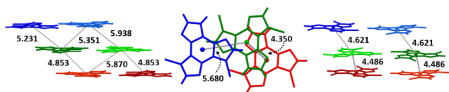
Figure 2. Fragments of crystal packing of 1CI (left), 2CI (center) and 3CI (right) showing three overlapped layers in different colors viewed from side or top (dark/light colors for A/B molecules of 1CI and 3CI ) and distances (in Å) between triazine centroids.
