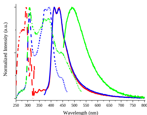
Figure 7. Normalized excitation (dotted lines) and emission (solid lines) spectra of 2CI-film at 298 K. Emission: \lambda_{\text{exc}}=308 nm (red), \lambda_{\text{exc}}=350 nm (blue) and \lambda_{\text{exc}}=433 nm (green). Excitation: \lambda_{\text{em}}=350 nm (red), \lambda_{\text{em}}=491 nm (blue) and \lambda_{\text{em}}=550 nm (green).
