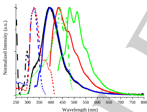
Figure 5. Normalized excitation (dotted lines) and emission (solid lines) spectra of 2CI crystals at 298 K. Emission: \lambda_{exc} = 280 nm (black), \lambda_{exc} = 308 nm (blue), \lambda_{exc} = 375 nm (red) and \lambda_{exc} = 413 nm (green). Excitation: \lambda_{em} = 328 nm (black), \lambda_{em} = 398 nm (blue), \lambda_{em} = 436 nm (red) and \lambda_{em} = 514 nm (green).
