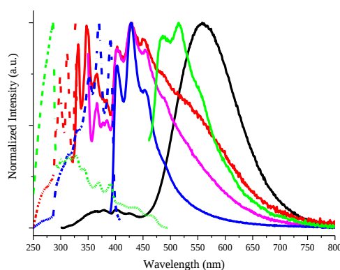
Figure 4. Normalized excitation (dotted lines) and emission (solid lines) spectra of 1CI crystals at 77 K. Emission: \lambda_{exc} = 280 nm (black), \lambda_{exc} = 300 nm (red), \lambda_{exc} = 327 nm (magenta), \lambda_{exc} = 370 nm (blue) and \lambda_{exc} = 440 nm (green). Excitation: \lambda_{em} = 348 nm (red), \lambda_{em} = 428 nm (blue) and \lambda_{em} = 515 nm (green).
