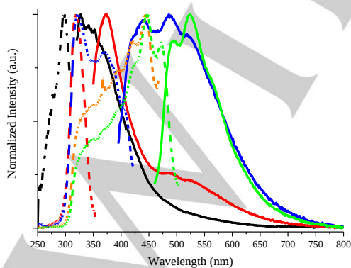
Figure 8. Normalized excitation (dotted lines) and emission (solid lines) spectra of 3CI crystals at 298 K. Emission: \lambda_{\text{exc}}=300 nm (black), \lambda_{\text{exc}}=330 nm (red), \lambda_{\text{exc}}=374 nm (blue) and \lambda_{\text{exc}}=440 nm (green). Excitation: \lambda_{\text{em}}=327 nm (black),
