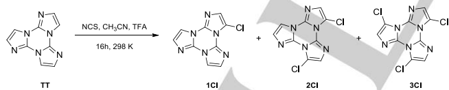
Scheme 1. Synthesis of chloro- TT derivatives.
