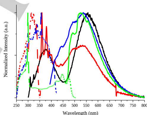
Figure 9. Normalized excitation (dotted lines) and emission (solid lines) spectra of 3CI crystals at 77 K. Emission: \lambda_{\text{exc}}=280 nm (black), \lambda_{\text{exc}}=330 nm (red), \lambda_{\text{exc}}=373 nm (blue) and \lambda_{\text{exc}}=440 nm (green). Excitation: \lambda_{\text{em}}=373 nm (red), \lambda_{\text{em}}=443 nm (blue) and \lambda_{\text{em}}=526 nm (green).
