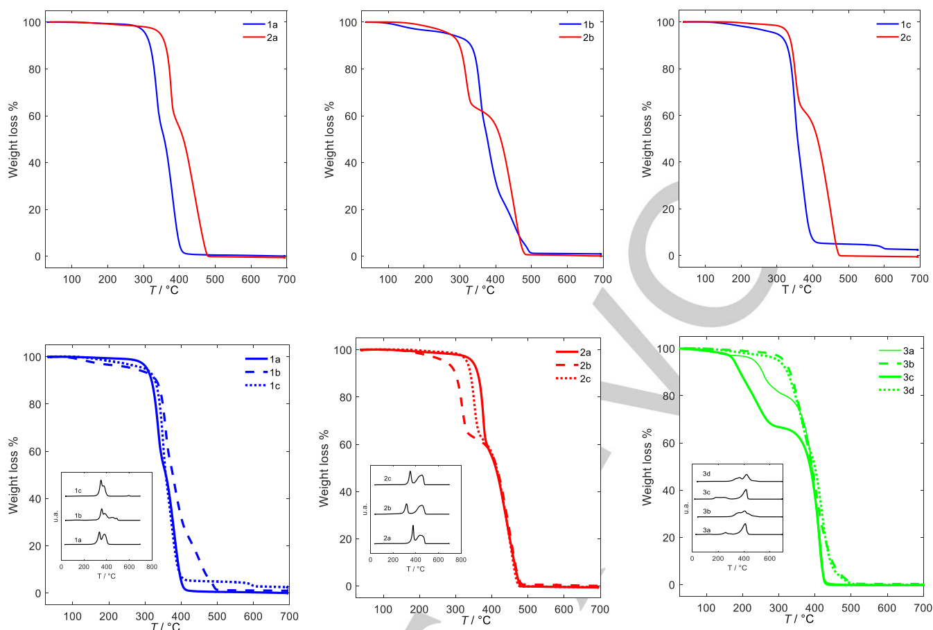
Figure 2. Comparing TGA features of CILs with chiral cations 1a-c (blue curves) and 2a-c (red curves), as well as of CILs with chiral anions 3a-d (green curves); insets provide a comparison of the curve derivatives
