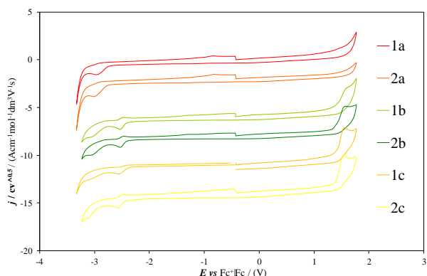
Figure 3a. A synopsis of CV features of the six CILs with chiral cations, recorded at 0.2 \text{ V s}^{-1} scan rate, in 0.00075 \text{ mol dm}^{-3} solutions in ACN + TBAPF 6 0.1 \text{ mol dm}^{-3} . Potentials have been normalized vs the formal potential of the intersolvental ferricinium|ferrocene ( \text{Fc}^+|\text{Fc} ) reference redox couple, recorded in the same conditions.
