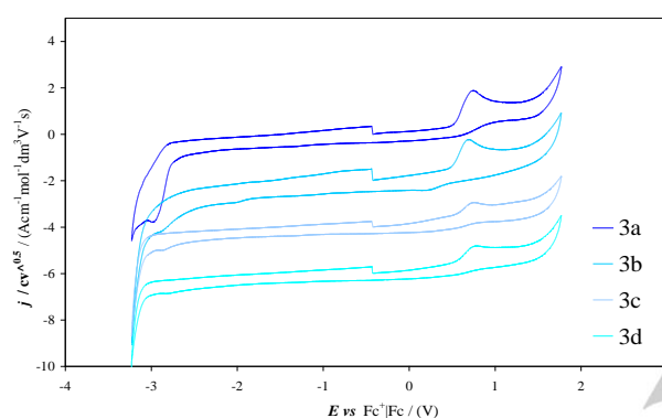
Figure 3b. A synopsis of CV features of four CILs with chiral anions, recorded at 0.2 \text{ V s}^{-1} scan rate, in 0.00075 \text{ mol dm}^{-3} solutions in ACN + TBAPF 6 0.1 \text{ mol dm}^{-3} . Potentials have been normalized vs the formal potential of the intersolvental ferricinium|ferrocene ( \text{Fc}^+|\text{Fc} ) reference redox couple, recorded in the same conditions.
