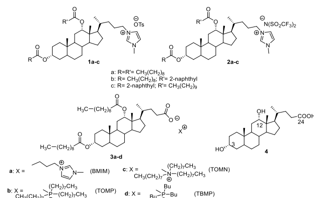
Figure 1. Structure of the synthesised CILs (1-3) and deoxycholic acid (4).
