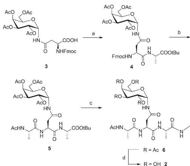
Scheme 1 Synthesis of the model glycopeptide Ac-Ala-Asn-( \alpha -N-Gal)-Ala-NHMe 2 . Reagents and conditions: (a) 1. H-Ala- O tBu-HCl, PyBROP, i\text{Pr}_2\text{NEt} , \text{CH}_2\text{Cl}_2 , 0 °C to room temperature, 83%; (b) 1. octanethiol, cat. DBU, THF; 2. Ac-Ala-OH, HATU, i\text{Pr}_2\text{NEt} , DMF, 65% over two steps; (c) 1. TFA, \text{CH}_2\text{Cl}_2 ; 2. \text{NH}_2\text{Me}\cdot\text{HCl} , PyBROP, i\text{Pr}_2\text{NEt} , DMF, 54%; (d) cat. \text{K}_2\text{CO}_3 , MeOH, 85%.
