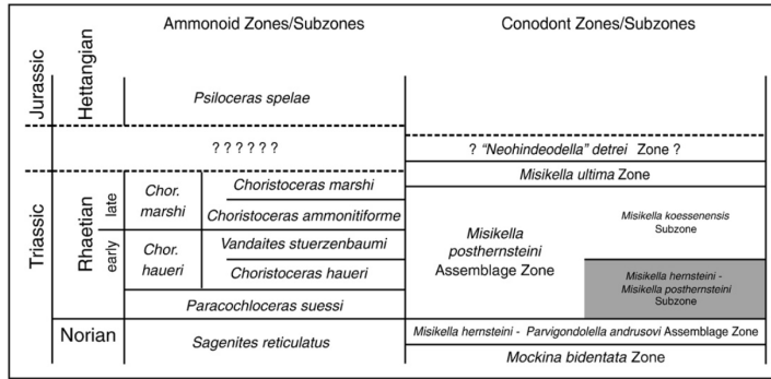
Fig. 5. Late Norian–Hettangian ammonoid and conodont zonation (after Krystyn, 1987; 1990; Kozur and Mock, 1991). The conodont zonation proposed by Kozur and Mock (1991) has been here modified by attributing an early Jurassic age to the Neohindeodella detrei Zone (after Pálfy et al., 2007). The upper part of the Zu1 member belongs to the conodont Misikella hermssteini – Misikella posthermsteini Subzone (lower Rhaetian), marked by the grey area. Ammonoid and conodont zonations are not on a linear time axis.
