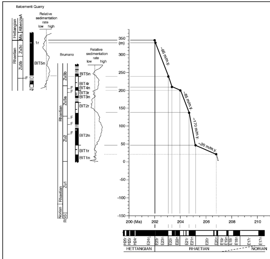
Fig. 12. Age model of sedimentation at Brumano and Italcementi Quarry obtained by means of correlation to the Newark APTS. Relative sedimentation rate curves are described in caption to Fig. 11 and in the text. Ma. is Malanotte Formation; RSS is Riva di Solto Shale.
