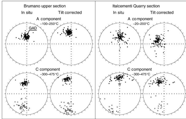
Fig. 9. Equal-area projections before ( in situ ) and after bedding tilt correction of the A and characteristic C component directions from Brumano and Italcementi Quarry (see Table 1). Closed symbols are projections onto the lower hemisphere and open symbols onto the upper hemisphere.
