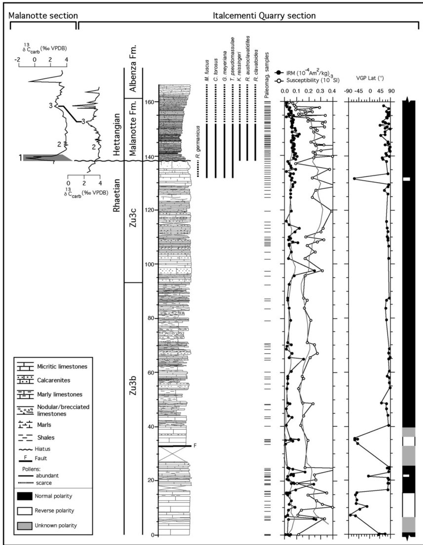
Fig. 4. Italcementi Quarry section. From left to the right: lithology subdivisions, ranges of palynomorph taxa and biostratigraphic age attribution, stratigraphic positions of paleomagnetic samples, natural remanent magnetization (NRM) and isothermal remanent magnetization (IRM), latitude of the sample VGP relative to the north pole of the mean paleomagnetic axis, with magnetic polarity zones shown by filled (open) bars for normal (reverse) polarity. Panels on the upper left side are the carbon isotope profiles from Italcementi Quarry and the nearby Malanotte section across the Triassic-Jurassic boundary (Galli et al., 2005; 2007). See text for discussion.
