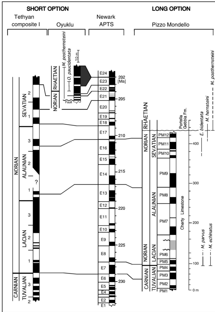
Fig. 1. Short duration vs. long duration options for the Rhaetian, the youngest stage of the Triassic. According to the compilation of magneto-biostratigraphic data from the Tethyan realm of Krystyn et al. (2002) and Gallet et al. (2003) (Tethyan composite I), and recent data from Oyuklu (Gallet et al., 2007), the Rhaetian is ~2 Myr in duration and in part missing in a supposed gap in the Newark APTS (Kent and Olsen, 1999). According to data from Pizzo Mondello (Muttoni et al., 2004), the Rhaetian should be ~6-7 Myr long, virtually similar in duration to the original estimate of Kent and Olsen (1999). The Triassic-Jurassic boundary in Newark section based on palynofloral evidence occurs near the base of E24n. See text for discussion.
