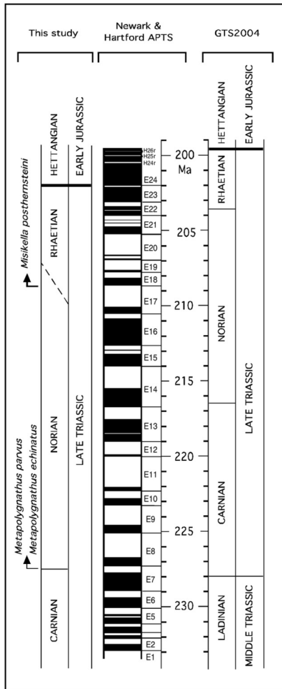
Fig. 13. The Triassic chronostratigraphy from this study compared to the Newark and Hartford basin astronomical polarity time scale (APTS) and the recent Triassic time scale of Gradstein et al. (2004). See text for discussion.
