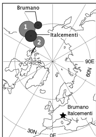
Fig. 10. Paleomagnetic poles calculated from the characteristic C component at Brumano and Italcementi Quarry (Table 1) compared to the Triassic paleomagnetic poles of NW Africa-Adria (Muttoni et al., 2001a; Table 3; entry #1: Middle-early Late Triassic; #2: Late Triassic-Early Jurassic). Equal-area projection was made with PaleoMac (Cogné, 2003). See text for discussion.
