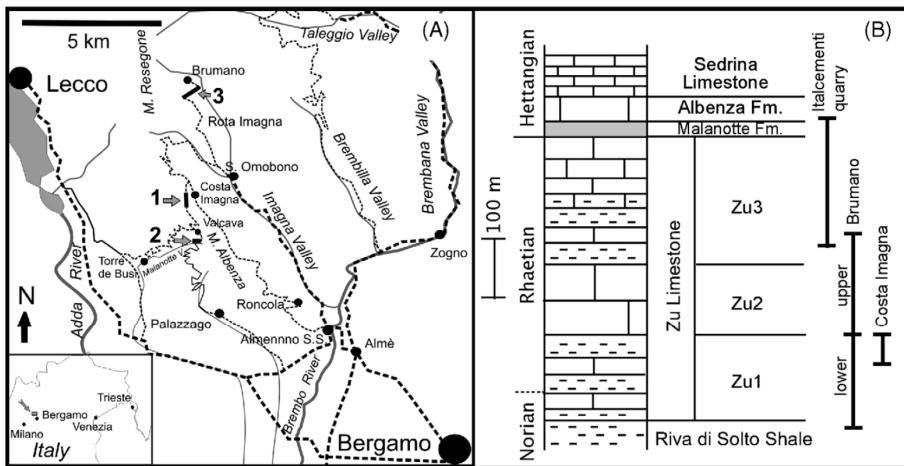
Fig. 2. (A) Location map of the sampling area with indication of sampling sections (1 = Costa Imagna; 2 = Italcementi Quarry and Malanotte; 3 = Brumano lower and upper sections). (B) Stratigraphy of the sampled interval with indication of stratigraphic coverage of individual sections.
