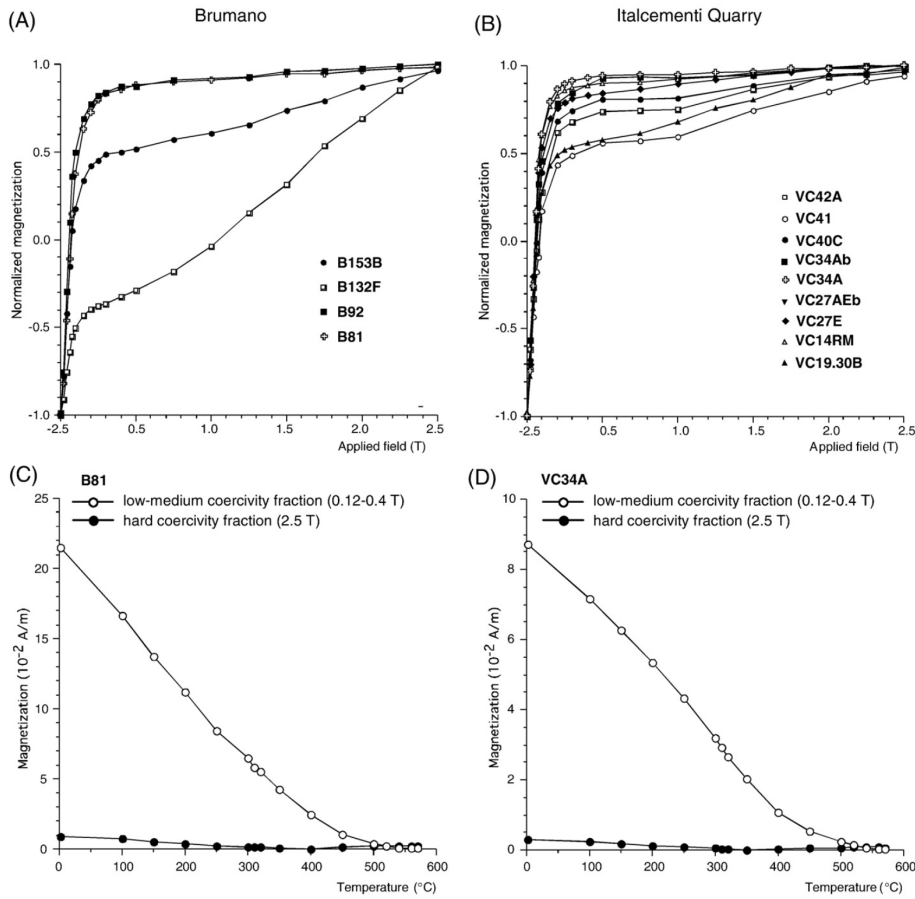
Fig. 7. Basic rock-magnetic properties using isothermal remanent magnetization (IRM) acquisition curves for Brumano (A) and Italcementi Quarry (B) samples. Thermal decay of 3-component IRM for a representative sample from Brumano (C) and Italcementi Quarry (D) indicating that samples have a dominant magnetite phase.
