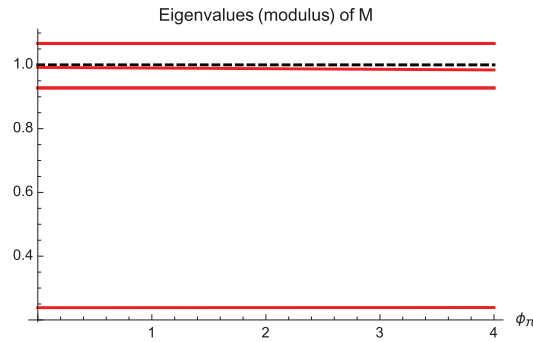
Fig. 7. Determinacy depending on \Phi_\pi . Notes: \beta = 0.99 , \sigma = 0.157 , \kappa = 0.001 , \Phi_y = 0.5 , \gamma = 1 , N = 3 .
