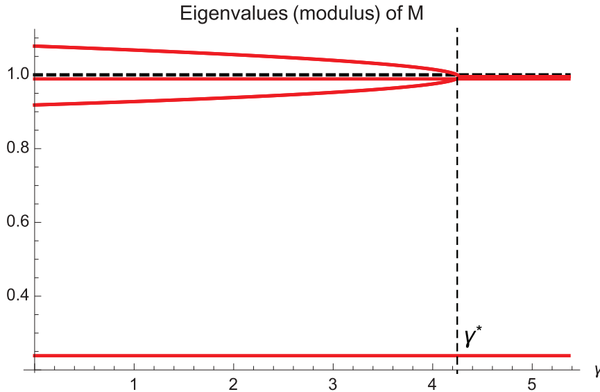
Fig. 3. Determinacy depending on \gamma . Notes: \beta = 0.99 , \sigma = 0.157 , \kappa = 0.001 , \Phi_\pi = 1.5 , \Phi_y = 0.5 , N = 3 . Parameter \gamma is a convolution of the currency union's structural parameter \sigma and the index of openness \alpha \in [0, 1] . The range of \gamma is thus obtained by letting \alpha vary between 0 and 1.
