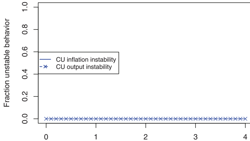
Fig. 6. Instability in the artificial fixed exchange rate regime in dependence of monetary policy parameter \Phi_\pi for unstable \gamma . Notes: \sigma = 0.157 , \kappa = 0.001 , \beta = 0.99 , \gamma = 1 , \Phi_y = 0.5 , sd=0.1 , N = 3 .
