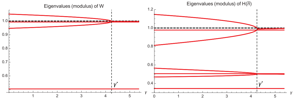
Fig. 1. Instability depending on \gamma . Notes: \beta = 0.99 , \sigma = 0.157 , \kappa = 0.001 , \Phi_\pi = 1.5 , \Phi_\gamma = 0.5 , N = 3 . Parameter \gamma is a convolution of the currency union's structural parameter \sigma and the index of openness \alpha \in [0, 1] . The range of \gamma is thus obtained by letting \alpha vary between 0 and 1.
