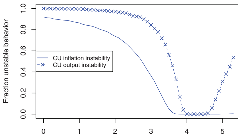
Fig. 2. Instability Depending on \gamma . Notes: \sigma = 0.157 , \kappa = 0.001 , \beta = 0.99 , \Phi_\pi = 1.5 , \Phi_y = 0.5 , sd=0.1 , N = 3 . Parameter \gamma is a convolution of the currency union's structural parameter \sigma and the index of openness \alpha \in [0, 1] . The range of \gamma is thus obtained by letting \alpha vary between 0 and 1.
