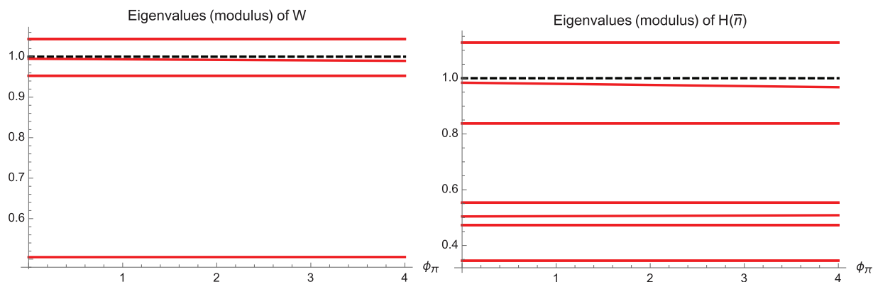
Fig. 4. Instability depending on \Phi_\pi for unstable \gamma . Notes: \beta = 0.99 , \sigma = 0.157 , \kappa = 0.001 , \Phi_y = 0.5 , \gamma = 1 , N = 3 .
