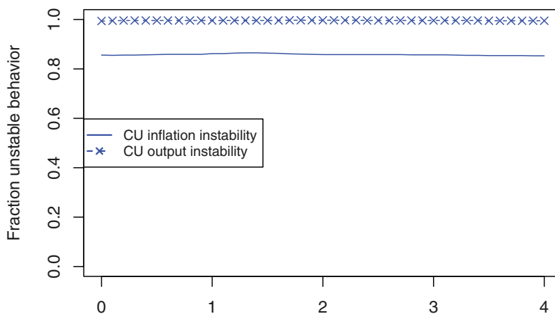
Fig. 5. Instability depending on \Phi_\pi for unstable \gamma . Notes: \sigma = 0.157 , \kappa = 0.001 , \beta = 0.99 , \gamma = 1 , \Phi_y = 0.5 , sd=0.1 , N = 3 .
