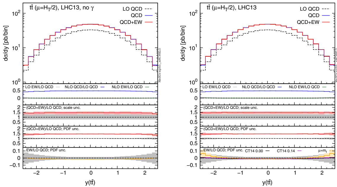
Fig. 8 Differential distributions for the \gamma(t\bar{t}) at 13 TeV. The format of the plots is described in detail in the text
