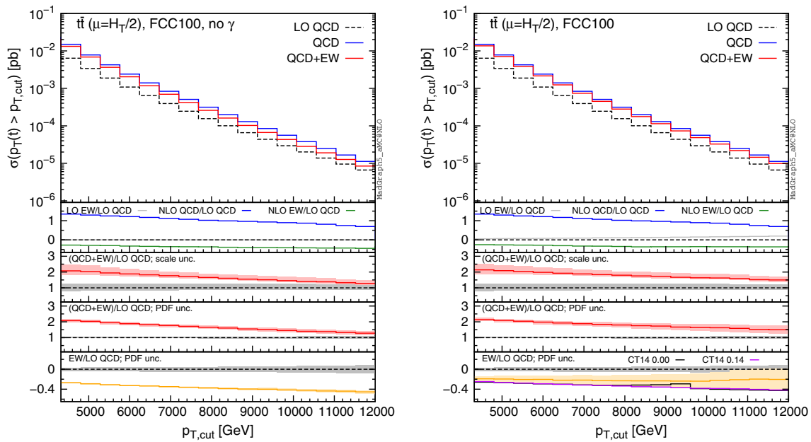
Fig. 14 Integrated distributions for the p_T(t) at 100 TeV. The format of the plots is described in detail in the text
