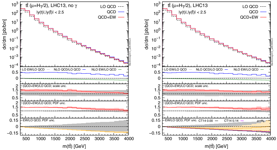
Fig. 6 Differential distributions for the m(t\bar{t}) at 13 TeV with |y(t)|, |y(\bar{t})| < 2.5 cuts applied. The format of the plots is described in detail in the text
