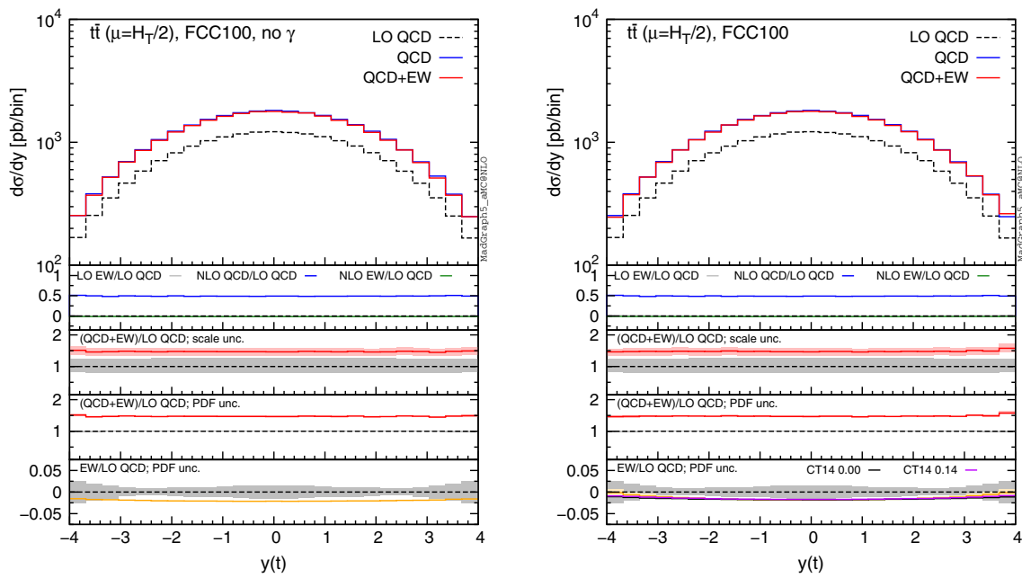
Fig. 12 Differential distributions for the y(t) at 100 TeV. The format of the plots is described in detail in the text
