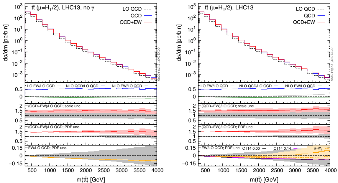
Fig. 5 Differential distributions for the m(t\bar{t}) at 13 TeV. The format of the plots is described in detail in the text
