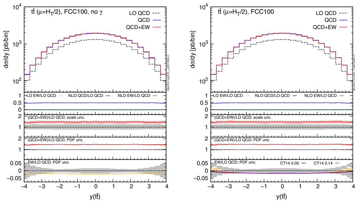
Fig. 13 Differential distributions for the y(t\bar{t}) at 100 TeV. The format of the plots is described in detail in the text
