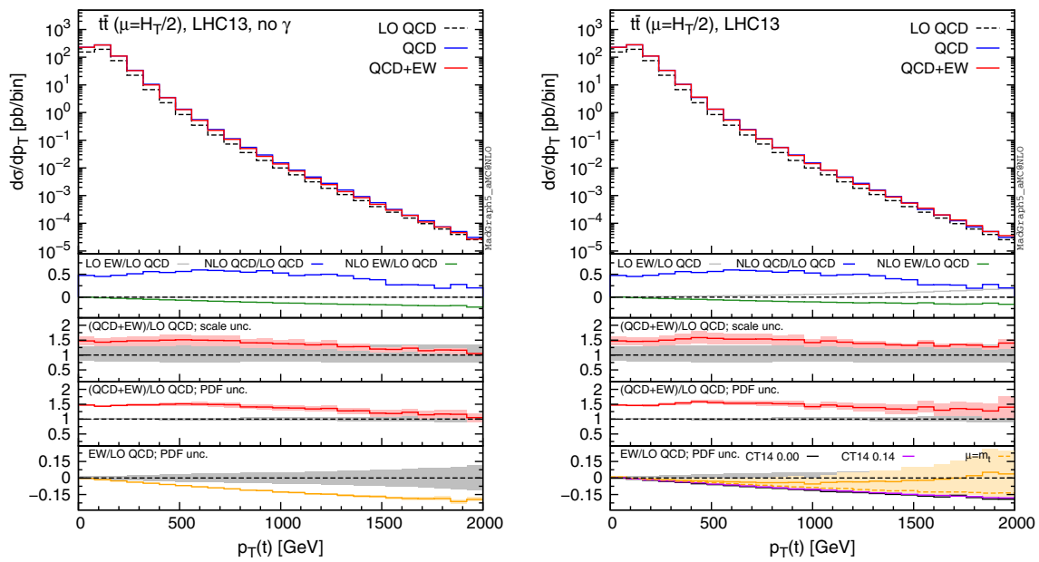
Fig. 4 Differential distributions for the p_T(t) at 13 TeV. The format of the plots is described in detail in the text
