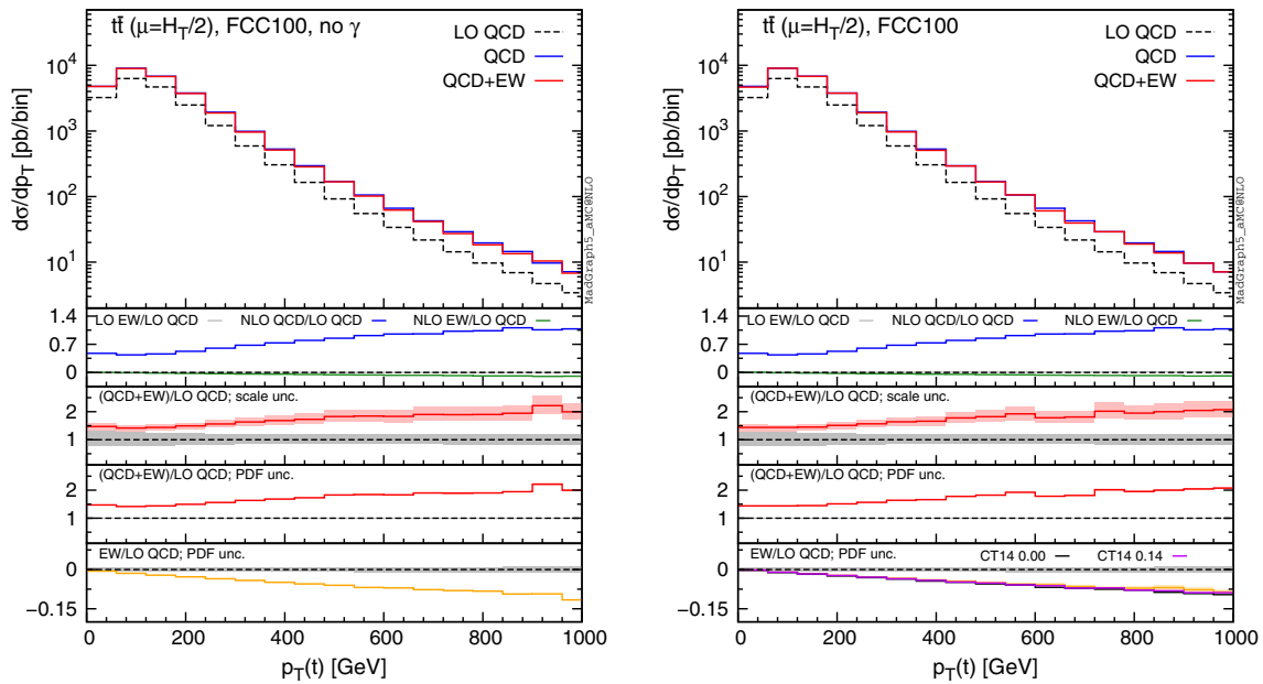
Fig. 10 Differential distributions for the p_T(t) at 100 TeV. The format of the plots is described in detail in the text
