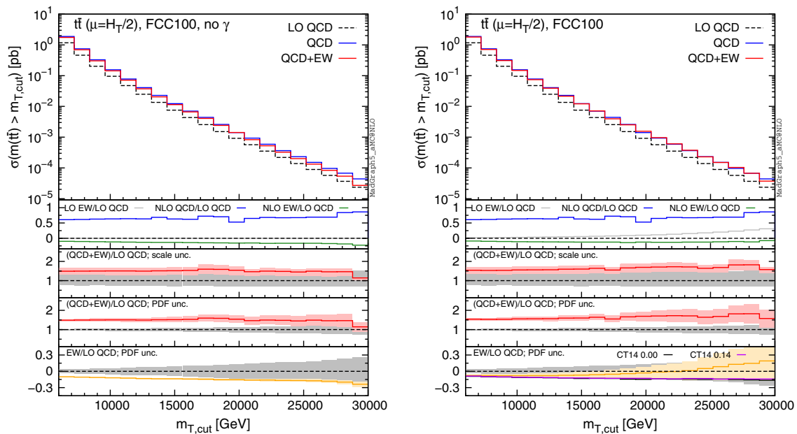
Fig. 15 Integrated distributions for the m(t\bar{t}) at 100 TeV. The format of the plots is described in detail in the text
