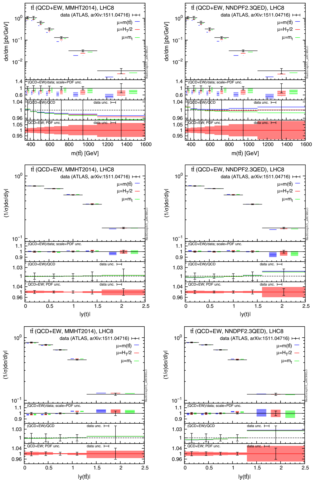
Fig. 17 Comparison of ATLAS data from Ref. [56] and NLO QCD+EW predictions computed with MMHT2104 ( left ) and NNPDF2.3QED ( right ) PDF sets
