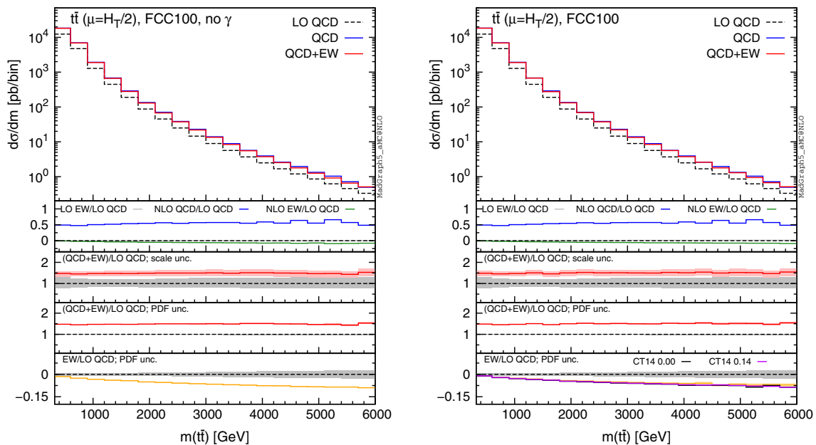
Fig. 11 Differential distributions for the m(t\bar{t}) at 100 TeV. The format of the plots is described in detail in the text
