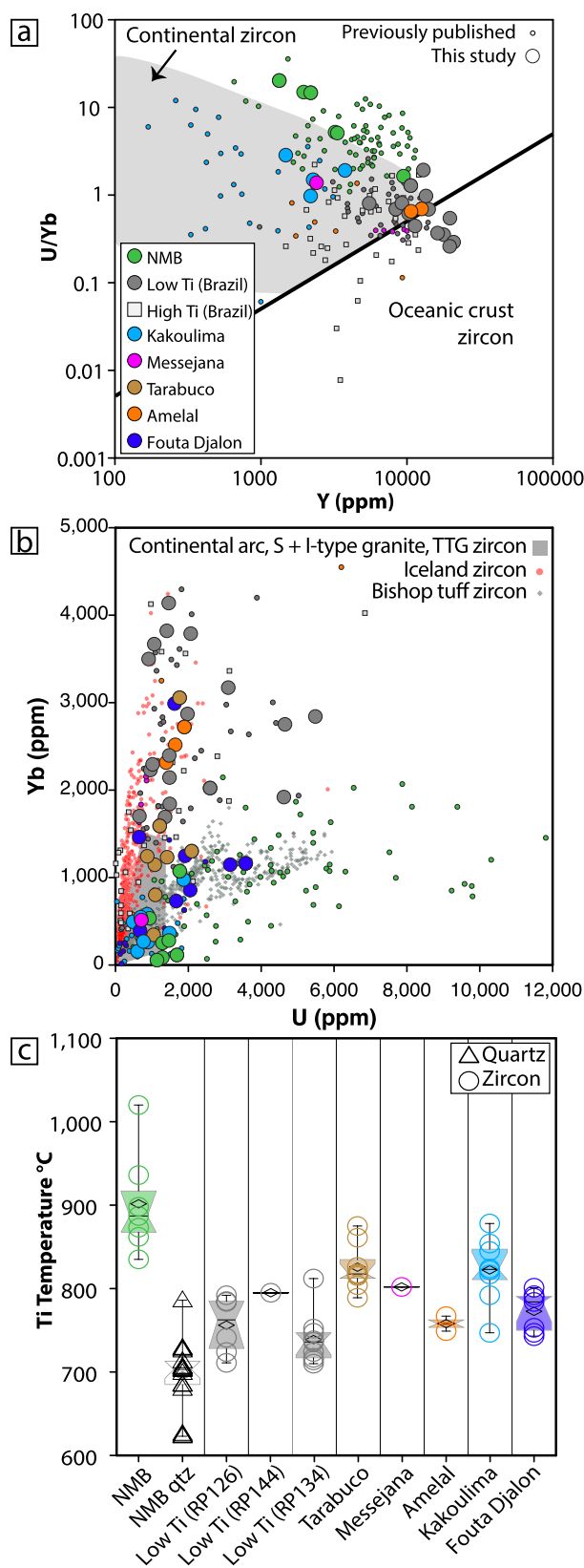
Fig. 5 Trace-element concentrations of CAMP zircon from this study (large symbols) and previously published zircon compositions (small symbols) from (Schoene et al. 2010b; Davies et al. 2017). a Zircon compositions plotted relative to the continental zircon and oceanic zircon fields of (Grimes et al. 2007); note the overlap of CAMP zircon with both fields and also that some analysis lies outside the proposed fields. b CAMP zircon plotted relative to the continental arc zircon, S- and I-type granite zircon, TTG zircon, Icelandic zircon, and zircon from the Bishop Tuff. Compilation of literature zircon data is from (Chamberlain et al. 2014; Carley et al. 2014; Reimink et al. 2020) and references therein. c Box and Whisker plots of Ti temperatures in zircon and quartz for the CAMP samples assuming an Si activity of 1 and a Ti activity of 0.6
