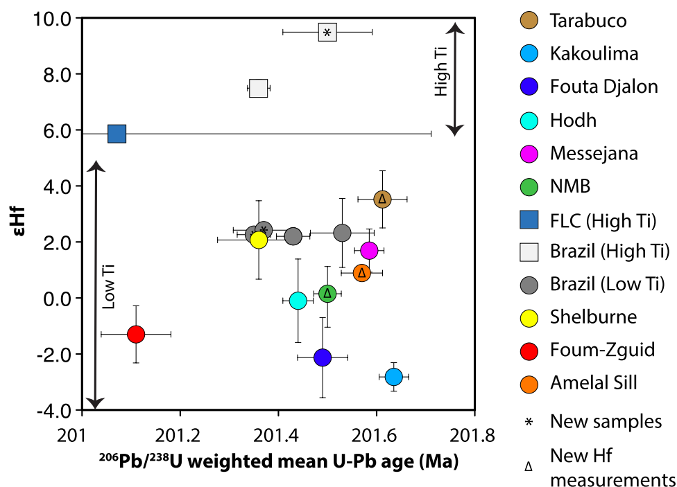
Fig. 3 Age and \epsilon\text{Hf} isotopic compositions of CAMP zircons from this study, and from Davies et al. (2017). Hf isotopic compositions represent average values for the sample with 2\sigma uncertainties. Double-headed arrow (bottom left) shows the range of \epsilon\text{Hf} values from low Ti samples from eastern USA (Elkins et al. 2020), the double-headed arrow (top right) for the high Ti samples is the range suggested for these samples in this study. Asterisks (*) represent the new U–Pb and Hf samples from this study, capital delta symbols ( \Delta ) indicate samples from (Davies et al. 2017) with updated Hf isotopic compositions
