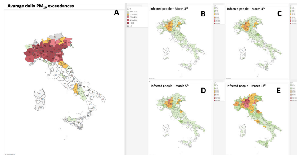
Figure 1 (A) Average daily exceedances of PM_{10} versus number of monitoring stations in different Italian provinces from February 9th to February 29th, 2020. (B–E) Spreading of COVID-19 infections (officially confirmed cases) during the period March 3rd to March 13th, 2020.
