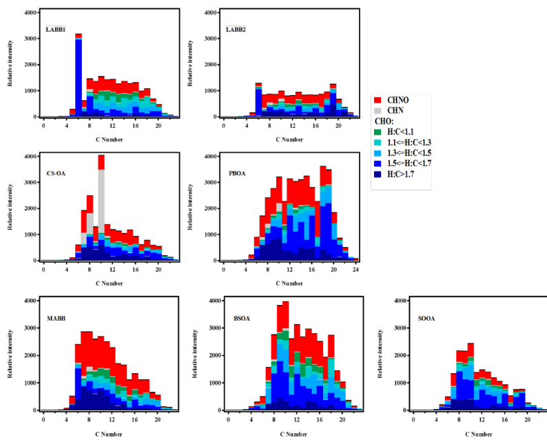
5 Fig. 3 Stacked histogram binned by carbon number of ions, showing the apportioned intensity of each bin to each factor. Colors correspond to 7 families.
