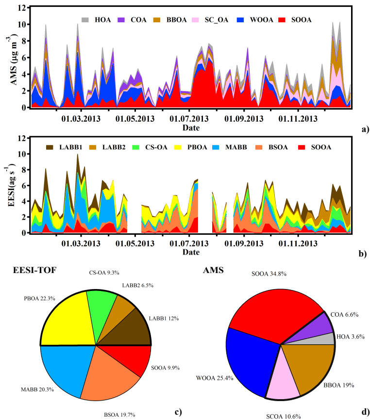
Fig. 10 Comparison between AMS factors and EESI factors: time series of the concentrations AMS PMF factor (a) and mass flux of EESI PMF factor (b). Pie charts of source apportionment results from the EESI (c) and AMS (d).
