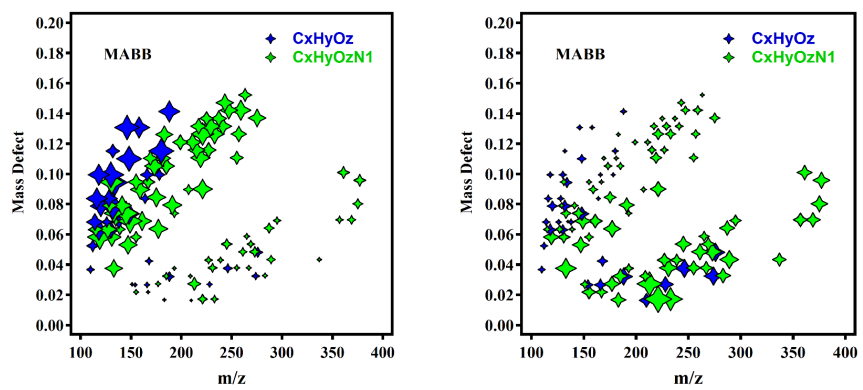
Fig. 7 Mass defect plot of factor-specific ions for the MABB EEST factor colored by nitrogen number, sized by H:C ratio (left) and O:C ratio (right).
