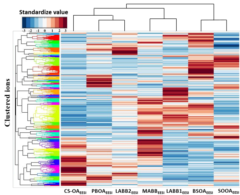
Fig. 4 Standardized matrix of individual EESI-TOF ions vs. EESI-TOF PMF factors, colored by z-score. Ions and factors are sorted according to the results of their respective hierarchical clustering analysis; the resulting dendrograms are shown on the respective axes. The color of the compounds' groups in the dendrogram are chosen to make groupings convenient to read (dendrogram colors are chosen arbitrarily to aid the eye).
