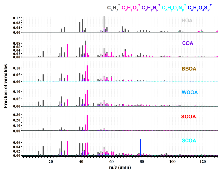
5 Fig.1 Factor profiles for the six-factor solution for AMS results with HOA AMS and COA AMS constrained by a=0.1 . The total signal of each factor is normalized to unity, and the y-axis presents the fractional contributions of the variables to the total signal of the factor. (HOA AMS : Hydrocarbon OA, COA AMS : Cooking-related OA, BPBOA AMS : Biomass burning OA, WOOA AMS : winter oxygenated OA, SOOA AMS : summer oxygenated OA, SCOA AMS : sulfur-containing oxygenated OA).
