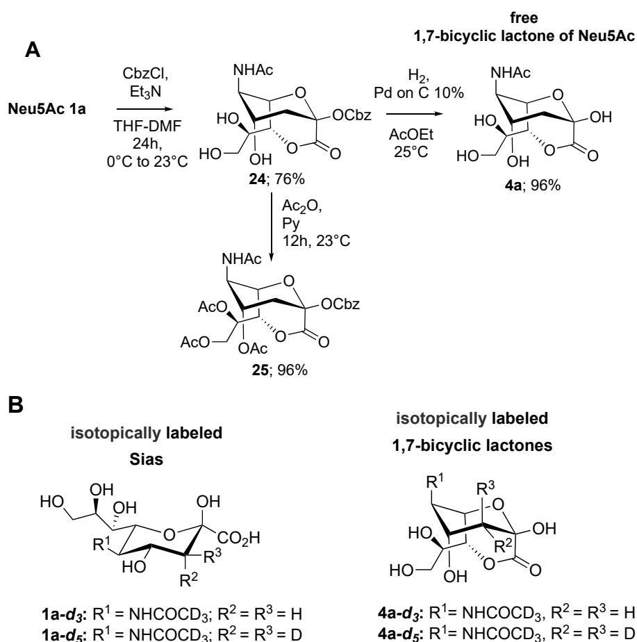
Scheme 6. (A) Synthesis of the free 1,7-bicyclic lactone of Neu5Ac 4a starting from Neu5Ac 1a [17]; (B) isotopically labeled 1,7-bicyclic lactones 4a-d 3 and 4a-d 5 derived from the corresponding Sias 1a-d 3 and 1a-d 5 [18].
