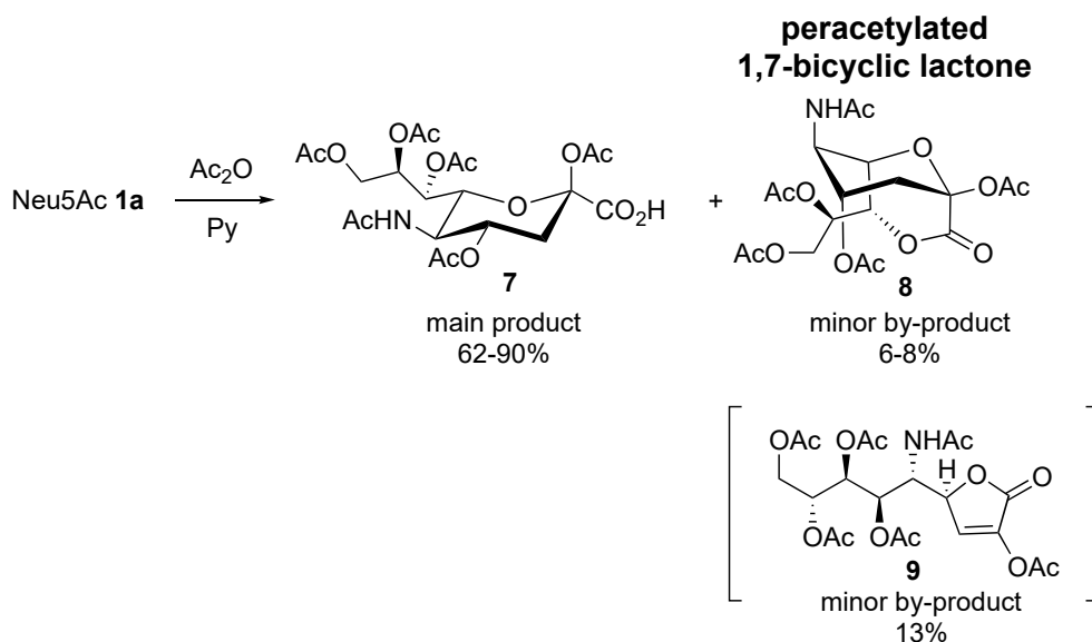
Scheme 2. Synthesis of the peracetylated 1,7-bicyclic lactone 8 as by-product of Neu5Ac 1a classical acetylation [71–73].
