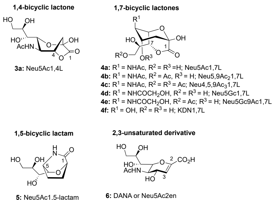
Figure 2. Representation of the 1,4-bicyclic lactone 3a , the six 1,7-bicyclic lactones 4a–f , the 1,5-bicyclic lactame 5 and the 2,3-unsaturated derivative DANA 6 .
