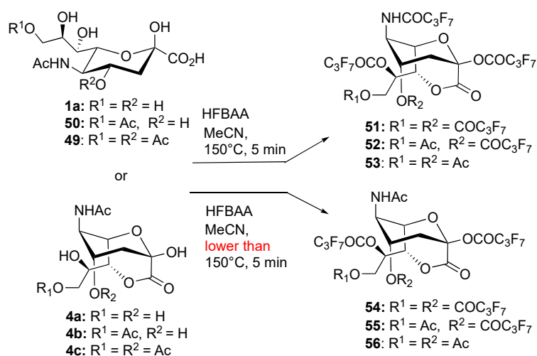
Scheme 18. Derivatization conditions with HFBA explored by Allevi's group [66].
