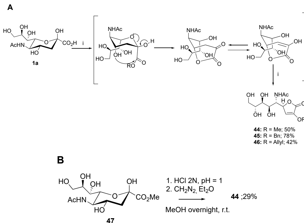
Scheme 11. (A) Synthesis of protected \gamma -lactones 44–46 and the proposed reaction mechanism [89]; (B) alternative synthesis of compound 44 [70].
