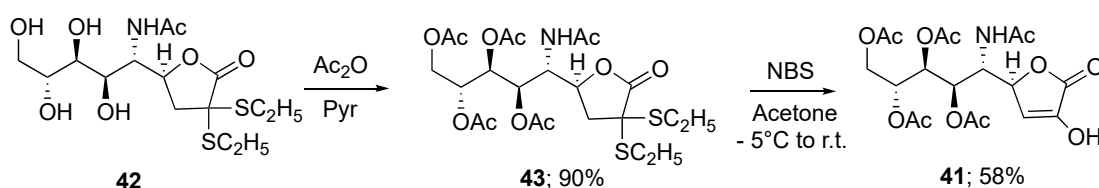
Scheme 10. Synthesis of protected \gamma -lactone 41 [88].
