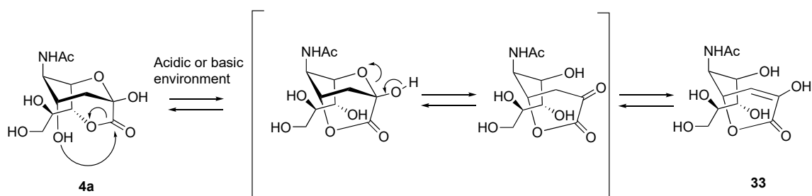
Scheme 13. Synthesis of the free \gamma -lactone 33 starting from the bicyclic 1,7-lactone 4a [78].
