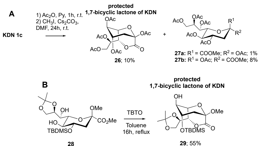
Scheme 7. (A) Synthesis of the peracetylated 1,7-bicyclic lactone of KDN 26 [79]; (B) synthesis of the protected 1,7-bicyclic lactone of KDN 29 [80].
