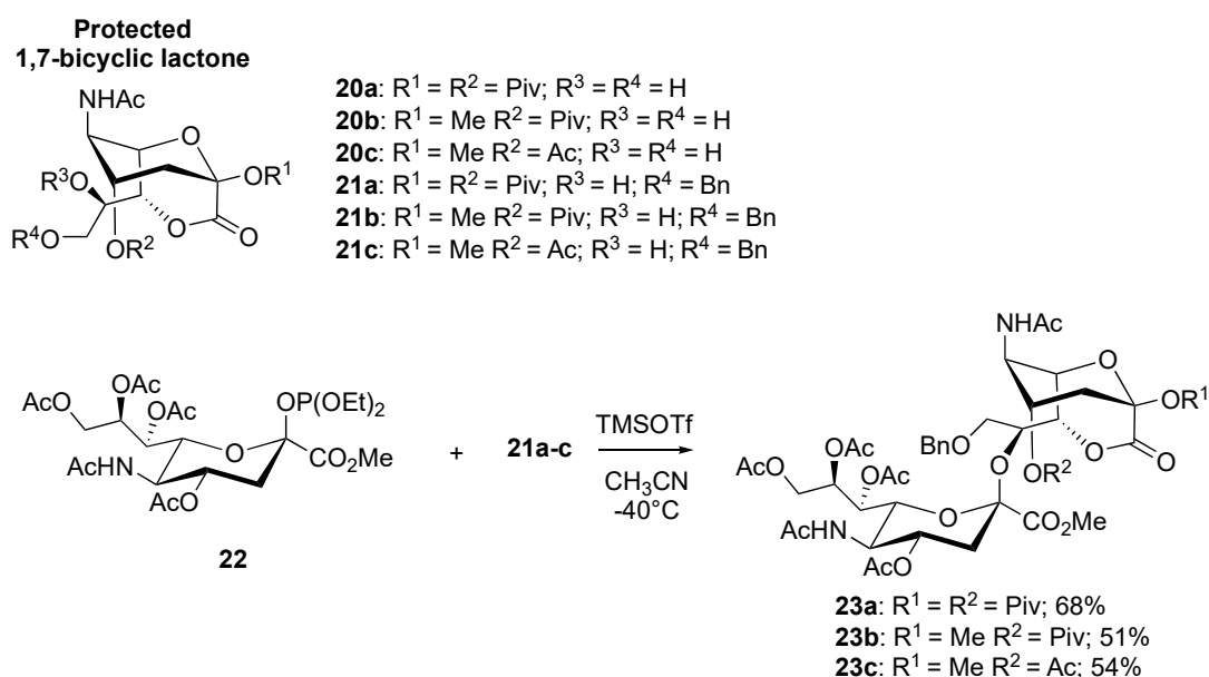
Scheme 5. Protected 1,7-bicyclic lactones 20a–c and 21a–c and synthesis of the \beta -2,8-unnatural saccharides 23a–c [75].
