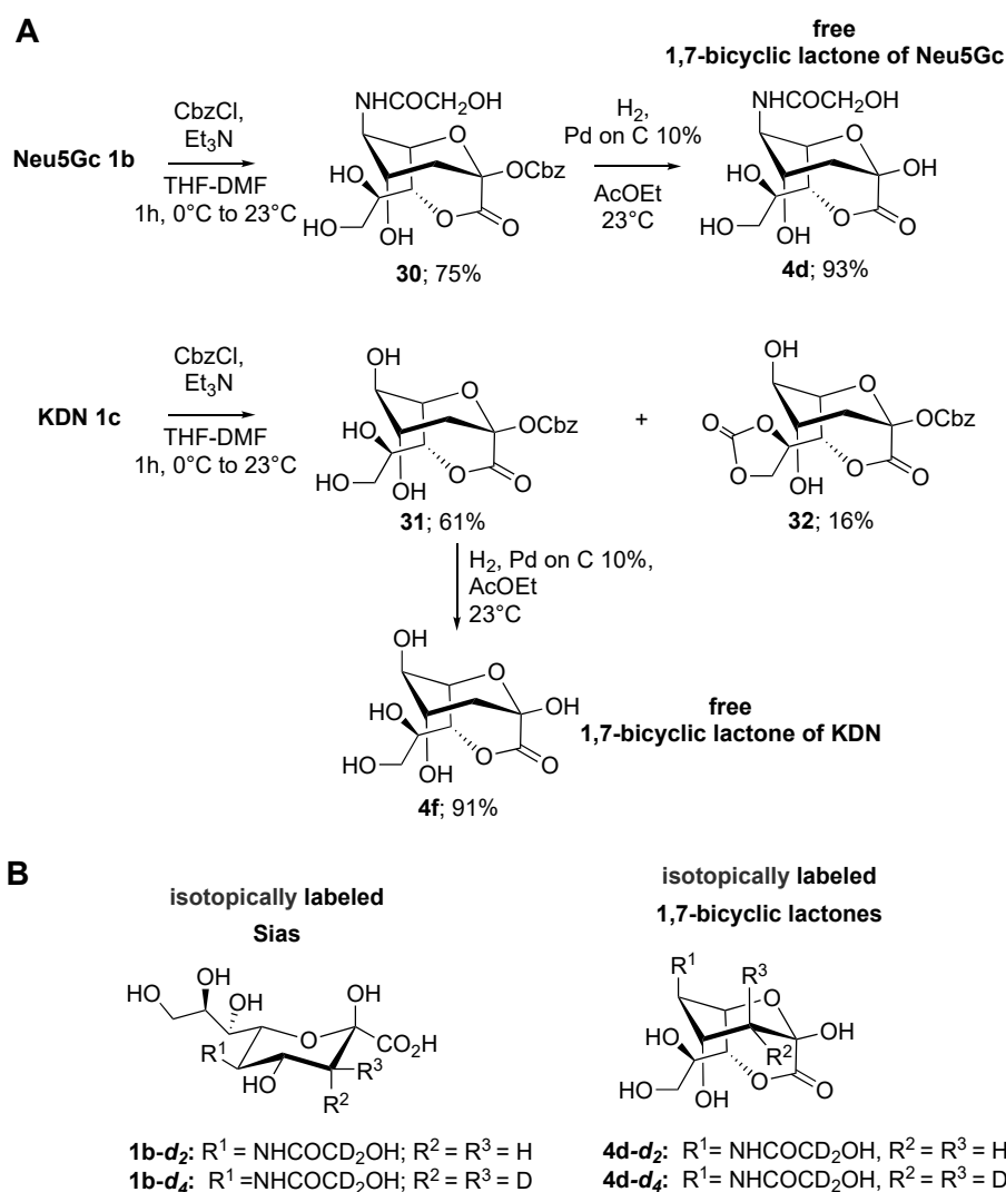
Scheme 8. (A) Synthesis of the free 1,7-bicyclic lactone of Neu5Gc 4d and of KDN 4f , starting from Neu5Gc 1b and KDN 1c , respectively [19]; (B) isotopically labeled 1,7-bicyclic lactones 4d-d 2 and 4d-d 4 derived from the corresponding Sias 1b-d 2 and 1b-d 4 [18].
