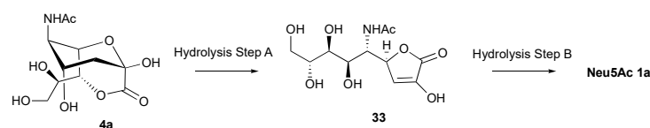
Scheme 16. General two-steps hydrolysis of compound 4a (see Table 1 for reaction conditions) [78].
