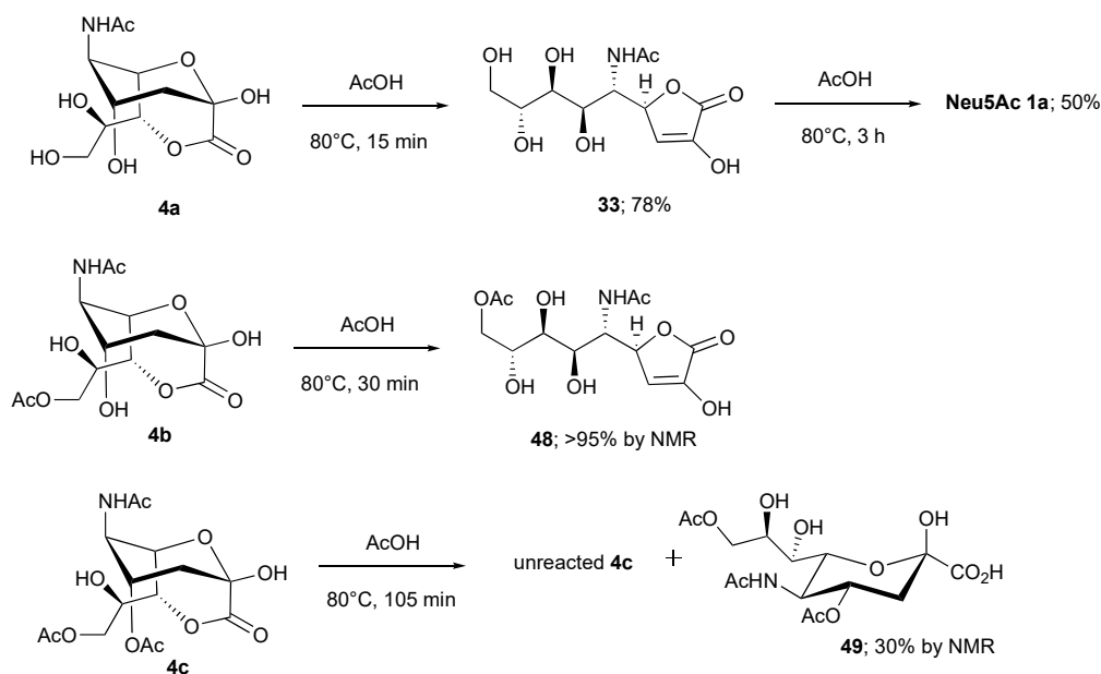
Scheme 17. Reactivity of 1,7-lactones 4a , 4b and 4c under acidic conditions (AcOH, 80 °C) [78].
