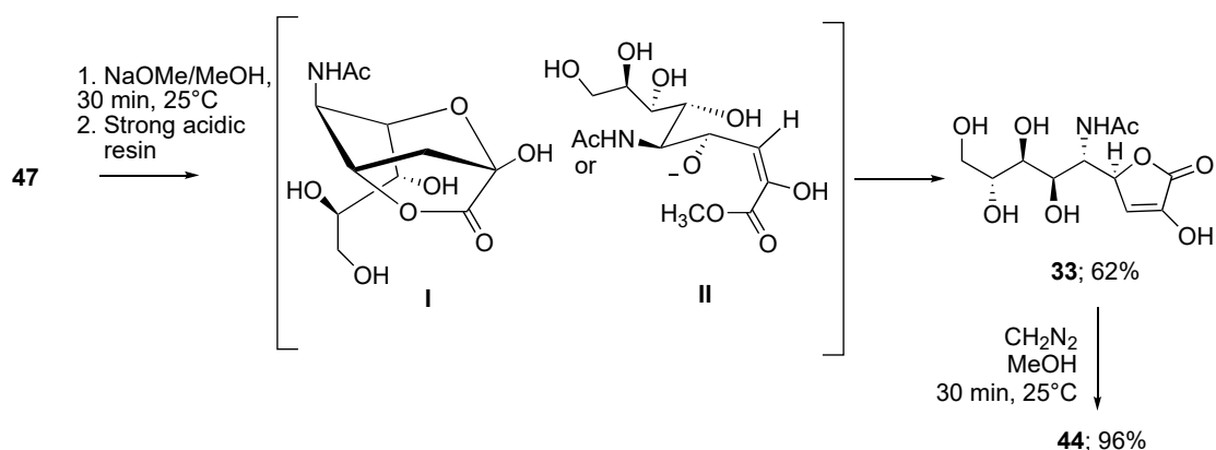
Scheme 12. Synthesis of the free \gamma -lactone 33 starting from the methyl ester 47 [85].
