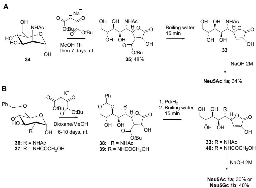
Scheme 9. (A) Synthesis of Neu5Ac 1a starting from N -acetylmannosamine 34 [83]; (B) synthesis of Neu5Ac 1a and Neu5Gc 1b starting from the protected compounds 36 and 37 , respectively [83,84].
