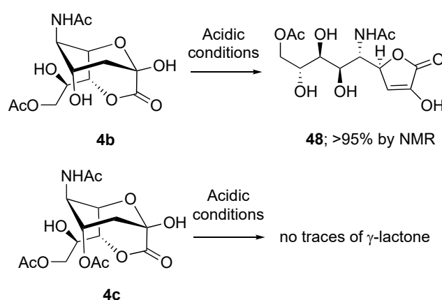
Scheme 14. Synthesis of the protected \gamma -lactone 48 starting from the corresponding bicyclic 1,7-lactone 4b [78].
