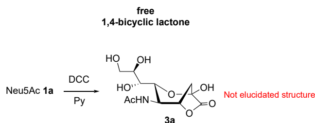
Scheme 1. Synthesis of the free 1,4-bicyclic lactone 3a starting from Neu5Ac 1a [16].
