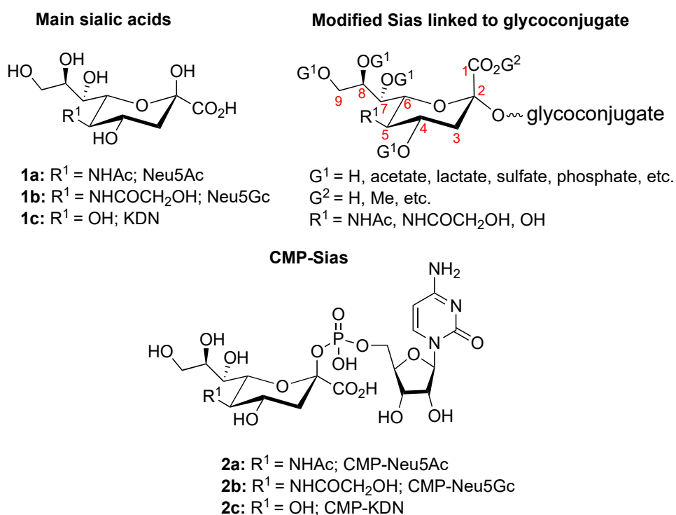
Figure 1. Representation of the three principal sialic acids (Neu5Ac 1a , Neu5Gc 1b , and KDN 1c ), the general structure of modified Sias linked to the glycoconjugate chain, and the three cytidine mononucleotide Sias (CMP)-Sias ( 2a–c ).
