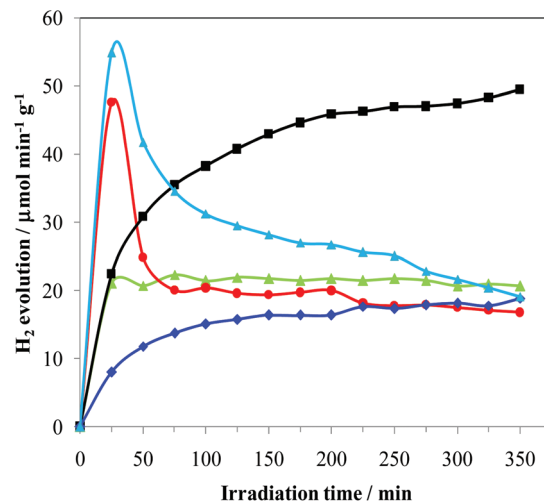
Fig. 1 \text{H}_2 production rates during Pd photo-deposition in methanol aqueous solutions by irradiation in the UV-vis region. ■- Pd(0.5%)-complex- \text{I}_3/\text{TiO}_2 (1); ◆- Pd(0.5%)-complex- \text{BF}_4/\text{TiO}_2 (2); ●- Pd(0.5%)-chloride/ \text{TiO}_2 (3); ▲- Pd(0.5%)-nitrate/ \text{TiO}_2 (4); ▲- Pd(0.5%)-nitrate- \text{I}_2/\text{I}^-/\text{TiO}_2 (5).
