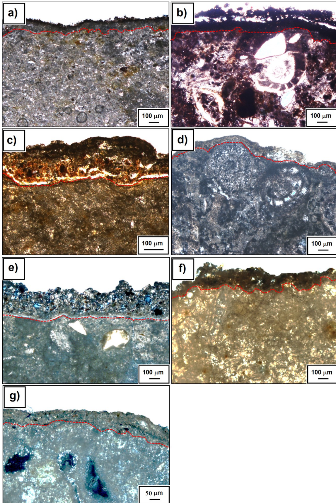
Fig. 2 Microphotographs in OM showing the main textural features of the limestones and the superficial layer associated. The red lines highlight the contact between the two components. A sample and relative image were selected for each study site. a) sample 4, site 1 (Crossed Polarized Light view - CPL). b) sample 5, site 2 (Plane Polarized Light view – PPL). c) sample 10, site 3 (CPL). d) sample 18, site 4 (CPL). e) sample D, site 5 (PPL). f) sample G, site 6 (CPL). g) sample I, site 7 (CPL)
