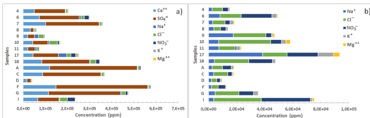
Fig. 3 Ionic concentrations measured in samples: chart a) contains all considered ions, while in chart b) calcium and sulfate ions are excluded
