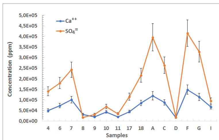
Fig. 4 Concentrations trends in samples of sulfate and calcium ions
