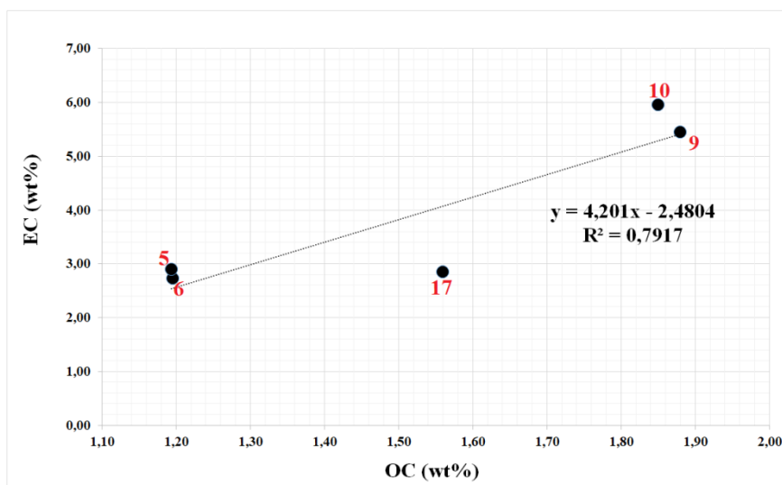
Fig. 7 Scatter plots of OC and EC concentrations for the samples 5,6,9,10, 17 taken at low heights
