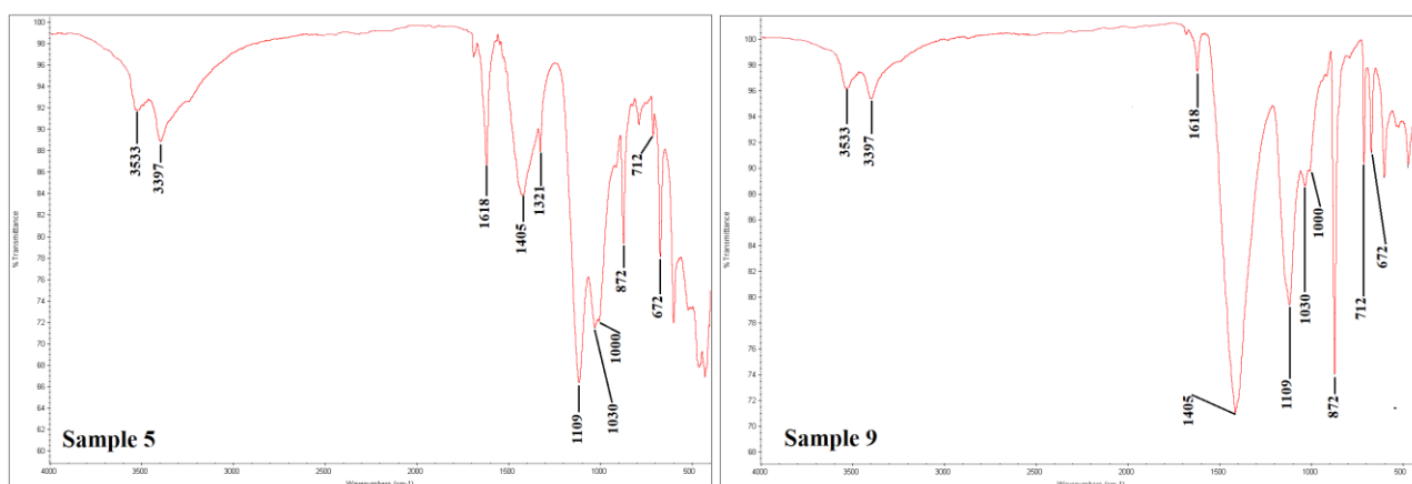
Fig. 5 FT-IR spectra of representative crust of samples 5 and 9
