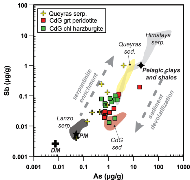
Fig. 9. As ( \mu\text{g/g} ) vs. Sb ( \mu\text{g/g} ) diagram showing the composition of Alpine ultramafic rocks from Queyras (Lafay et al. , 2013) and Cima di Gagnone (CdG; Scambelluri et al. , 2014; Cannà et al. , 2015). The fields of metasediments from the same localities and of oceanic (Lanzo; Debret et al. , 2013b) and wedge serpentinites (Himalaya; Hattori & Guillot, 2003) are shown for comparison. Devolatilization of sedimentary rocks can release these elements (grey arrow starting from oceanic pelagic clays and shale reservoirs; Li, 1991). Interaction of these fluids with serpentinite and meta-peridotite bodies within the Queyras and Cima di Gagnone mélanges leads to element storage in ultramafic rocks (grey arrow departing from the oceanic Lanzo serpentinite). It is important to note that ultramafic rocks from Cima di Gagnone might have partially lost As and Sb during antigorite dehydration. These are therefore minimum levels of enrichment for such rocks. Primitive and depleted mantle (PM and DM) are from McDonough & Sun (1995) and Salters & Stracke (2004).
