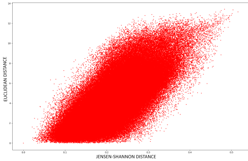
Figure 6: Scatter plot of points representing pairs of rank trajectories: the y-axis reports the Euclidean distance of the embeddings computed with UMAP, the x-axis the Jensen-Shannon distance between symbol distributions
