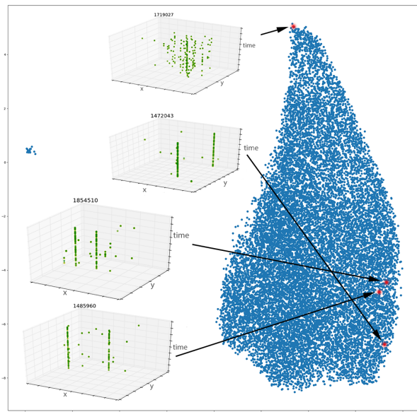
Figure 9: The embeddings corresponding to the four trajectories represented in the spatio-temporal space.
