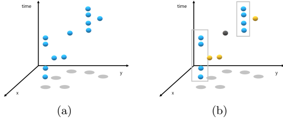
Figure 1: (a) A CDR trajectory with 12 occurrences (in space-time). (b) The rectangles contains two groups of occurrences for the same symbol, i.e. clusters along the temporal line. There are also 3 local noise points (colored in yellow) and one transition point (colored in black) [9].
