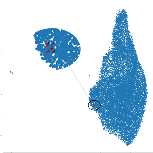
Figure 8: Visual analysis of embeddings: source trajectory (point 0) and the five similar trajectories (points 1 to 5).
