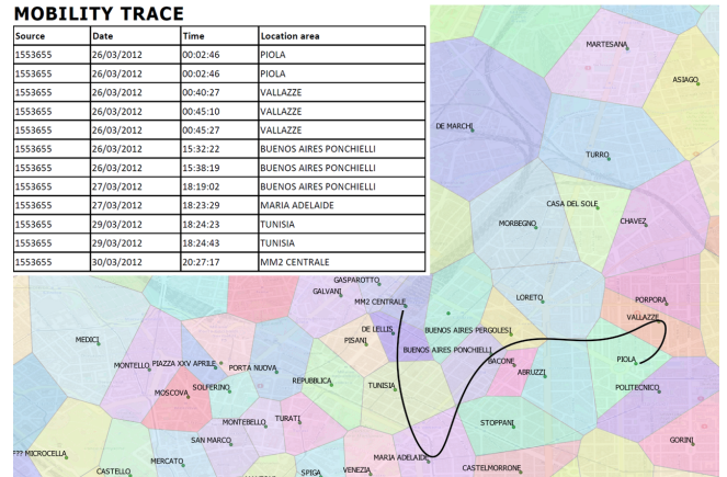
Figure 2: A fragment of CDR trajectory along with the Voronoi diagram approximating the Location Areas.
