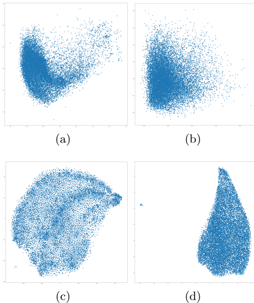
Figure 5: Examples of dimensional reduction of trajectory embeddings: (a) Isometric Mapping; (b) Principal Component Analysis; (c) t-SNE; (d) UMAP. In all non-linear methods (a, c, d) the axes have no specific meaning: any rotation produces an equally valid embedding.
