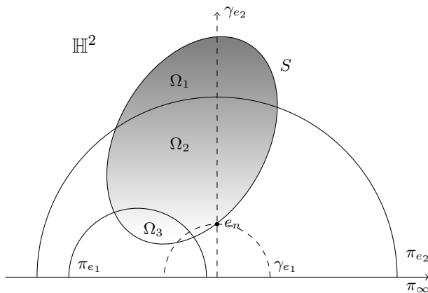
FIGURE 5. A picture of the proof of lemma 6.1 in \mathbb{H}^2 . Here e_j = e_1 and e_i = e_2 .
