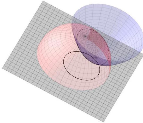
FIGURE 2. In the figure U is the paraboloid in \mathbb{H}^3 parametrized by \chi(u, v) = (v \cos(u), 1/2 - v \sin(u), v^2 + 1/2) and \pi is the half-sphere about the origin of radius one.
