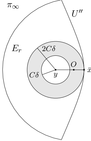
FIGURE 4. Case 3 in the proof of theorem 1.3.
