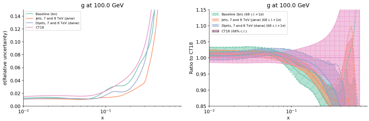
Figure 4.11. Same as Fig. 4.3, but now comparing the baseline ( \#bn ) to the fits with all single-inclusive jet ( \#janw ) and dijet data ( \#danw ) of Fig. 4.10. All results are shown as a ratio to the CT18 fit (also shown for reference).
