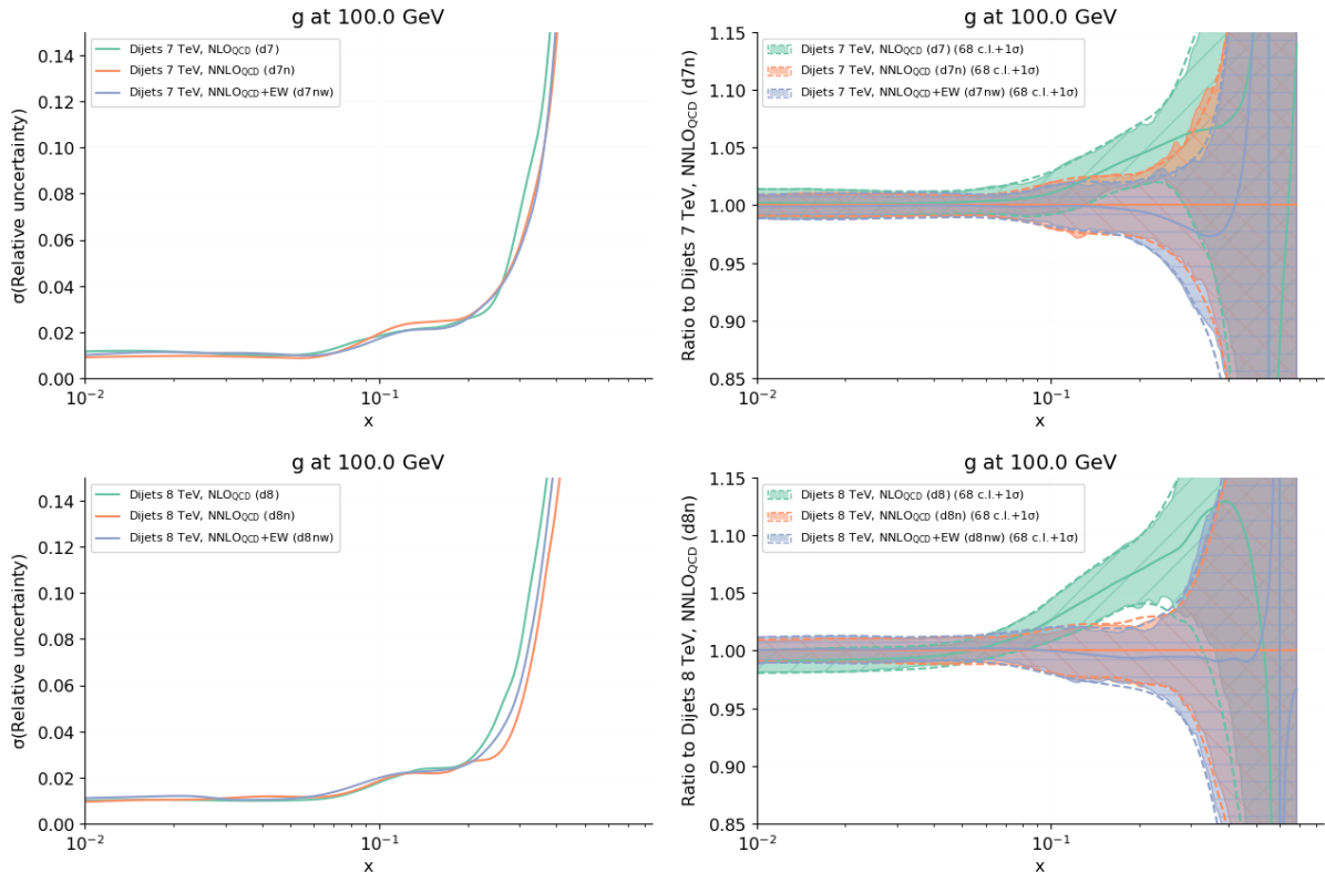
Figure 4.9. Same as Fig. 4.4, but now for dijets.
