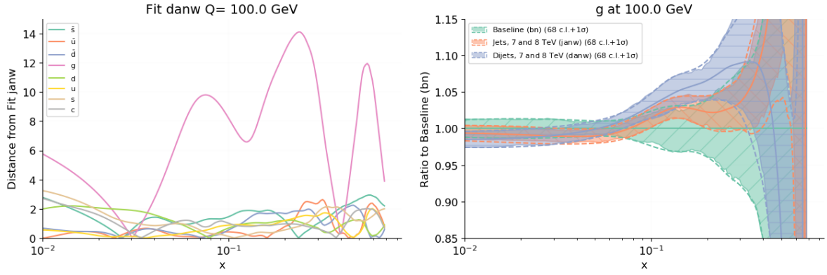
Figure 4.10. Same as Fig. 4.2, but now comparing the fits with all single-inclusive jet data ( \#janw ), and that with all dijet data ( \#danw ) and highest theory accuracy (NNLO QCD+ EW) and default settings. In the gluon comparison (right) results are displayed as a ratio to the baseline with no jet data included (also shown for reference).
