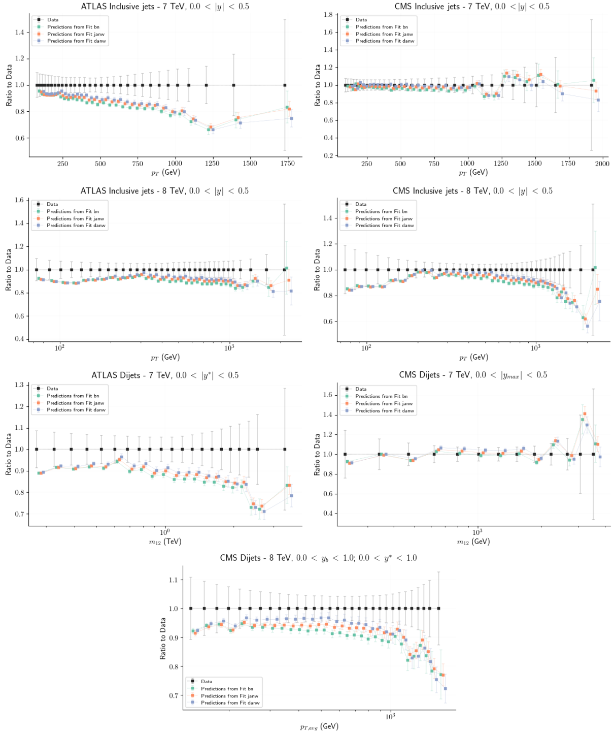
Figure 4.12. The theory to data ratio for a representative set of points from each dataset introduced in Sect. 2. Specifically, we show the central rapidity bins for all the ATLAS and CMS jet and dijet datasets at 7 and 8 TeV. Theoretical predictions are computed from fits #bn, #janw and #danw with corresponding theoretical accuracy.
