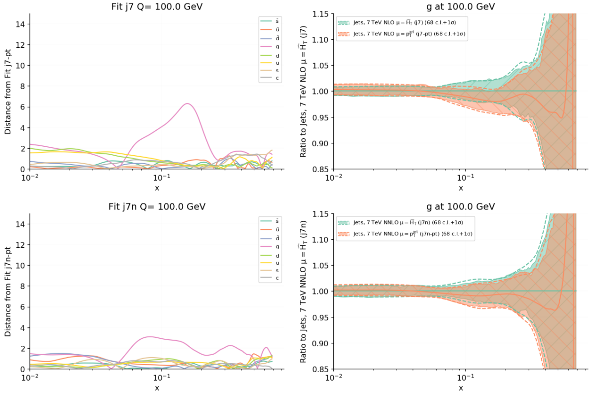
Figure 4.5. Same as Fig. 4.2, but now comparing fits to the 7 TeV data with the choices of central renormalization and factorization scale \mu = \bar{H}_T (as shown in Fig. 4.4, top) and \mu = p_T^{\text{jet}} at NLO (fits #j7 and #j7-pt) and NNLO (fits #j7n and #j7n-pt). The gluon is shown as ratio to the fits with \mu = \bar{H}_T .
