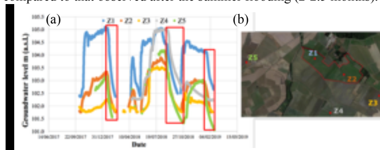
Fig. 2 Groundwater levels (m a.s.l.) monitored in the study area. Colours in (a) correspond to piezometers in (b). Red boxes highlight the groundwater depletion rates after the flooding periods.
