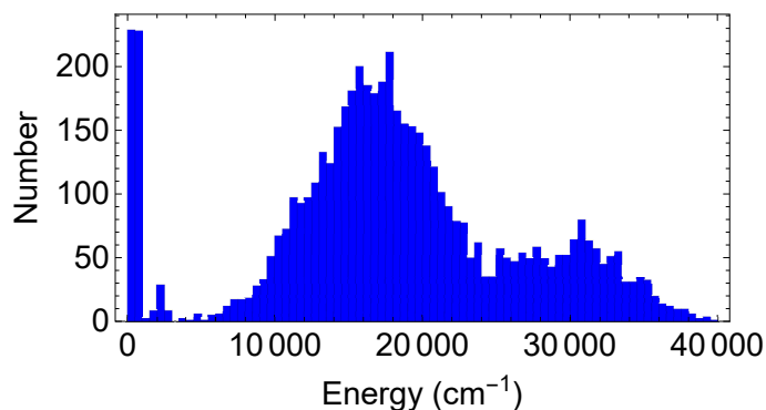
Fig. 2 Histogram of energies for geometries used as the dataset for acetyl-acetone. The bin size for the abscissa is 500 \text{ cm}^{-1} . The database has 5,500 energies and (not shown) 45 \times 5,500 gradient components.
