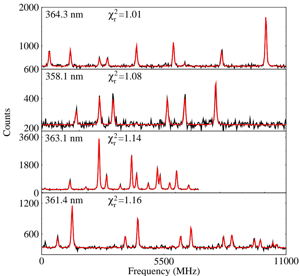
Figure 2. Fitted hyperfine structures of the 364.3 nm, 358.1 nm, 363.1 nm and 361.4 nm lines for the stable ^{45}\text{Sc} isotope investigated during the off-line preparation tests.
