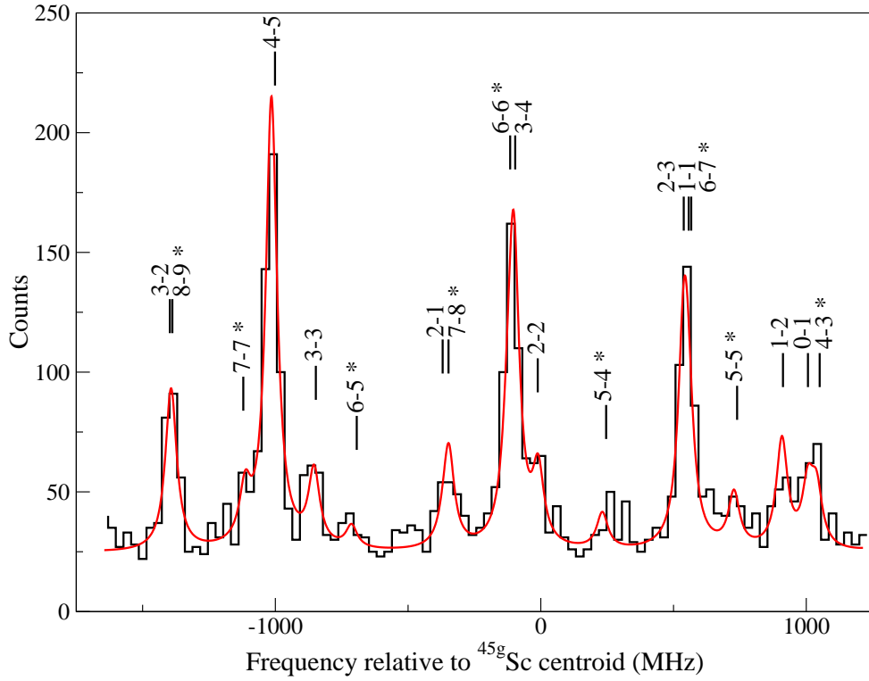
Figure 3. Example of a resonance fluorescence spectrum for ^{44g,m}\text{Sc} . The hyperfine F_1 \rightarrow F_u transitions are indicated, with isomeric components denoted with an asterisk (*). Other spectra (not shown) with overlapping scan regions were also taken and analyzed simultaneously.
