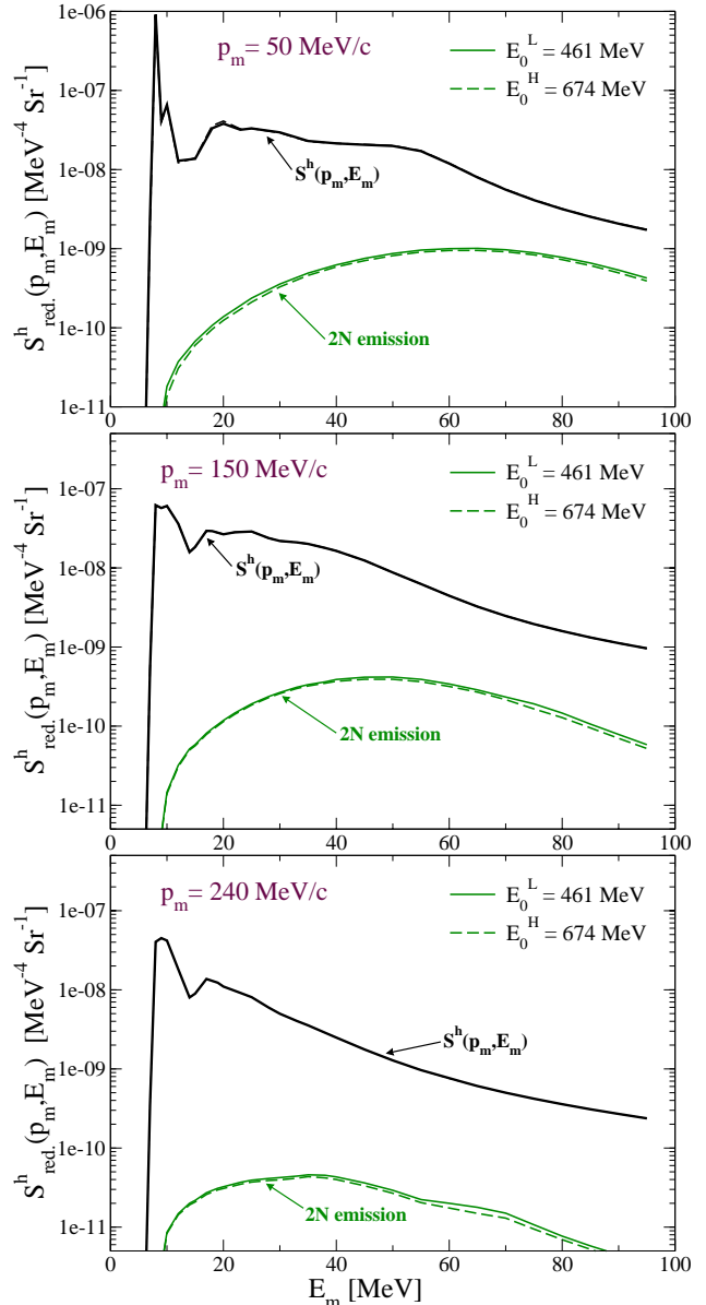
Fig. 2. Theoretical results for the rescattering contribution to the reduced spectral strength of 208 Pb for the kinematics of Ref. [21]. The full (dashed) lines refer to the kinematics with lower ( E_0^L ) and higher ( E_0^H ) energy beams. The thick lines show the input spectral function, S_p^h(p_m, E_m) .
