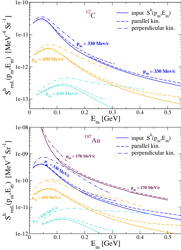
Fig. 3. Theoretical results for the reduced spectral strength in the correlated region obtained in parallel (dashed line) and perpendicular (dot-dashed line) kinematics. The full line shows the model spectral function, Eq. (2), employed in the calculations. The results are shown for ^{12}\text{C} (top) and ^{197}\text{Au} (bottom) targets.
