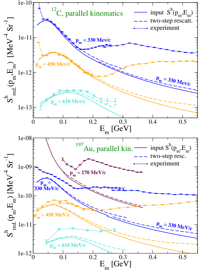
Fig. 4. Theoretical results for the total reduced spectral strength (dashed line) are compared to the experimental data in parallel kinematics. The full line shows the model spectral function, Eq. (2), employed in the calculations. The top (bottom) panel refer to a ^{12}\text{C} ( ^{197}\text{Au} ) target and the experimental data are from Ref.[20]. The values of p_m refer to the center of the experimental bins.
