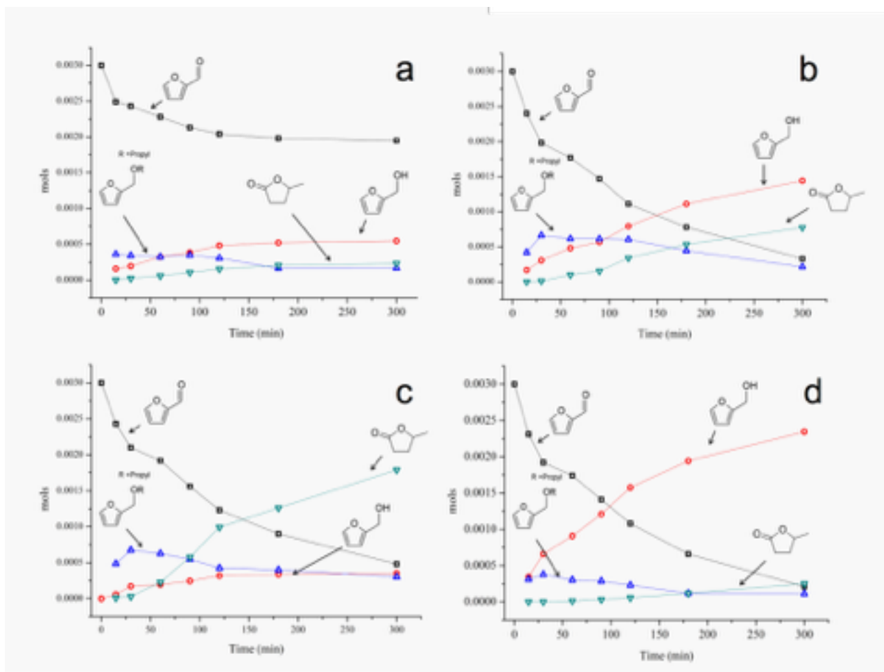
Figure 2. Product distribution for Ru/ZrO 2 (section a), AuRu/ZrO 2 (section b), AuRu/Y-ZrO 2 (section c) and AuRu/La-ZrO 2 (section d).
