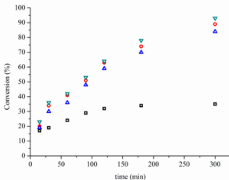
Figure 1. Reaction profile for monometallic Ru/ZrO 2 (black squares), and bimetallic AuRu/ZrO 2 (red circles), AuRu/Y-ZrO 2 (blue triangles) and AuRu/La-ZrO 2 (cyan triangles) catalysts.
