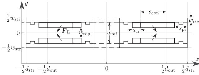
Figure 15. Cross sectional sketch of the demonstrator coil. The characterizing geometrical parameters of the mechanical structure are shown together with the forces.
