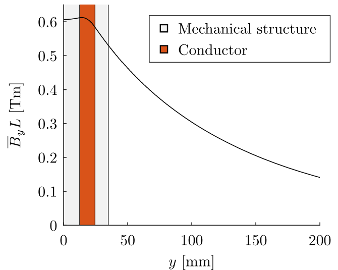
Figure 19. The bending strength as a function of y for the demonstrator coil.
