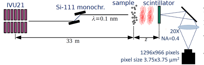
Figure 3: Schematic drawing of the HNFS setup installed at NCD-Sweet beamline at ALBA.
